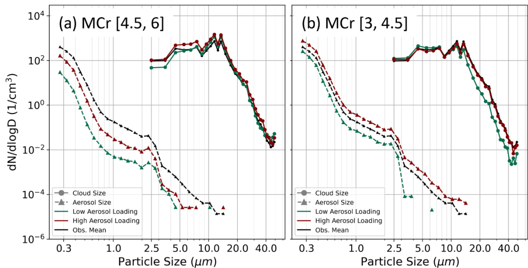
Figure 11: Size distribution of aerosols (triangles) and cloud droplets (circles). The black line represents the mean of all observations during the study period (not constrained by MCr intervals). Red and green lines follow the same conditions as in Figure 10. (a) Red and green lines limited to the MCr range [4.5, 6]; (b) Red and green lines limited to the MCr range [3, 4.5].
