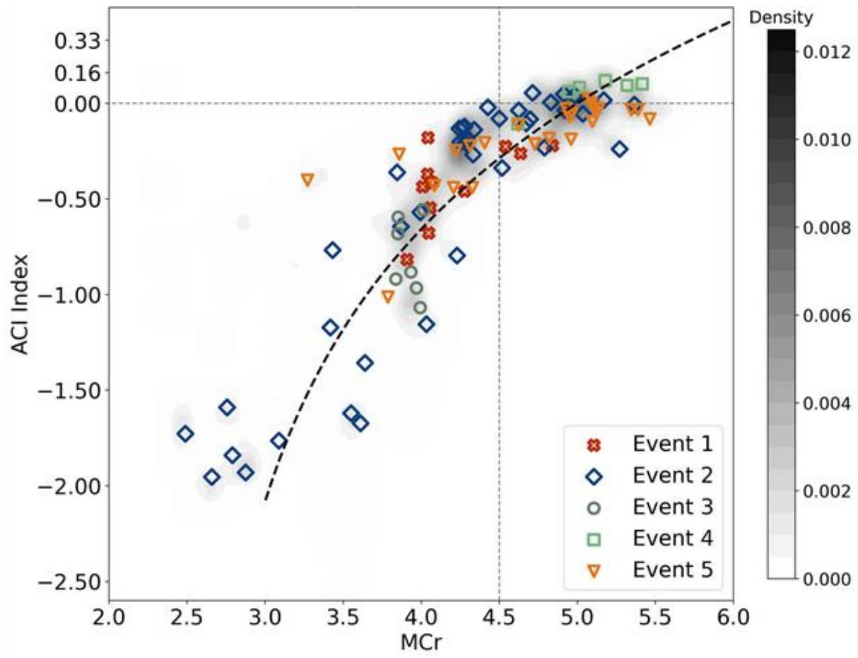
815 Figure 7: Scatter and density plots of the MCr-ACI index for the continuous cloud events. The density plot illustrates the overall distribution of all calculated results, while the scatter plot shows the distribution of individual cloud events using different colors and symbols (one point shown for every 30 calculations).
