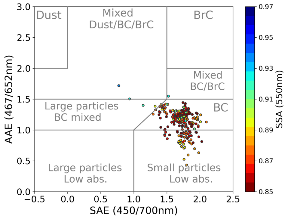
Figure 5: Classification of PM 10 aerosols at LABS from March 1 to March 12, 2024 (Classification method adapted from Schmeisser et al. (2017)), BC means black carbon type, BrC means brown carbon type.
