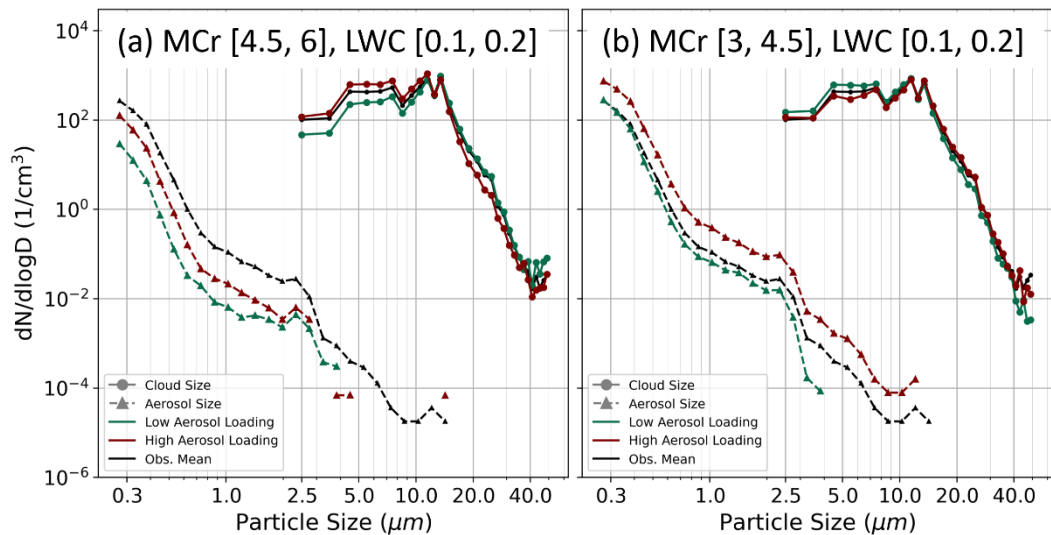
Figure 12: Same as Fig. 11, but all data are limited to the LWC range of 0.1-0.2 g m -3 , including the black line, which represents the mean of all observation data within this LWC range.
