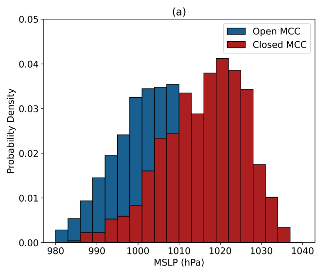
Figure S2: Probability density distribution of MSLP during open and closed MCC conditions.
