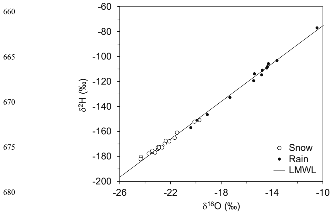
660 665 670 675 680 Figure A2 Isotopic composition of rain samples collected at the spring and snow samples collected at the spring or its vicinity (< 4 km). The local meteoric water line (LMWL) was derived from all precipitation samples that were collected during this study.
