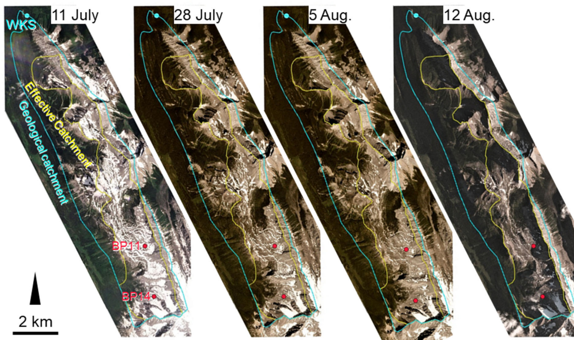
690 Figure A3 Satellite images of the potential recharge areas of the Watridge Karst Spring (WKS) on 11 July, 28 July, 5 August, and 12 August of 2020. The images show the tracer release locations (BP11 and BP14) the geological catchment, and the effective catchment (Figure 1a). Image source: Planet Team (2025).
