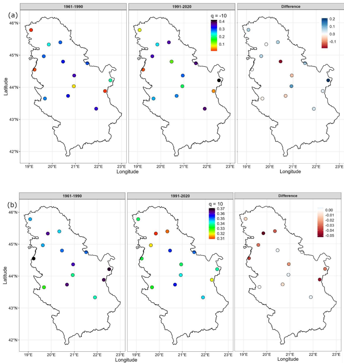
Figure 9: GWPEC for q = -10 (a) and q = 10 (b) for 14 stations in Serbia for two periods (1961-1990 and 1991-2020). The third panel illustrates the change between these periods, expressed as the difference in GWPC (1991-2020 minus 1961-1990), highlighting regions with increasing or decreasing complexity of small ( q=-10 ) and large ( q=10 ) precipitation fluctuations.
