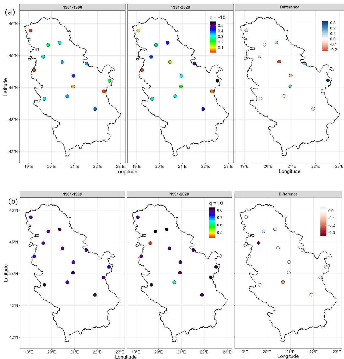
Figure 8: GWPE for q = -10 (a) and q = 10 (b) for 14 stations in Serbia for two periods (1961-1990 and 1991-2020). The third panel illustrates the change between these periods, expressed as the difference in GWPE (1991–2020 minus 1961–1990), highlighting regions with increasing or decreasing predictability of small ( q=-10 ) and large ( q=10 ) precipitation fluctuations.
