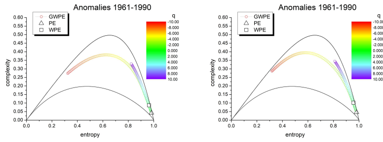
Figure 4: GWPE curves representing entropy/complexity as a function of the magnification parameter q for 14 meteorological stations in Serbia during the first sub-period (1961–1990). The parameter q highlights small fluctuations for q < 0 and large fluctuations for q > 0 , enabling scale-sensitive analysis of precipitation dynamics. Solid lines indicate theoretical bounds for a segment size of w = 6 days, as defined by Martin et al. (2006).
