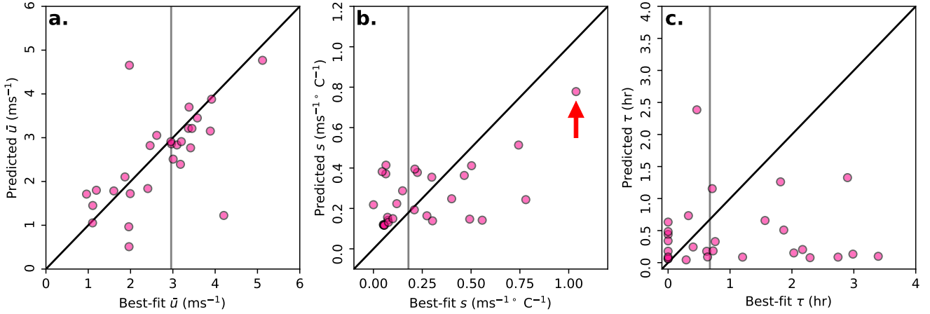
Figure 5. The value of model parameters predicted by Eqs. 10–12 are plotted against their observed best-fit values from all 28 stations. The grey vertical line shows the median value of each model parameter across all stations. a) The predictor \sqrt{\frac{|\bar{T}|}{\varsigma_{10}}} was found to have a strong relationship with \bar{u} , with an R^2 of 0.9 ( p < 0.001 ). b) For s , the predictor 1/\sqrt{|\bar{T}|/\varsigma_{10}} was found to have a significant relationship with an R^2 of 0.57 ( p < 0.001 ), but upon removal of the data point marked with red arrow, the relationship became insignificant. c) None of the predictors discussed in sect. 3.1.3 showed a significant relation with \tau . Due to the lack of predictability of s and \tau , we used the corresponding median values to estimate them for ungauged glaciers, which does not capture variability of these quantities between glaciers.
