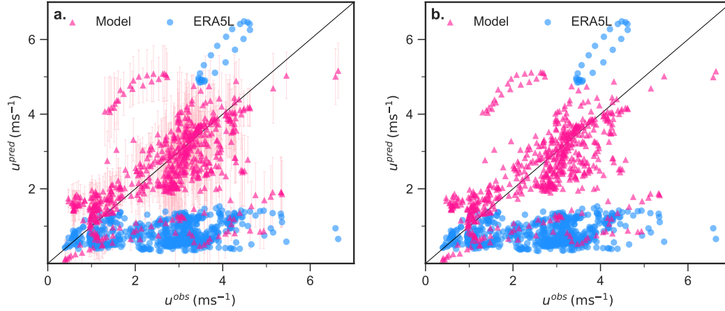
Figure 6. The mean summertime diurnal wind speed predicted using Eqs. 1, 7–9–10–12 (red solid triangle) were compared with corresponding observation. The corresponding comparison for ERA5L wind speed are also shown (blue solid circles). (b) The inset shows the distribution result of RMSEs for LOOCV (main text, section 4.2.2): For each of the 28 left-out stations, the predicted u is compared to the corresponding observed values. The ERA5L wind speeds for both our model (the left-out stations are also shown as light pink histogram) and ERA5 (shown as light blue histogram solid circles).
