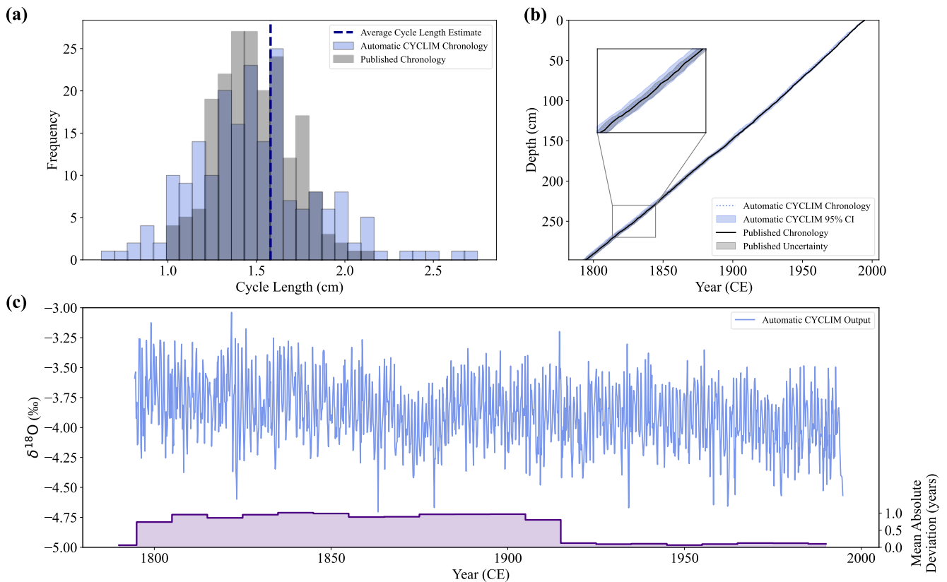
Figure 8: The CYCLIM age model and final output for the Houtman Abrolhos Coral record. (a) Distribution of annual cycle lengths for the automatic (light blue) and published (grey) chronologies. The vertical dashed line shows the average cycle length hyperparameter estimate. (b) The automatic CYCLIM age model (light blue) shown with the published age model (black) presented in Kuhnert et al. (1999), both with their respective uncertainties. (c) The automatic CYCLIM output record (blue) and chronological mismatch with the published record (purple). Mismatches are averaged by decade.
