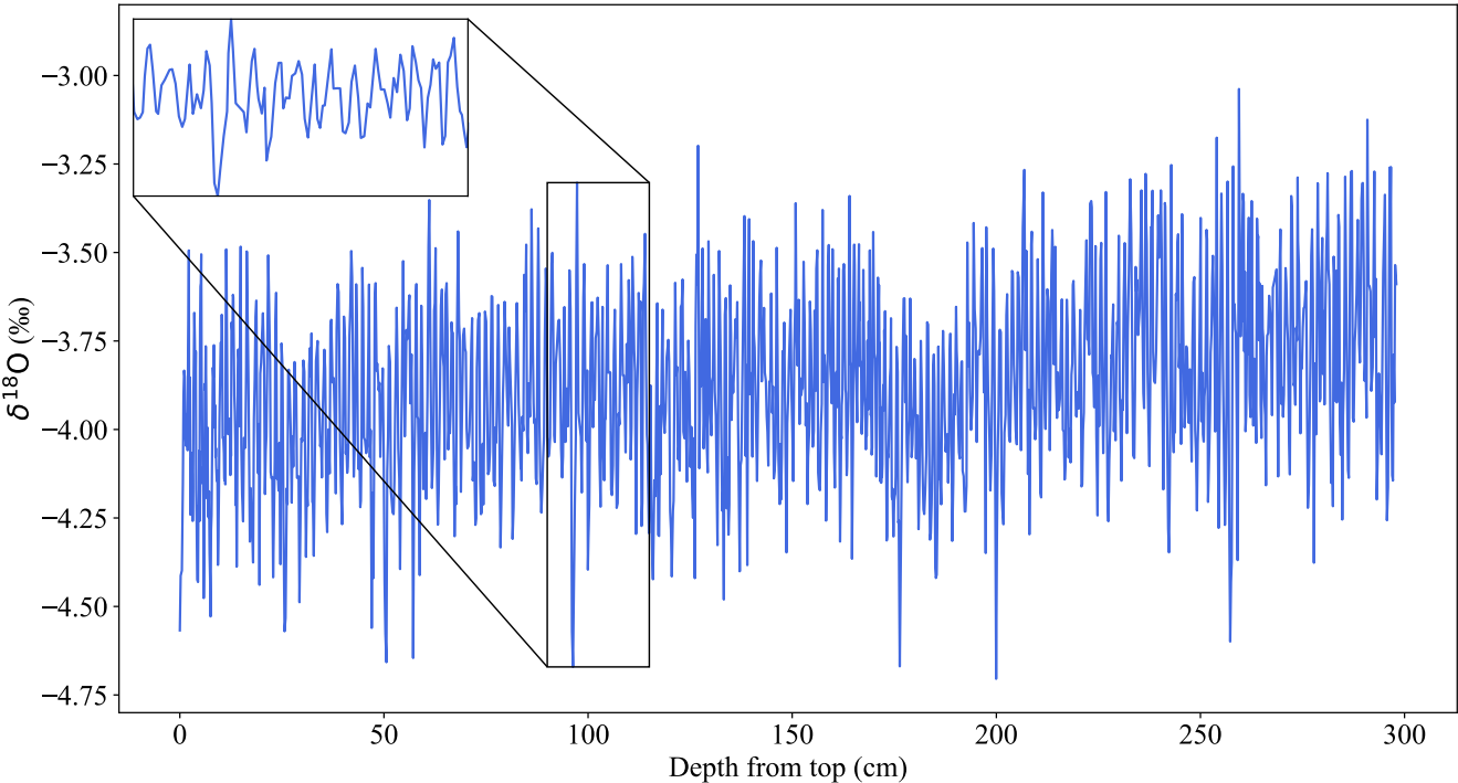
Figure 4: The depth-proxy Houtman Abrolhos Coral \delta^{18}\text{O} record (blue; Kuhnert et al. (1999)). The inset shows an example interval of annual scale cyclicality.
