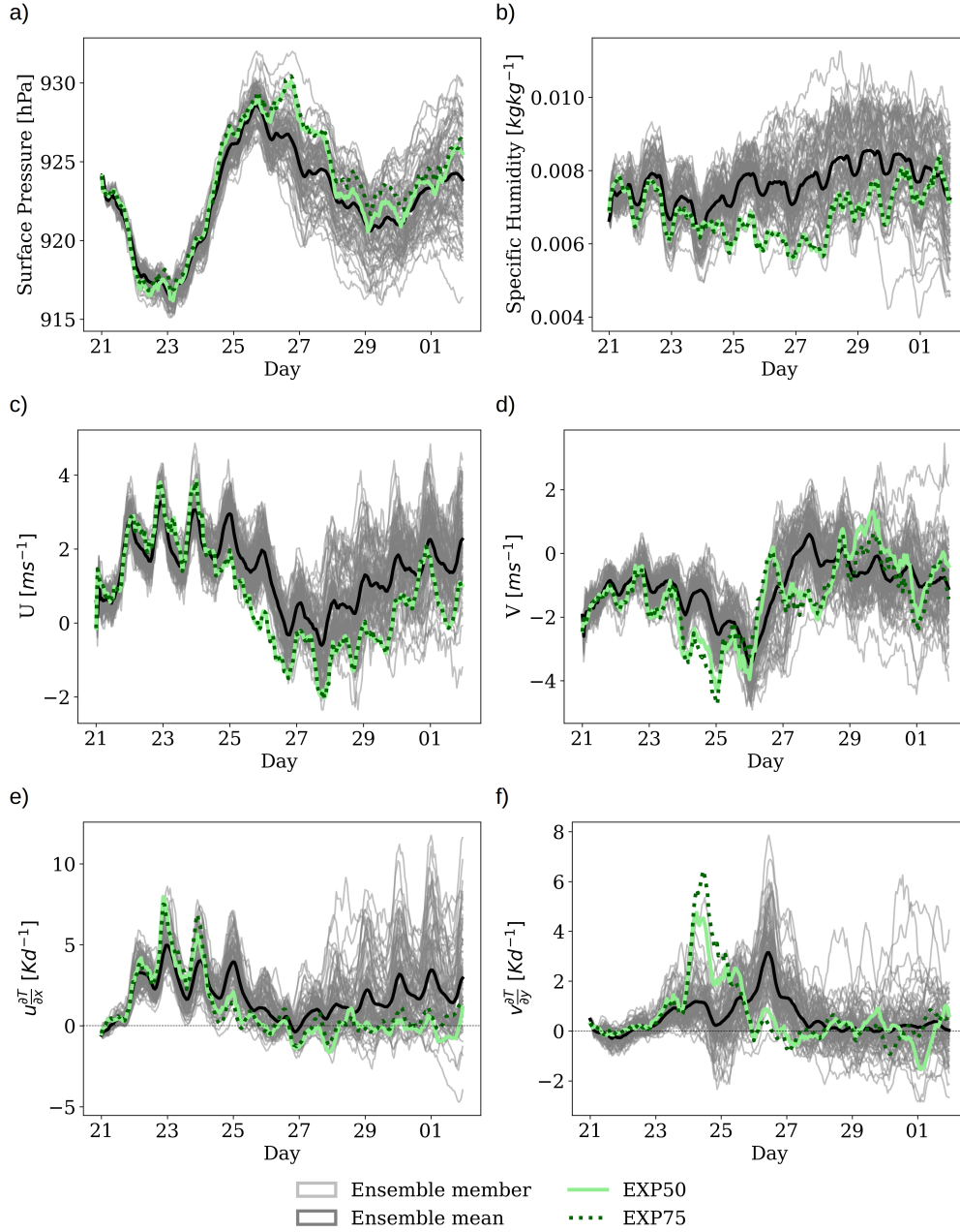
Figure 5. Time series of (a) surface pressure, (b) near-surface specific humidity, (c) U-component of wind, (d) V-component of wind, (e) and (f) temperature advection for each component at 1000 hPa . Data from the optimized trajectory are shown alongside the individual ensemble members (in grey) and the ensemble mean (thick black line).
