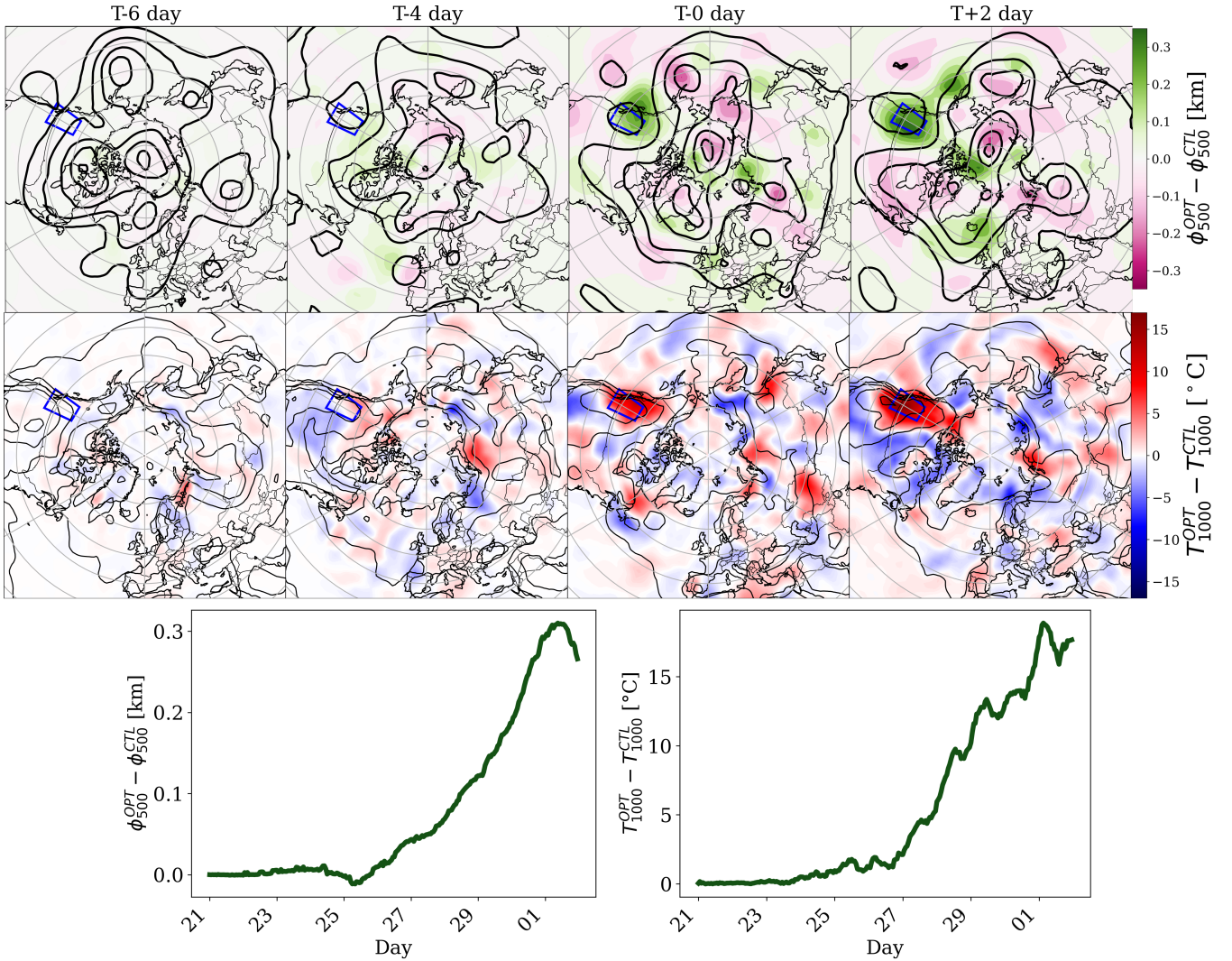
Figure 2. Top row: Evolution of the difference in 500-hPa geopotential height ( \Delta Z , in km) between the optimized simulation and the control run for EXP75. Black contours (optimized run) outline the amplified Rossby wave pattern, with deeper troughs and higher ridges compared to the control. Middle row: The difference in 1000-hPa temperature ( ^{\circ}\text{C} ) between the optimized and control simulations. Bottom row: The difference between the 500-hPa geopotential height and 1000-hPa temperature averaged over the target domain.
