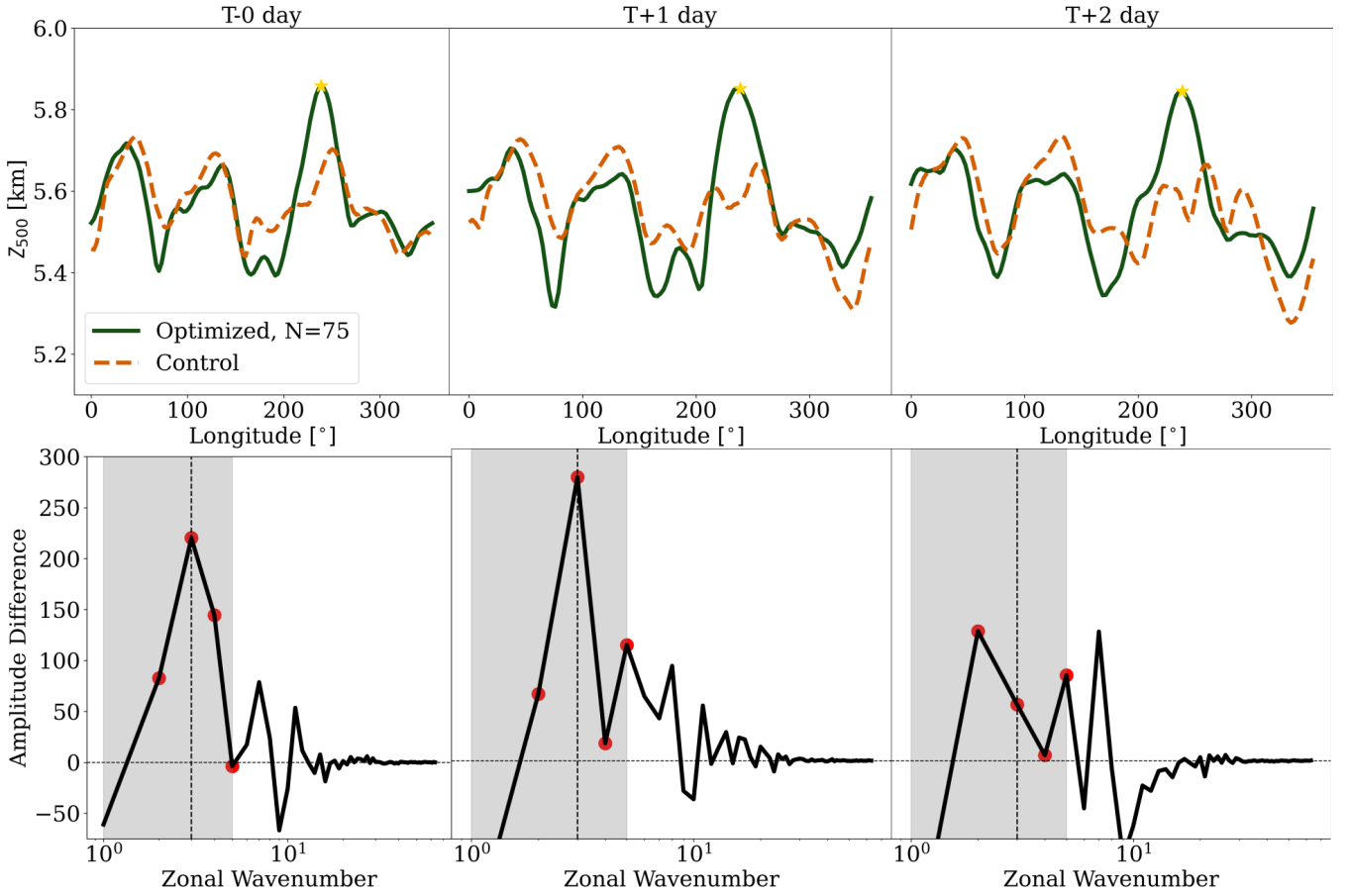
Figure 3. Top row: cross section of 500-hPa geopotential along a fixed latitude for EXP75. Bottom row: the amplitude difference of the Fourier spectrum, including wavenumbers 1–5 highlighted in greygray . Red dots highlight wavenumbers 2–5.
