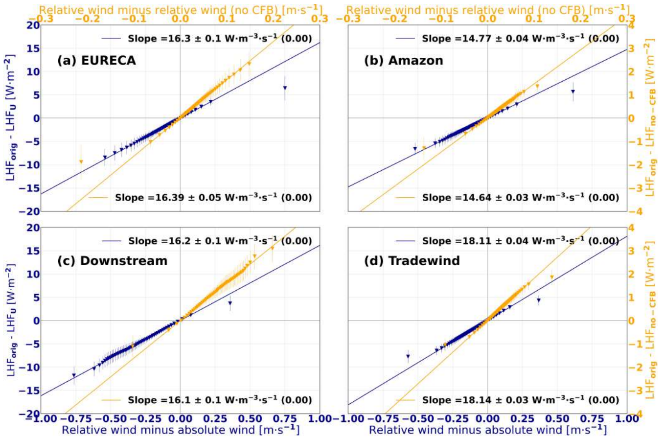
Figure 6. LHF sensitivity to surface currents for (a) EURECA, (b) Amazon, (c) Downstream, and (d) Tradewind. In all panels, blue markers represent the difference between \text{LHF}_U and \text{LHF}_{\text{orig}} as a function of the difference between the norm of the first vertical level wind velocity and the relative wind velocity field. Orange markers indicate the difference between \text{LHF}_{\text{orig}} and \text{LHF}_{\text{no-CFB}} as a function of the difference between the norms of relative winds, with and without the CFB effect. The methodology used to derive these LHF datasets is detailed in the main text. The x-axis variable is divided into intervals containing an equal number of values, using a 2% percentile separation. Vertical error bars indicate the standard deviation relative to the mean for each interval, while straight lines denote the least-squares regression fits. The regression slope \pm standard error (p-value) is displayed in each panel's legend.
