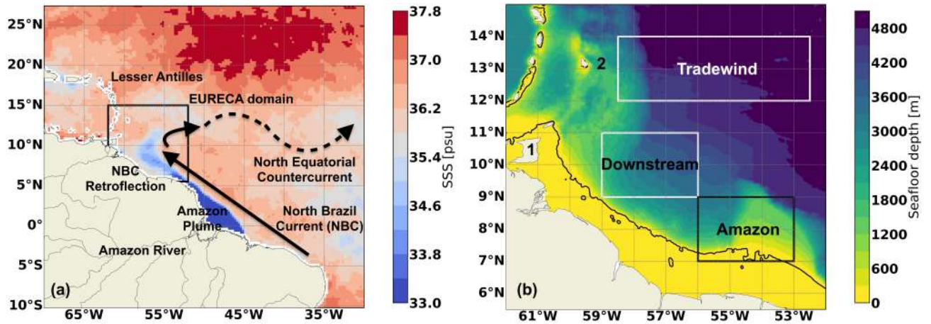
Figure 2. (a) Major dynamical features of the western equatorial Atlantic (arrows) overlaid on the averaged sea-surface salinity (SSS) field from February 17 th –19 th , 2020. The SSS field is derived from the SMAP-SSS Level 3, version 4.0, 8-day running-mean gridded product (Boutin et al., 2021). The black box delineates the EURECA region, which corresponds to the simulation domain used in this study. (b) Seafloor depth from the simulation used in this study which is derived from the GEBCO 2020 global bathymetric dataset (Conejero et al., 2024). The three boxes delineate the three sub-regions within the EURECA domain assessed in this paper: Amazon, Downstream and Tradewind and the black contour represents the 100 m isobath. Numbers 1 and 2 mark the locations of Trinidad and Tobago and a region near Barbados, respectively. These geographical references, along with the Lesser Antilles marked in panel (a), are used throughout the main text. Detailed descriptions of the simulation used in this study and of the sub-regions follow in Sections 2 and 3 respectively.
