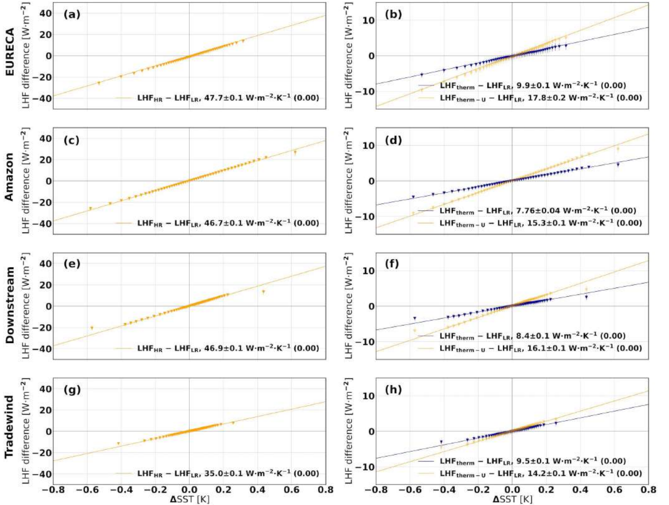
Figure 5. LHF sensitivity to \Delta SST (see Eq. 3) across different regions. Each row corresponds to a specific domain: the EURECA region (first row), the Amazon sub-region (second row), the Downstream sub-region (third row), and the Tradewind sub-region (fourth row). Panels (a), (c), (e), and (g) display the difference between LHF_{HR} and LHF_{LR} as a function of \Delta SST . Panels (b), (d), (f), and (h) show the differences between LHF_{therm} and LHF_{LR} , and between LHF_{therm-U} and LHF_{LR} , as a function of \Delta SST (blue and orange, respectively). The methodology used to compute these LHF datasets is detailed in the main text. The SST anomaly values are binned into 2% percentile intervals. Vertical error bars indicate the standard deviation from the mean in each interval, while straight lines represent the least-squares regression fits. The regression slope \pm standard error (p-value) is reported at the bottom of each panel.
