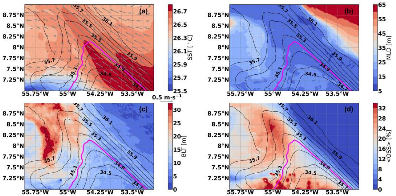
Figure 9. February 2020 average of (a) SST (shading) and surface currents (arrows), (b) mixed layer depth (MLD, shading), (c) barrier layer thickness (BLT, shading) and (d) OSS index integrated down to the base of the mixed layer ( \langle OSS \rangle , shading). In all panels black contours denote the February 2020 averaged SSS and the magenta contour the mean February 2020 position of the edge of the Amazon plume (35 psu isoline).
