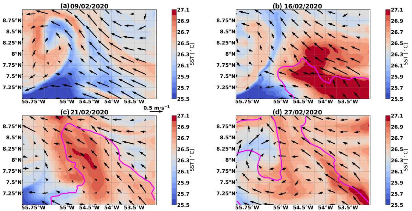
Figure 8. Daily snapshots of SST (shading) overlaid with surface currents (arrows) and the 35 psu isoline which we use to delimit the Amazon plume (magenta) for the (a) 9 th , (b) 16 th , (c) 21 th and (d) 27 th of February 2020.
