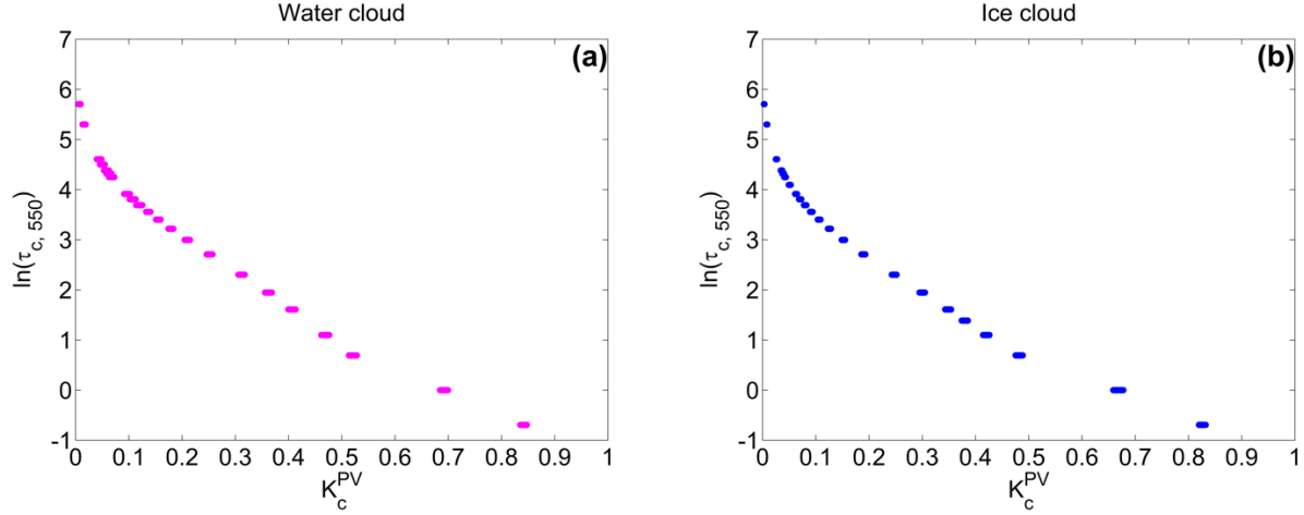
Figure 3. Scatterplot between K_c^{PV} on horizontal axis and \ln(\tau_{c,550}) on vertical axis by varying all parameters except AOD_{550}=0.074 , \rho_g=0.2 and ws=5 \text{ m s}^{-1} . (a) for water cloud and (b) for ice cloud.
