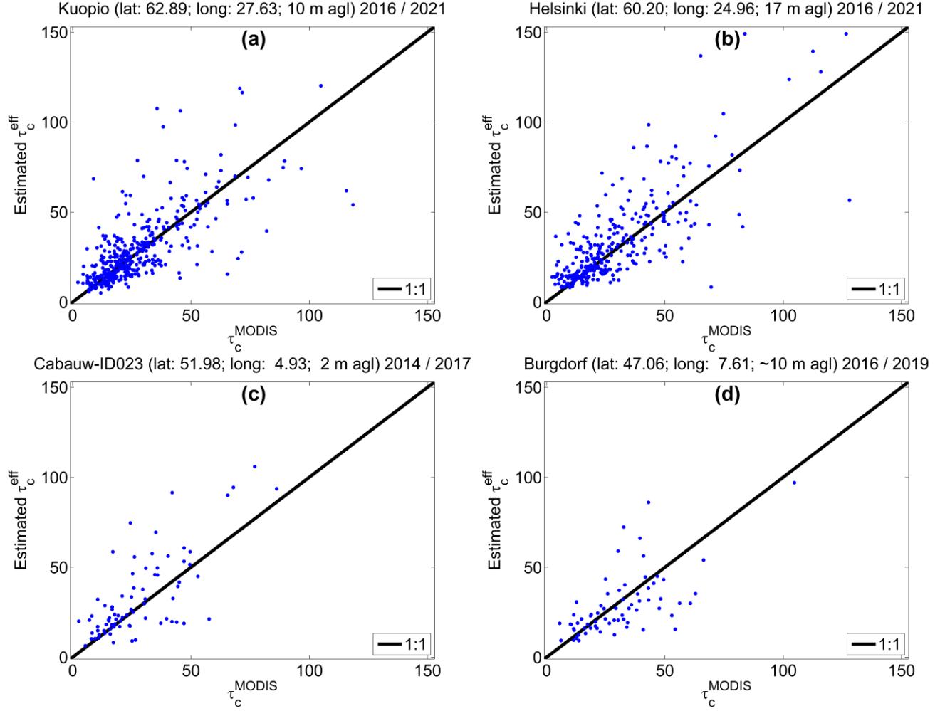
Figure 9. Scatterplots between instantaneous \tau_c^{MODIS} retrievals (horizontal axis) and 15-min averages of \tau_c^{eff} estimates (vertical axis) for water clouds at (a) Kuopio, (b) Helsinki, (c) Cabauw–ID023 and (d) Burgdorf when using CF^{MODIS} for selecting overcast sky conditions.
