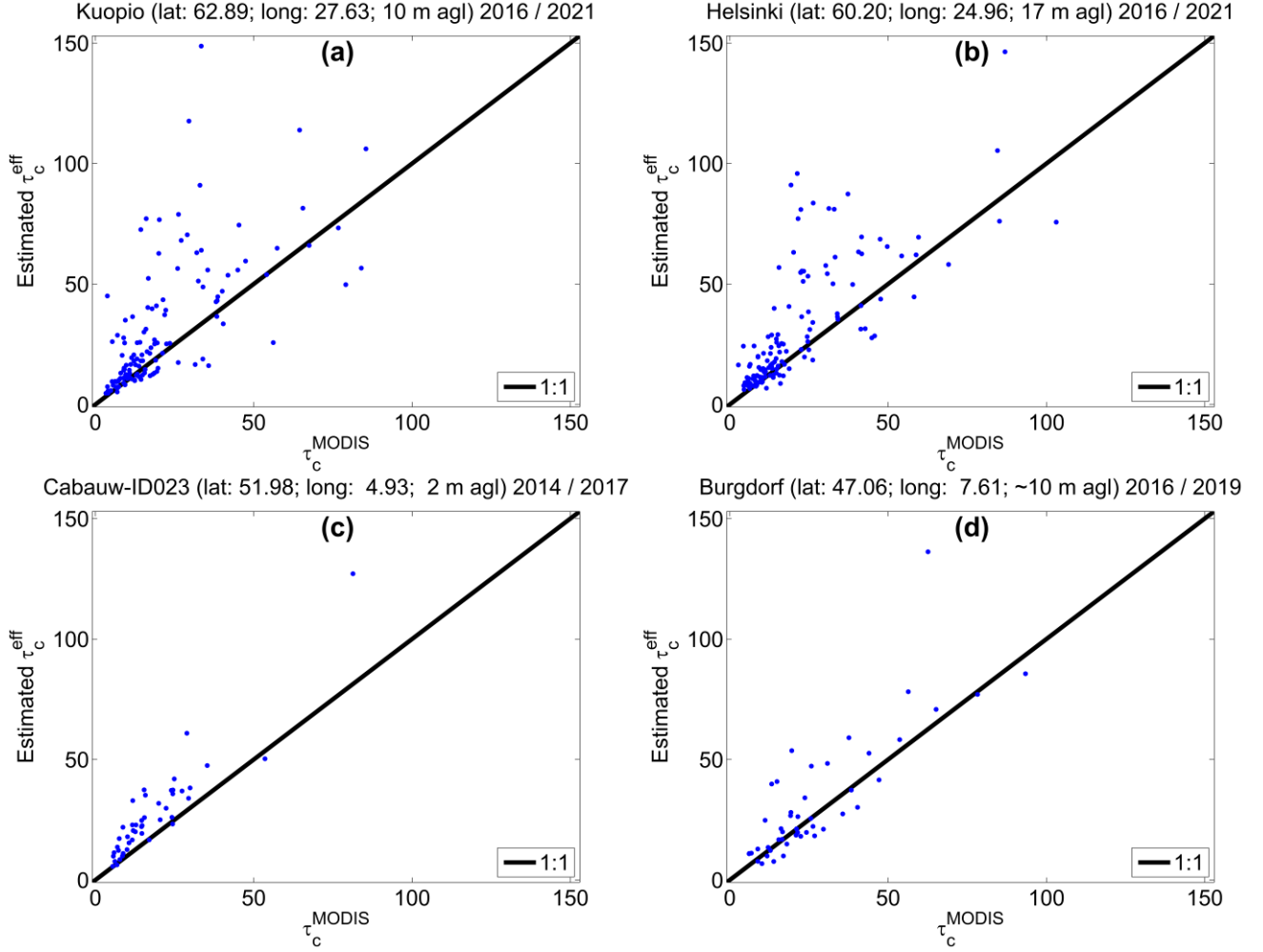
Figure 10. Scatterplots between instantaneous \tau_c^{MODIS} retrievals (horizontal axis) and 15-min averages of \tau_c^{eff} estimates (vertical axis) for ice clouds at (a) Kuopio, (b) Helsinki, (c) Cabauw–ID023 and (d) Burgdorf when using CF^{MODIS} for selecting overcast sky conditions.
