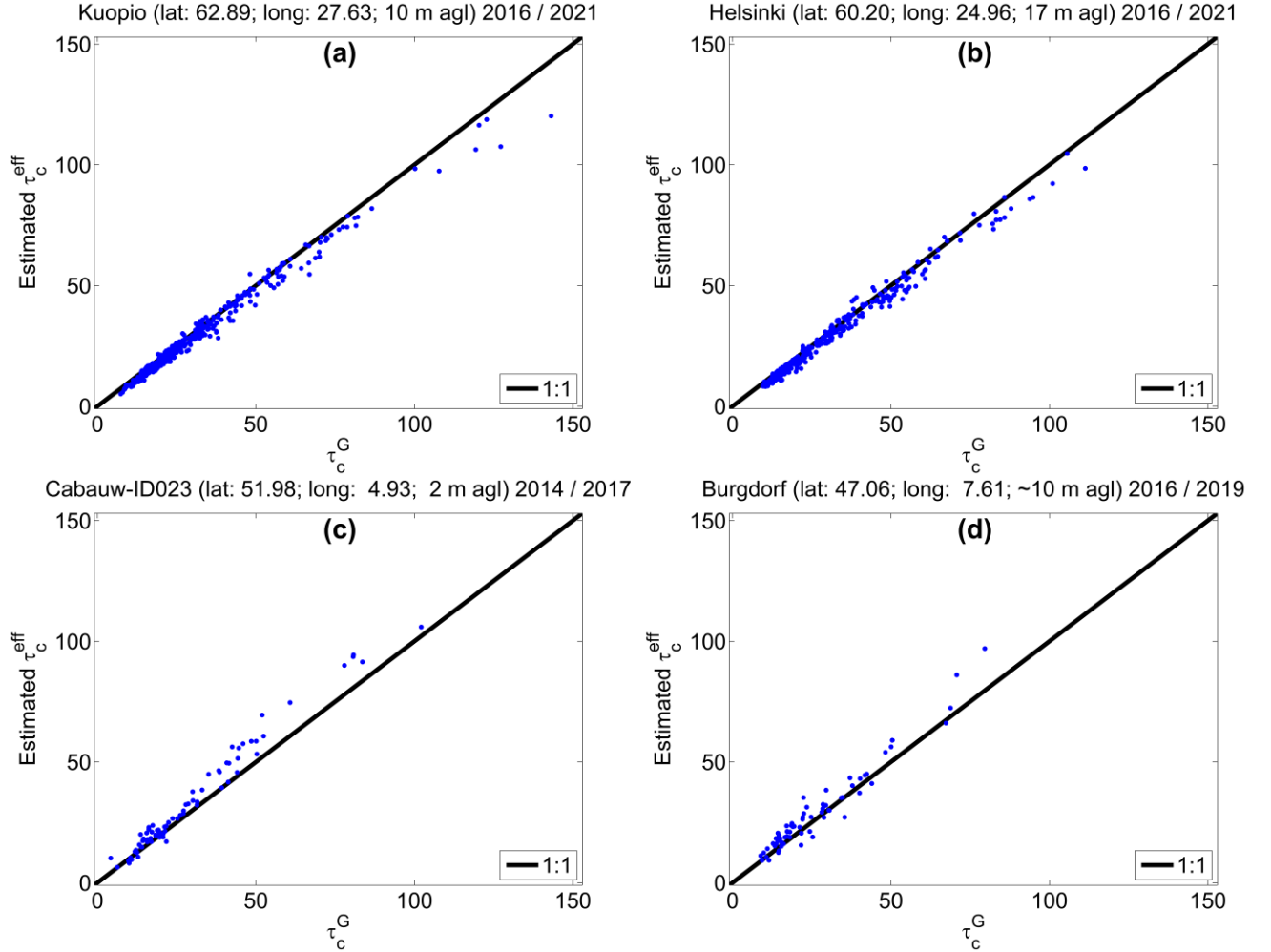
Figure 8. Scatterplots of 15-min averages between \tau_c^G retrievals (horizontal axis) and \tau_c^{eff} estimates (vertical axis) for water clouds at (a) Kuopio, (b) Helsinki, (c) Cabauw–ID023 and (d) Burgdorf when using CF^{MODIS} for selecting overcast sky conditions.
