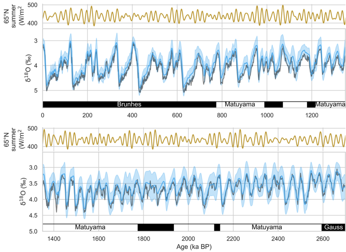
Figure S1. Comparison of BIGSTACK LR04 with the LR04 stack. Blue line with shading shows BIGSTACK LR04 and its 95% confidence limits. Black line is the LR04 stack. Yellow line is the Northern Hemisphere insolation at 65°N. Geomagnetic polarity chrons are marked at the top and bottom of the figure, with the four subchrons within Matuyama being, from young to old, Jaramillo, Cobb Mountain, Olduvai, and Réunion (Feni).
