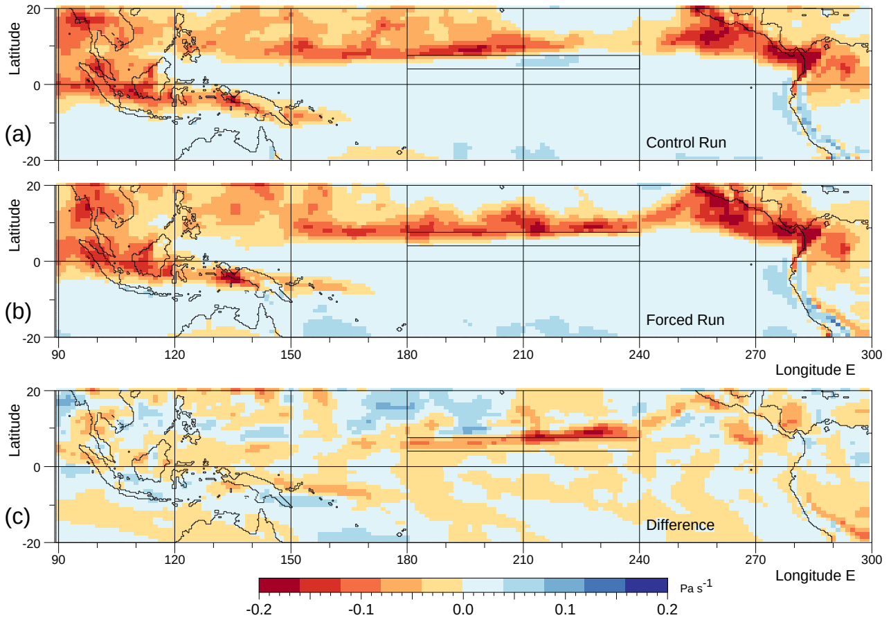
Figure 1. Average rate of change of pressure following particles ( dP/dt ), also known as Omega, crossing the 525 hPa pressure surface in September of year 5 for (a) the control run and (b) the forced run and (c) the difference. The forcing, described in the text, starts at the beginning of August in year 5 and is non-zero within the marked rectangular region in the central Pacific. Negative (red) values correspond to convection.
