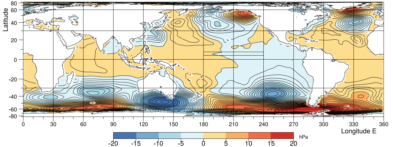
Figure 3. Global change in sea level pressure, due to the forcing, averaged over September of year 5. Contour interval 1 hPa.
