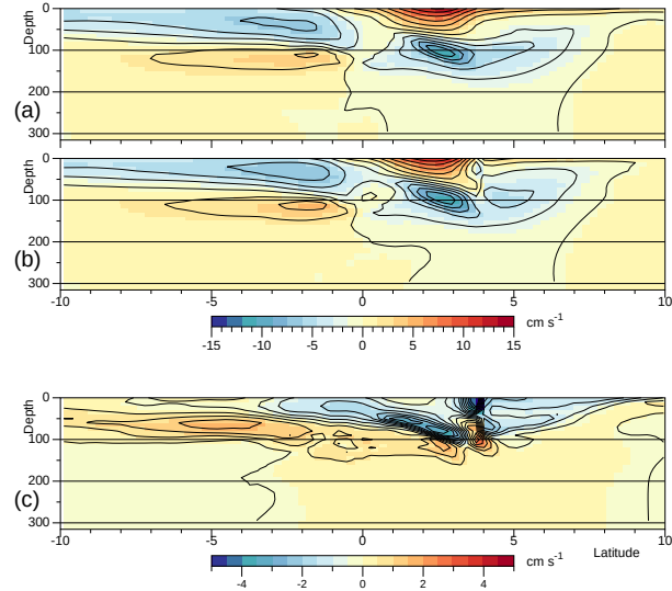
Figure A4. Northward component of velocity, averaged between 210°-E and 240°-E during September of year 5 for (a) the control run, (b) the forced run, (c) the difference.
