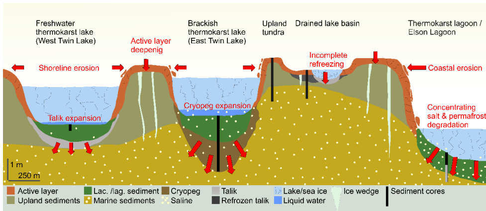
570 Figure 6: Conceptual illustration of physical properties and dynamics currently affecting the Barrow Peninsula with potential for future acceleration. The sediments are present in a variety of thermal states, seasonally frozen (active layer), perennially frozen (upland and marine sediments), unfrozen (talik, lacustrine sediments, partly DLB in the drained lake basin), unfrozen cryotic (cryopeg and lacustrine/lagoon sediments) and refrozen (DLB drained lake basin). Model illustrated at approximate scale.
