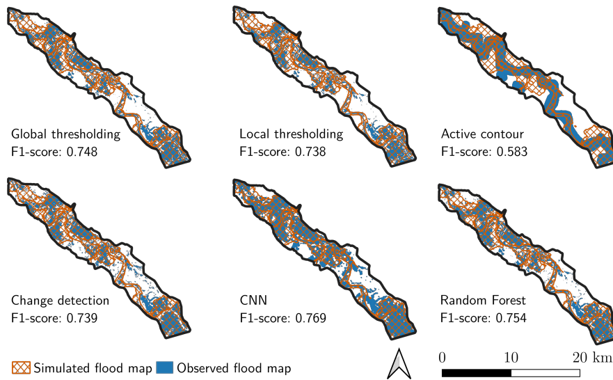
Figure 14. Comparison of the simulated flood maps ( green orange ) with the generated flood maps (blue) for 2 February 2021.
