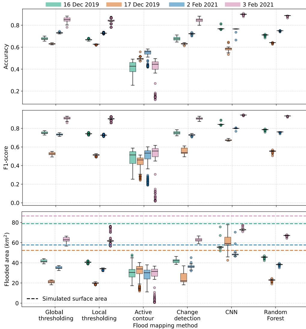
Figure 9. Accuracy and F1-score and flooded area for the generated flood maps for four satellite images and various six flood mapping methods compared against their respective simulated flood maps for four satellite images.
