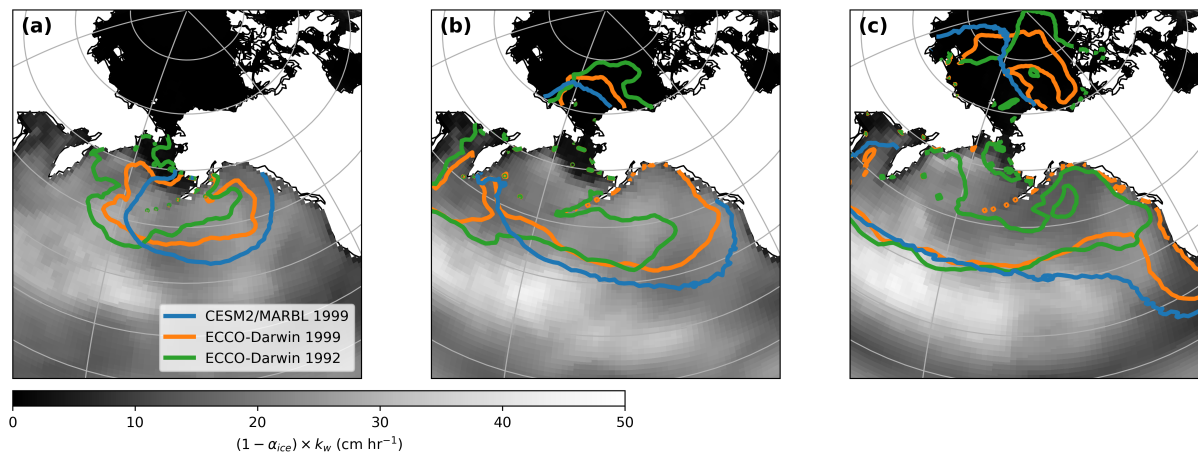
Figure 2. Three different plume outlines overlaid on the k parameter in greyscale from OceanSODA(Gregor and Gruber, 2021). State is shown a) 12 b) 36 and c) 72 months after alkalinity release near Alaska.
