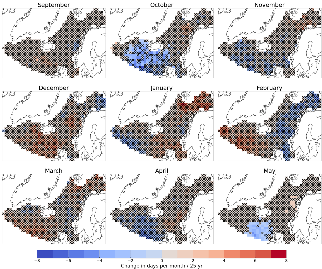
Figure C1. Trends for each month calculated using the Theil-Sen estimator. Stippled points are insignificant by not satisfying a false discovery rate of 0.2.
