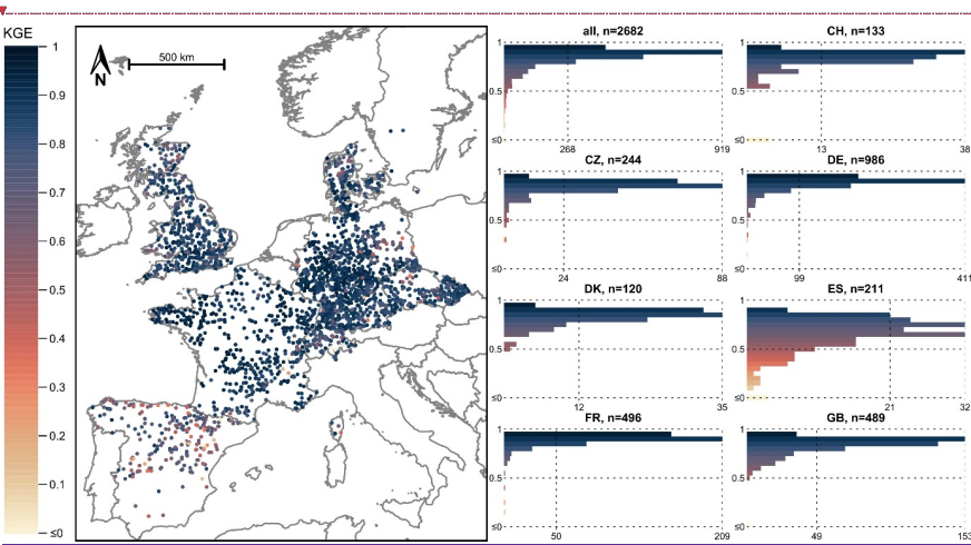
Figure 4: Model performance (Kling-Gupta efficiency, KGE) achieved for the 20-year period between October 1995 and September 2015 when the E-OBS data obtained from EStreams were used for model calibration (scenario II). Note that the lower limit of the colour scale was cut at zero. Lower performances were plotted last to improve their visibility.
