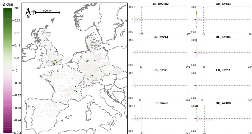
Figure A67: Difference in model performance when all meteorological input data were obtained from E-OBS (i.e., EStreams, scenario II) and when the E_{pot} data from E-OBS were replaced with those from CAMELS (scenario IV). Positive values and green colours indicate higher model performances with the E_{pot} data from E-OBS, negative values and pink colours indicate higher model performances with the E_{pot} data from CAMELS. Note that the colour scale was cut at a difference in KGE of \pm 0.3 . The catchments with the largest differences in model performance were plotted last to increase their visibility.
