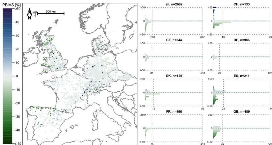
Figure 5: PBIAS (relative deviation of the simulated streamflow from the observed streamflow) for the 20-year period between October 1995 and September 2015 when the E-OBS data obtained from EStreams were used for model calibration (scenario II). Note that the limits of the colour scale were cut at \pm 50\% . Largest deviations were plotted last to improve their visibility.
