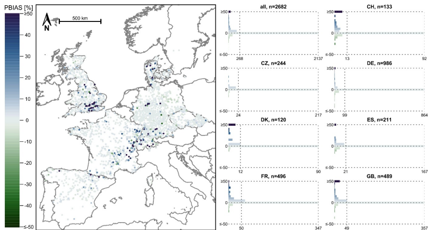
Figure A4: PBIAS (relative deviation of the simulated streamflow from the observed streamflow) for the 20-year period between October 1995 and September 2015 when the E-OBS data obtained from EStreams were used for model calibration (scenario II). Note that the limits of the colour scale were cut at \pm 50\% . Largest deviations were plotted last to improve their visibility.
