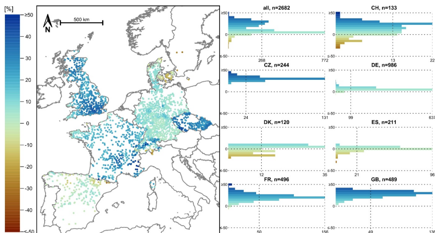
Figure 2: Relative difference in the mean annual E_{pot} (for a 20-year period: 1995-2015) obtained from EStreams and calculated from the E-OBS data compared to the mean annual E_{pot} calculated from the different CAMELS datasets. Negative values and brown colours indicate a lower E_{pot} in E-OBS than in the CAMELS datasets, positive values and blue colours a higher E_{pot} . On the map, the catchments with the largest deviations were plotted last to increase their visibility.
