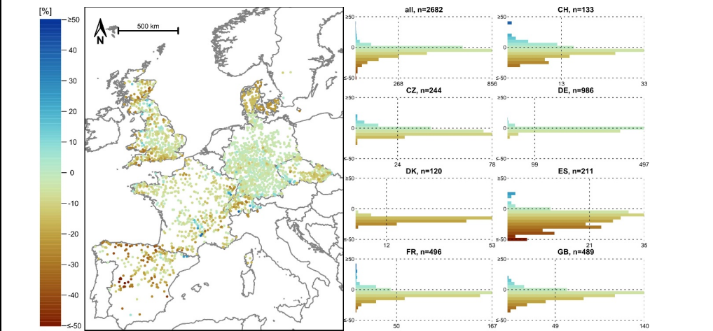
Figure 1: Relative difference in the mean annual precipitation (for a 20-year period: 1995-2015) between the E-OBS data obtained from EStreams and the different CAMELS datasets. Negative values and brown colours indicate less precipitation in E-OBS than in CAMELS, positive values and blue colours more precipitation in E-OBS. On the map, the catchments with the largest deviations were plotted last to increase their visibility. Note that there is no separate histogram for the three catchments in Sweden and that the number of catchments per histogram differ. This is illustrated by the vertical lines indicating 10 % (rounded) of the number of catchments per histogram. The colour scale was cut at \pm 50 %. The scale bar refers to the map center. The base map was obtained from Natural Earth (naturalearthdata.com). The colour palette used in this and all other maps are scientific colour palettes from Crameri (2023).
