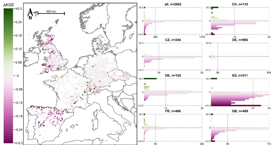
Figure A5: Difference in model performance when all meteorological input data were obtained from E-OBS (i.e., EStreams, scenario II) and when the precipitation data from E-OBS were replaced with those from CAMELS (scenario III). Positive values and green colours indicate higher model performances with the precipitation data from E-OBS, negative values and pink colours indicate higher model performances with the precipitation data from CAMELS. Note that the colour scale was cut at a difference in KGE of \pm 0.3 . The catchments with the largest differences in model performance were plotted last to increase their visibility.
