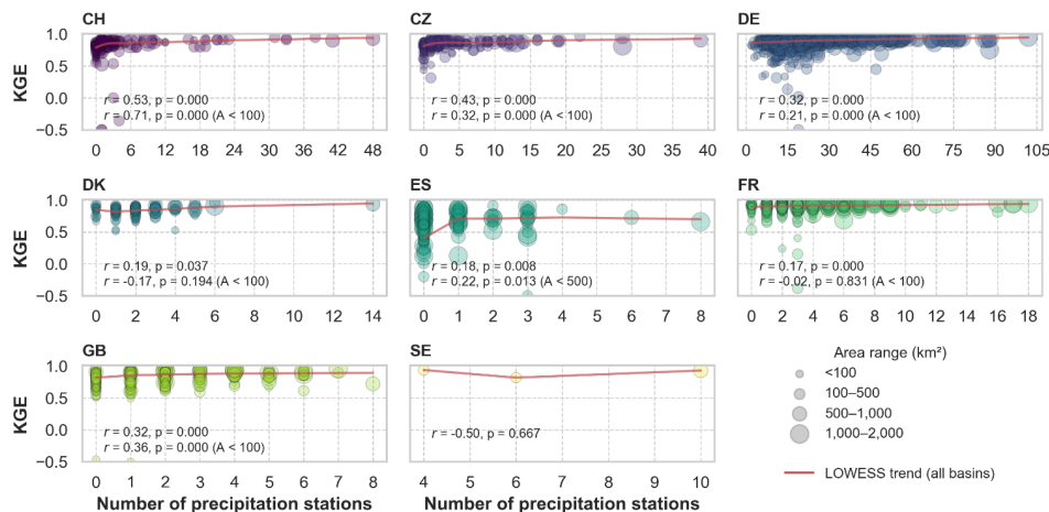
Figure 6: Scatterplots showing the model performance (Kling-Gupta efficiency, KGE) for scenario II (y-axes) versus the number of E-OBS precipitation stations in and around each catchment, per country. Each circle represents one catchment, the size is based on catchment area. Each subplot contains the Spearman rank correlation (r) and corresponding p-value, and the lowest trend line. The r and the p-value are computed for all catchments per country and also for the ones with an area below 100 km² (500 km² for Spain). Note that the y-axes were cut at -0.5, in accordance to Fig. 4, and the x-axes differ for the different subplots.
