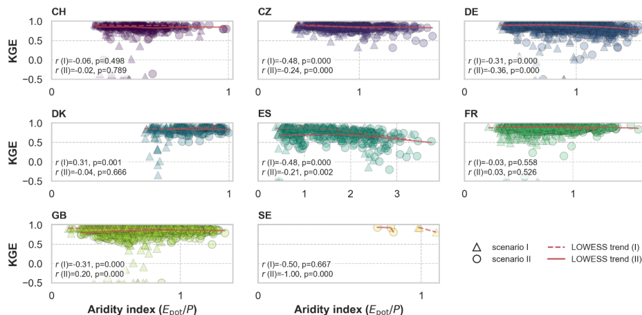
Figure 7: Scatterplots showing the model performance (Kling-Gupta efficiency, KGE) for scenario I and II (y-axes) versus the aridity indices derived from the corresponding forcing data (CAMELS for scenario I, E-OBS from EStreams for scenario II), per country. Each subplot contains the Spearman rank correlation ( r ) and corresponding p -value, and the lowess trend line. Note that the y-axes were cut at -0.5, in accordance to Fig. 4. Note that the x-axes differ for the different subplots.
