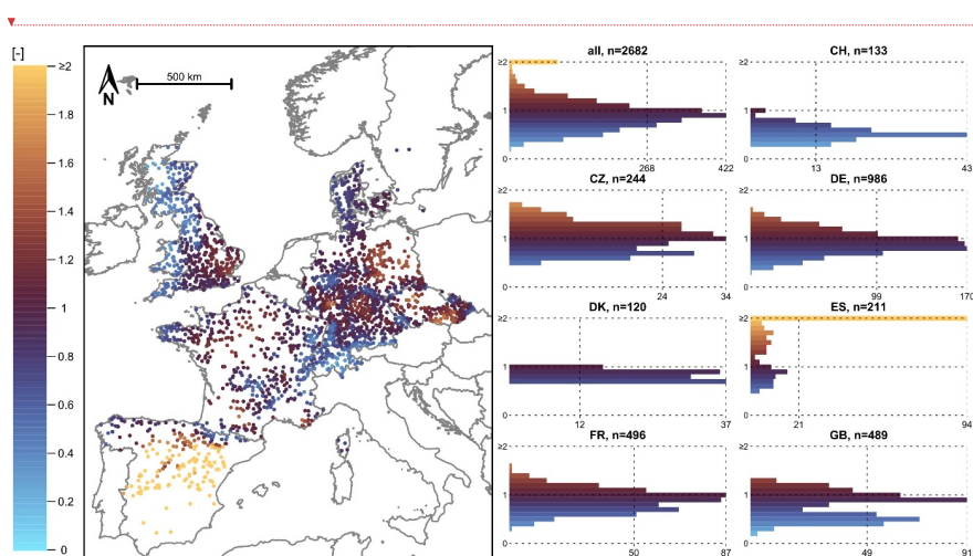
Figure A2: Aridity index ( E_{pot}/P ) calculated from the E-OBS data obtained from EStreams (for a 20-year period: 1995-2015). Note that the colour scale was cut at a value of two.
