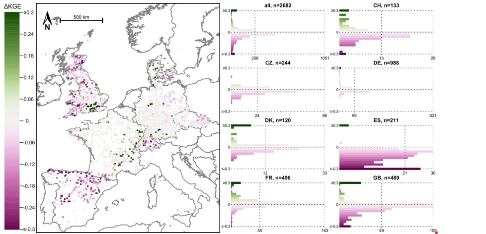
Figure 5: Difference in model performance (Kling-Gupta efficiency, KGE) between scenario II and scenario I. Positive values and green colours indicate higher performances when the E-OBS data obtained from EStreams were used, negative values and pink colours indicate higher performances when the CAMELS data were used. For the model performances, see Figs. 4 and A4. The catchments with the largest differences (in absolute terms) were plotted last to improve their visibility. Note that the colour scale was cut at \pm 0.3 .
