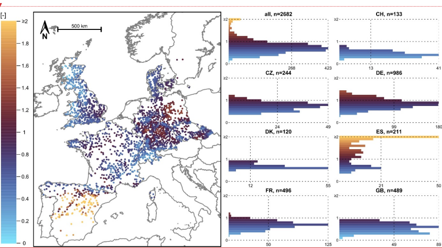
Figure A1: Aridity index ( E_{pot}/P ) calculated from the CAMELS data (for a 20-year period: 1995-2015). Note that the colour scale was cut at a value of two .
