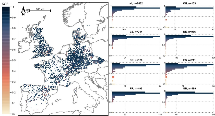
Figure A34: Model performance (Kling-Gupta efficiency, KGE) achieved for the 20-year period between October 1995 and September 2015 when the input data from the CAMELS datasets were used for model calibration (scenario I). Note that the lower limit of the colour scale was cut at zero. Lower performances were plotted last to improve their visibility.
