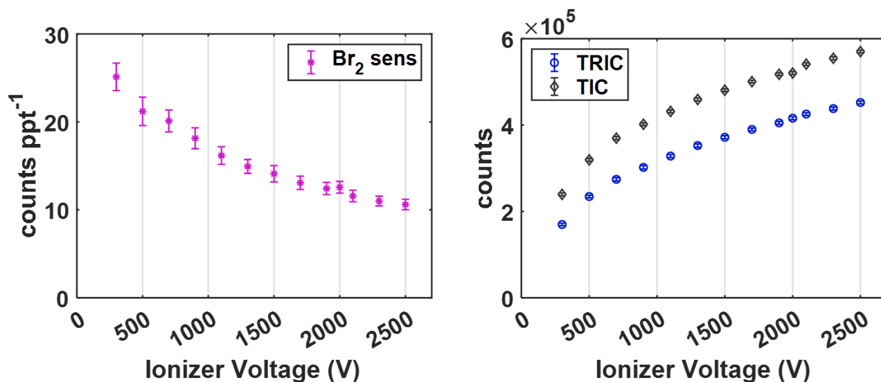
Figure 2. (left) Br 2 average sensitivity (counts ppt -1 per 1e6 TRIC) vs. electric potential applied to VUV ionizer and (right) average TRIC and Total Ion Counts (TIC) vs. ionizer voltage.
