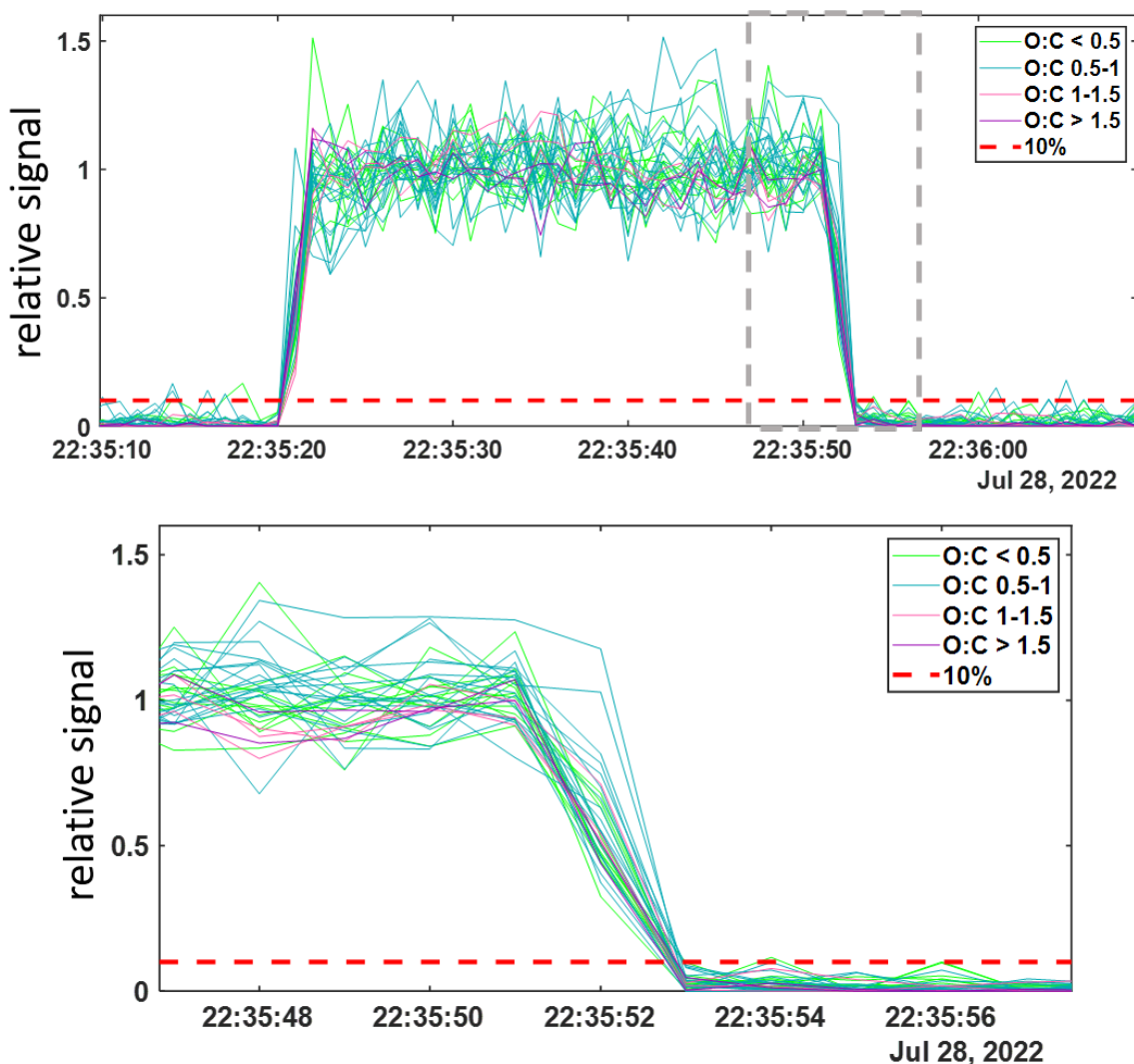
Figure 3. 1 Hz time series of 35 \alpha -pinene ozonolysis products generated in a laboratory study and detected in the t-IMR. Compounds shown colored by O:C ratio and reported in normalized signals relative to the averaged detected during addition. Relative 10% signal lines shown in red. Bottom plot shows zoomed in view of time series as shown in grey box of top plot.
