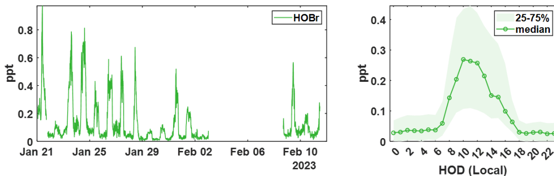
Figure 4. (Left) 15-minute averaged time series of ambient (water-vapor-corrected) HOBr concentrations measured during the winter BLEACH campaign and (right) the diurnal profile showing median signal at each hour of day (HOD) in local time. Shading indicates the bounds of the 25 th and 75 th quartiles for the measured concentrations in each hourly bin.
