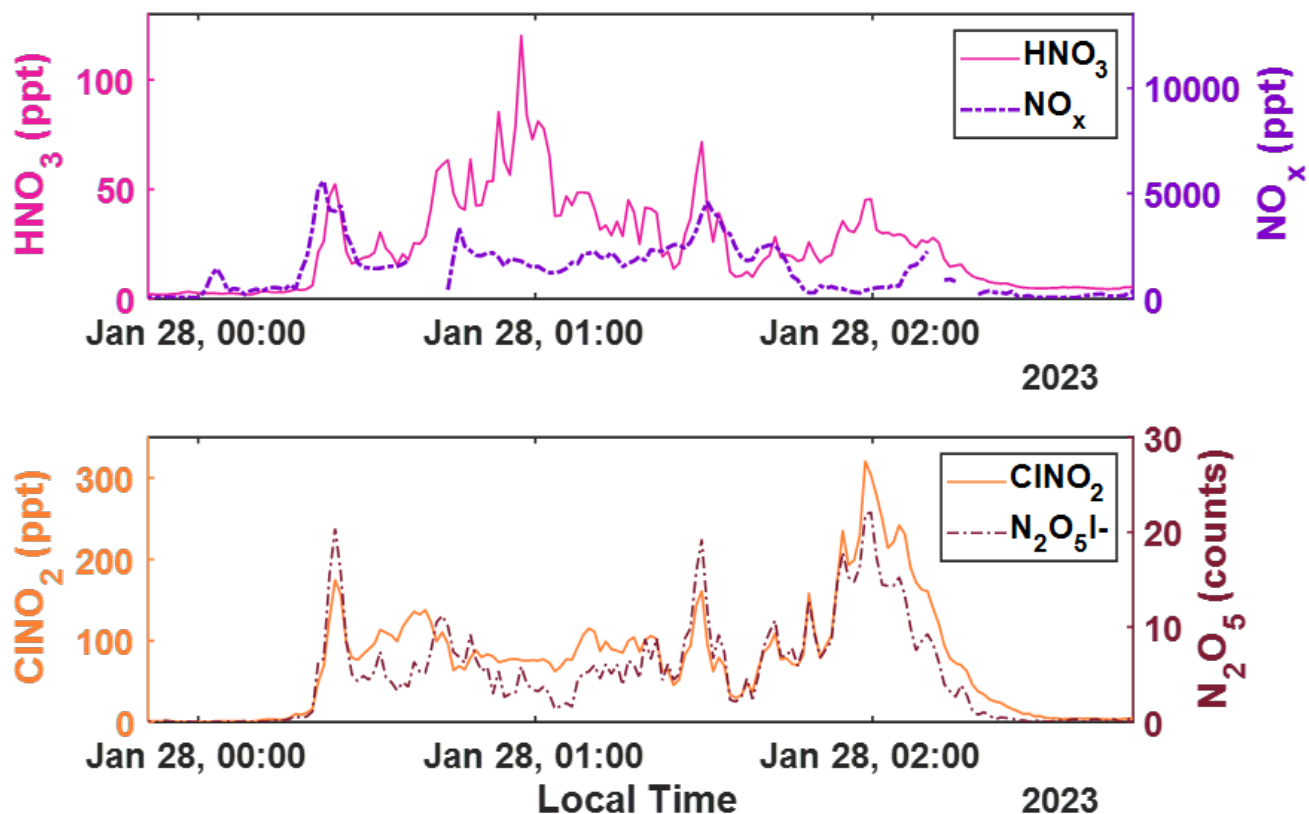
Figure A6. Representative 1-minute time series of (top) \text{HNO}_3 and \text{NO}_x concentrations in magenta and purple dashes, respectively; as well as (bottom) \text{ClNO}_2 concentrations and signal counts of \text{N}_2\text{O}_5 , respectively in orange and dark red dashes. The concentrations and signals of all but \text{HNO}_3 are background subtracted.
