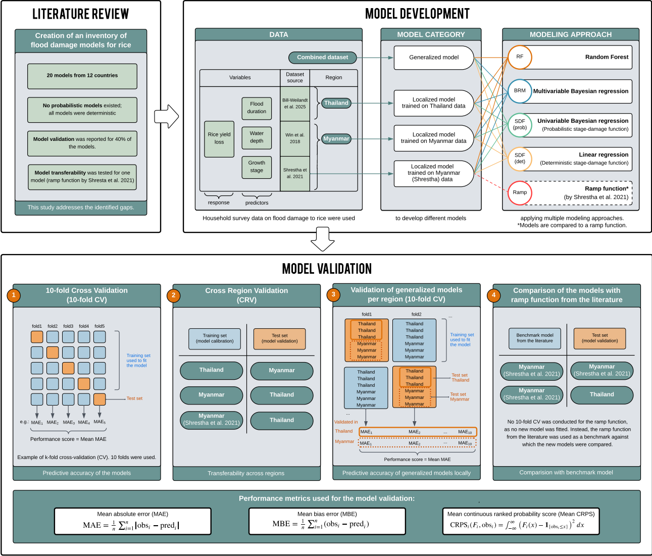
Fig. 3: Visualization of the model development and validation steps. The figure highlights key findings from the literature review that informed the methodological framework. Household survey data were used to develop different models; for each model category, four modeling approaches (boxes with solid lines) were applied. In addition, results were compared against the benchmark ramp function for Myanmar created by Shrestha et al. 2021 (box with dashed line). Three model validation steps were defined. In each step, the same three performance metrics were used.
