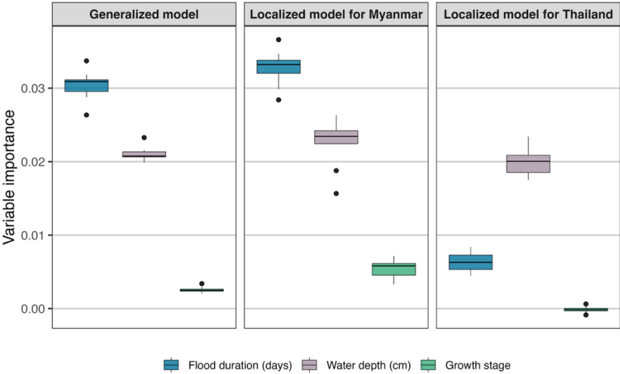
Fig. 6: Box plots indicating the predictor importance for the generalized and localized RF models. Each boxplot shows the median (thick horizontal line), the interquartile range (IQR), the most extreme values within 1.5xIQR (whiskers), and outliers (black points).
