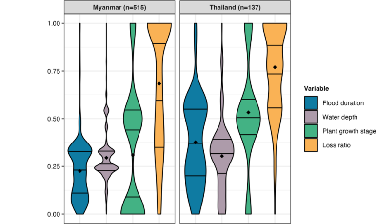
265 Fig. 4: Kernel density estimations of the variable distributions for the Myanmar and Thailand datasets, with lines representing the quartiles and the dots showing the mean. Continuous variables were scaled to the range [0;1] and integers were assigned to each growth stage [(1) "vegetative stage", (2) "reproductive stage", (3) "maturity stage"].
