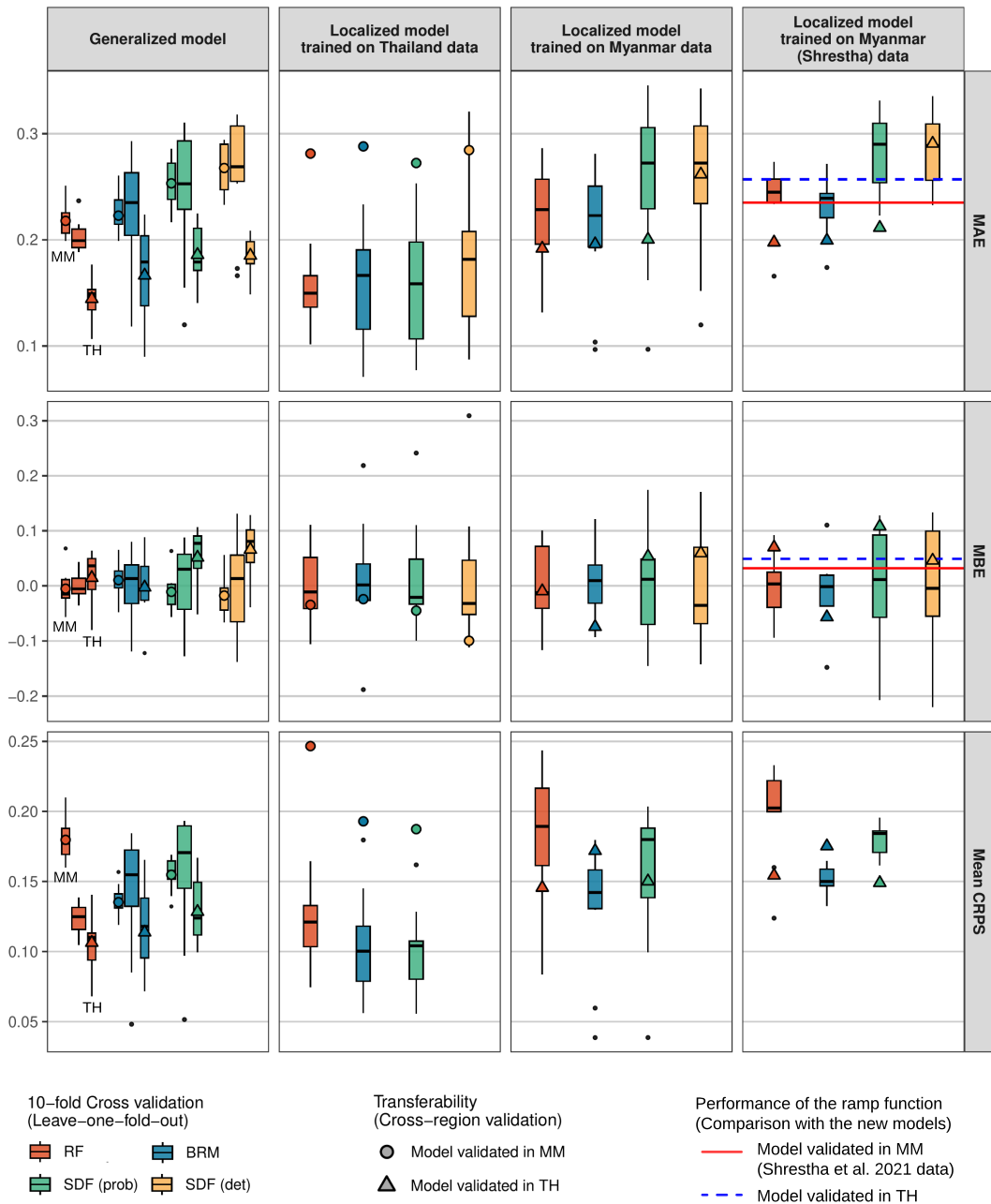
Fig. 5: Results of performance evaluation and transferability assessment. Results are shown for three performance metrics (rows) and four calibration setups (generalized, localized trained on Thailand data and Myanmar data, and localized trained on Myanmar data by Shrestha et al. 2021) (columns). Colors indicate the model types (RF, BRM, probabilistic SDF, and deterministic SDF). Boxplots show the 10-fold cross-validation results. The thick lines show the median; boxes represent the interquartile range (IQR); whiskers extend to 1.5×IQR; and black points are outliers. Each box summarizes variability across 10 folds. For localized models, shapes indicate the performance of transferred models (CRV). For generalized models, shapes indicate mean performance metrics from local validation across ten folds, and the thin boxplots summarize variability in the local validation across the 10 folds. The lines mark the mean performance of the benchmark ramp function in Myanmar (solid red line) and in Thailand (dashed blue lines).
