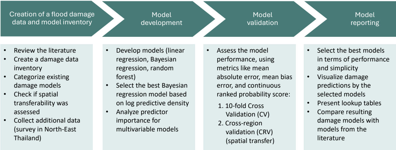
Fig. 2: Methodological framework Crop-Loss-X for damage model development and validation for the agricultural sector through machine learning & model transferability assessments
