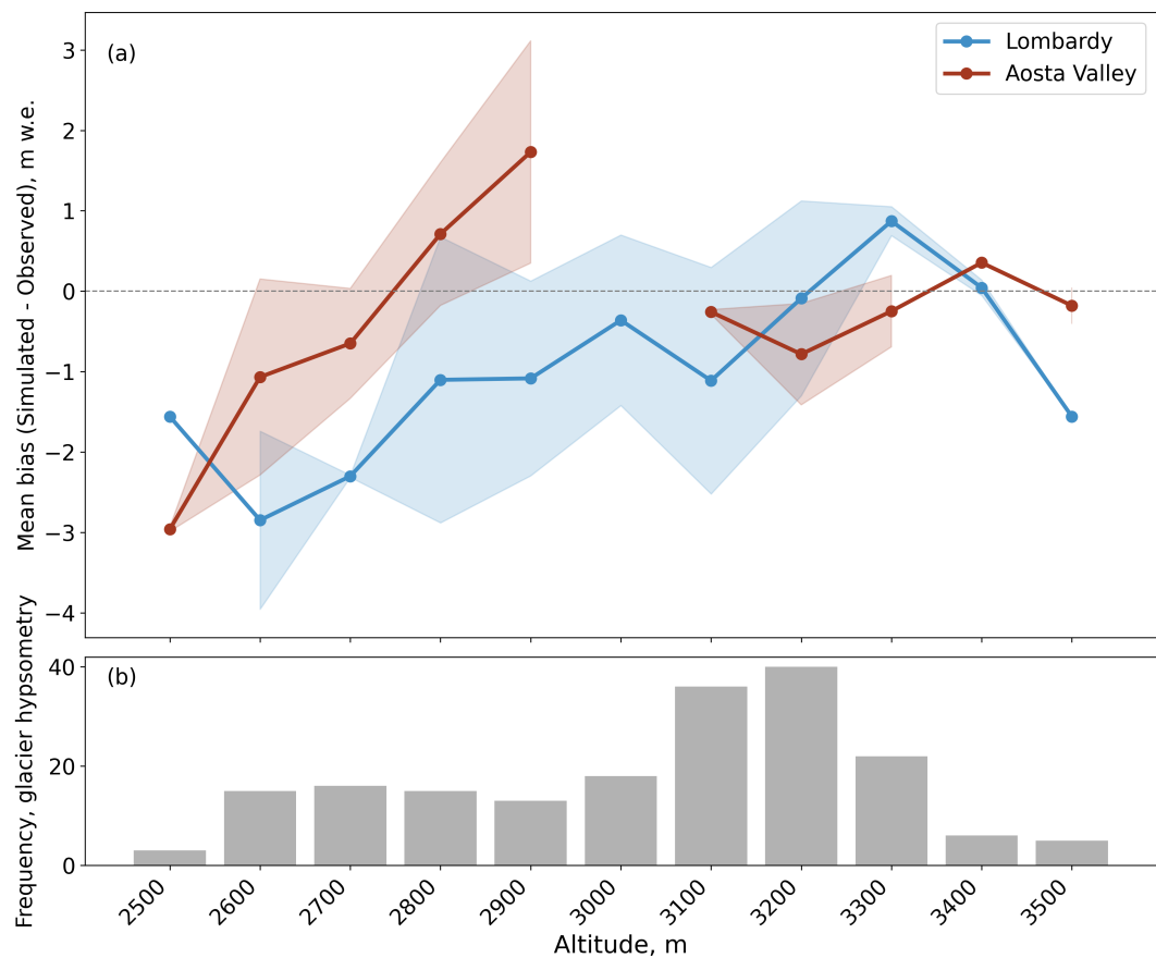
Figure 2. In panel (a), the mean bias of S3M (modeled values) against stake measurements (observed values), binned by elevation, for both Aosta Valley (in red) and Lombardy (in blue). Shaded areas show the standard deviation of the model - observations differences. Missing data points for Aosta Valley are because data were unavailable between 2900-3000 and 3000-3100 m a.s.l.. Panel (b) shows the frequency distribution of glacier elevations in both regions.
