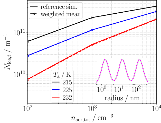
Figure 5. Weighted mean approach for six ambient aerosol populations. Displayed is the final number of ice crystals formed N_{\text{ice},f} as a function of total aerosol number concentration n_{\text{aer},\text{tot}} for different ambient temperatures T_a . The six populations comprise three geometric mean radii \bar{r}_{\text{d},\text{aer}} = \{2, 20, 200\} nm each combined with two hygroscopicities \kappa_{\text{aer}} = \{0.05, 0.5\} (illustrated by the inset; the solid grey and the dotted magenta lines indicate the two hygroscopicities). Each population is assumed to contribute one sixth to the total aerosol number concentration. Reference simulations including all six aerosol populations in a single simulation (solid lines) are compared to the weighted mean approach after Eq. (4) (dashed lines with marker).
