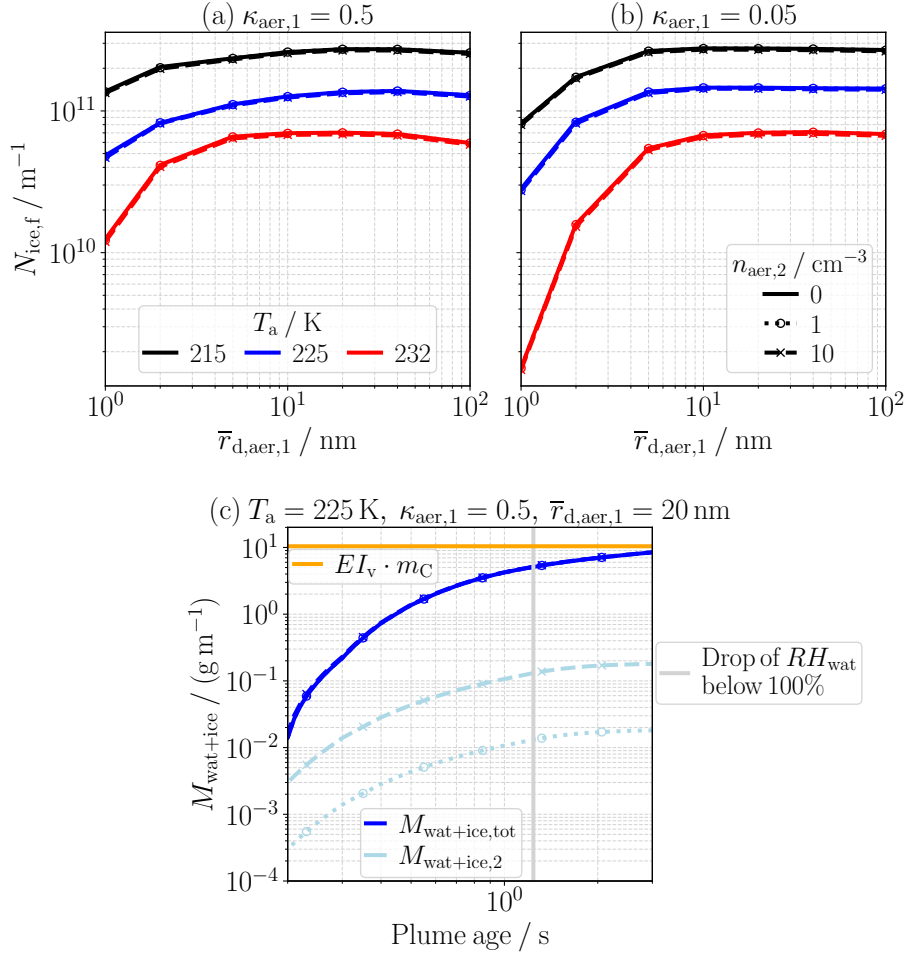
Figure 2. (a)-(b) Impact of coarse mode particles ( \bar{r}_{d,aer,2} = 2000 nm , \kappa_{aer,2} = 0.05 ) on the final number of ice crystals formed N_{ice,f} . In all simulations, the total aerosol number concentration is n_{aer,tot} = n_{aer,1} + n_{aer,2} = 1000 cm^{-3} with varying n_{aer,2} values (different line styles). Shown are results as a function of the geometric radius of the smaller aerosol mode \bar{r}_{d,aer,1} for different ambient temperatures T_a (different colors) and different hygroscopicity combinations (panel). (c) Illustrative example of the evolution of depleted water-vapor mass on droplets and ice crystals. Shown are both the total depleted mass and the portion attributed to coarse-mode particles. The orange horizontal line marks the emitted water-vapor mass corresponding to the fuel consumption of m_C \approx 1.17 g m^{-1} . The vertical grey line indicates the time at which the plume relative humidity with respect to water falls below 100%, marking the approximate end of droplet activation.
