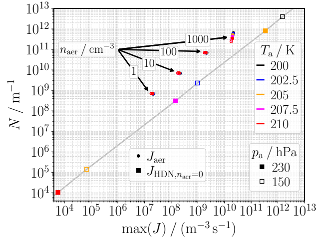
Figure B1. Maximum of nucleation rate \max(J) and integrated number N = \int J(t) \hat{A}(t) dt for different combinations of ambient temperature T_a (indicated by color) and pressure p_a (filled vs. unfilled markers). Results are presented for droplet activation on ambient aerosols (circle markers), obtained from box-model simulations using several aerosol number concentrations n_{aer} . Moreover, results are shown for the HDN rates that would arise if the plume relative humidity and temperature evolved along the mixing line (square markers). These results are connected by the grey line.
