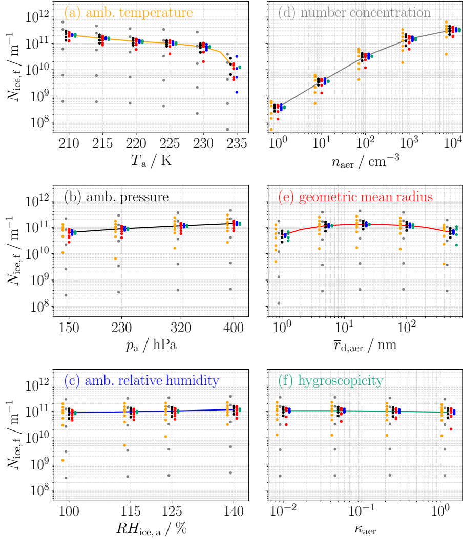
Figure 9. Mean dependence of the final number of ice crystals formed N_{\text{ice},f} on the various parameters (different colored solid lines in each panel). The colored dots show the mean N_{\text{ice},f} calculated within subgroups grouped by the specific parameter value at the x-axis and by the values of a co-parameter. Different colors indicate the various co-parameters, with the corresponding parameter ranges taken from Table 2. The dots for the different co-parameters correspond to the parameter value at the center but are shifted for visualization purposes. In (a), the dependence on the co-parameters is not displayed for T_a = 232.5 \text{ K} and in (e) the dependence on the co-parameters is only displayed for each second geometric mean radius.
