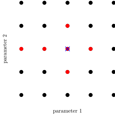
Figure 8. Schematic depiction of the difference between a one-at-a-time approach and the simulation setup used in the current study. Starting from a set of baseline values (blue cross), the values of a single parameter are varied in a one-at-a-time approach while all other parameters are kept constant (red dots). In the current study, we set up simulations for all possible combinations of parameter values (black dots).
