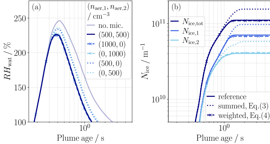
Figure 3. Evolution of (a) plume relative humidity RH_{\text{wat}} and (b) ice crystal number N_{\text{ice}} at an ambient temperature of T_a = 225 \text{ K} for a case with two aerosol populations ( n_{\text{aer},1} = n_{\text{aer},2} = 500 \text{ cm}^{-3} , \kappa_{\text{aer},1} = \kappa_{\text{aer},2} = 0.5 , \bar{r}_{\text{d,aer},1} = 20 \text{ nm} , \bar{r}_{\text{d,aer},2} = 2 \text{ nm} ). (a) Shown is the RH_{\text{wat}} evolution from a simulation excluding microphysical water-vapor depletion (transparent line), together with the evolution when both aerosol populations are included simultaneously (dark-blue line). Also shown are simulation results including only one population at a time, using its respective properties and either its actual number concentration or the total number concentration (different colors and linestyles). (b) Displayed are the total ice crystal number N_{\text{ice,tot}} and the contributions from the two aerosol populations, N_{\text{ice},1} and N_{\text{ice},2} . Additionally, the approximations obtained from Eqs. (3) and (4) are shown.
