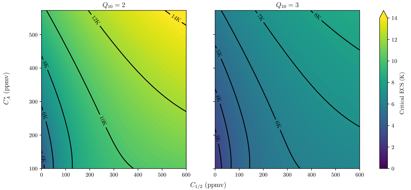
Figure 5. The critical ECS as a function of pre-industrial \text{CO}_2 levels, C_A^* , and the \text{CO}_2 fertilisation effect for two different values of Q_{10} . Notice the critical ECS is smaller for smaller pre-industrial \text{CO}_2 levels, \text{CO}_2 fertilisation strength and larger Q_{10} .
