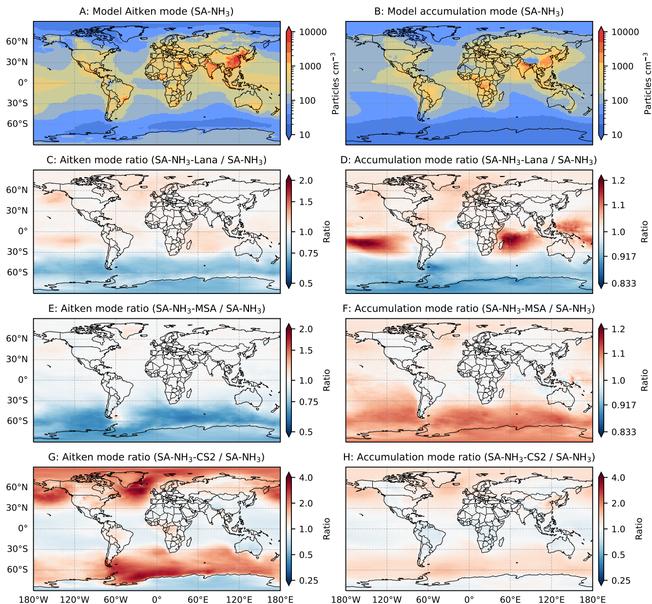
Figure 12. Global distribution of marine boundary layer aerosol changes following implementation of the Lana et al. (2011) DMS climatology, MSA condensation and CRI-Strat2 scheme. Panels show aerosol number concentrations in the marine boundary layer (0 - 2 km altitude) averaged over monthly data from July 2016 to June 2018: (A) Aitken mode aerosols from the benchmark SA-NH 3 simulation, (B) accumulation mode aerosols from the benchmark SA-NH 3 simulation, (C) ratio of Aitken mode concentrations between SA-NH 3 -Lana and benchmark SA-NH 3 simulations, and (D) ratio of accumulation mode concentrations between SA-NH 3 -Lana and benchmark SA-NH 3 simulations, (E) ratio of Aitken mode concentrations between SA-NH 3 -MSA and benchmark SA-NH 3 simulations, and (F) ratio of accumulation mode concentrations between SA-NH 3 -MSA and benchmark SA-NH 3 simulations, (G) ratio of Aitken mode concentrations between SA-NH 3 -CS2 and benchmark SA-NH 3 simulations, and (H) ratio of accumulation mode concentrations between SA-NH 3 -CS2 and benchmark SA-NH 3 simulations.
