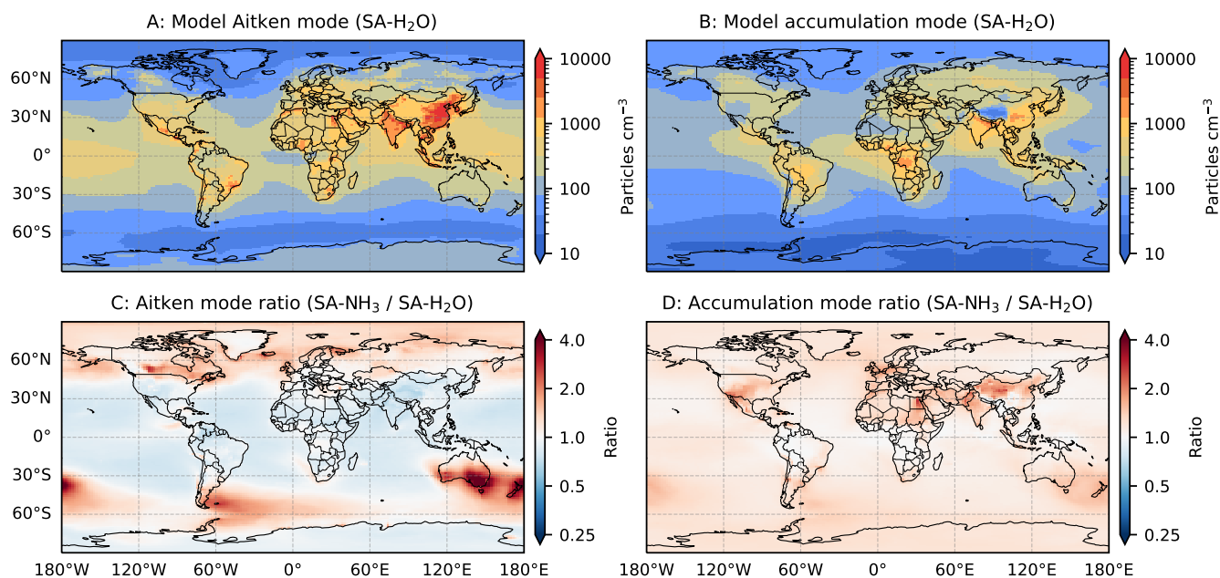
Figure 11. Global distribution of marine boundary layer aerosol changes following implementation of the \text{H}_2\text{SO}_4\text{--NH}_3 nucleation mechanism. Panels show aerosol number concentrations in the marine boundary layer (0 - 2 km altitude) averaged over monthly means from July 2016 to June 2018: (A) Aitken mode aerosols from the default SA-H 2 O simulation, (B) accumulation mode aerosols from the default SA-H 2 O simulation, (C) ratio of Aitken mode concentrations between benchmark SA-NH 3 and default SA-H 2 O simulations, and (D) ratio of accumulation mode concentrations between benchmark SA-NH 3 and default SA-H 2 O simulations.
