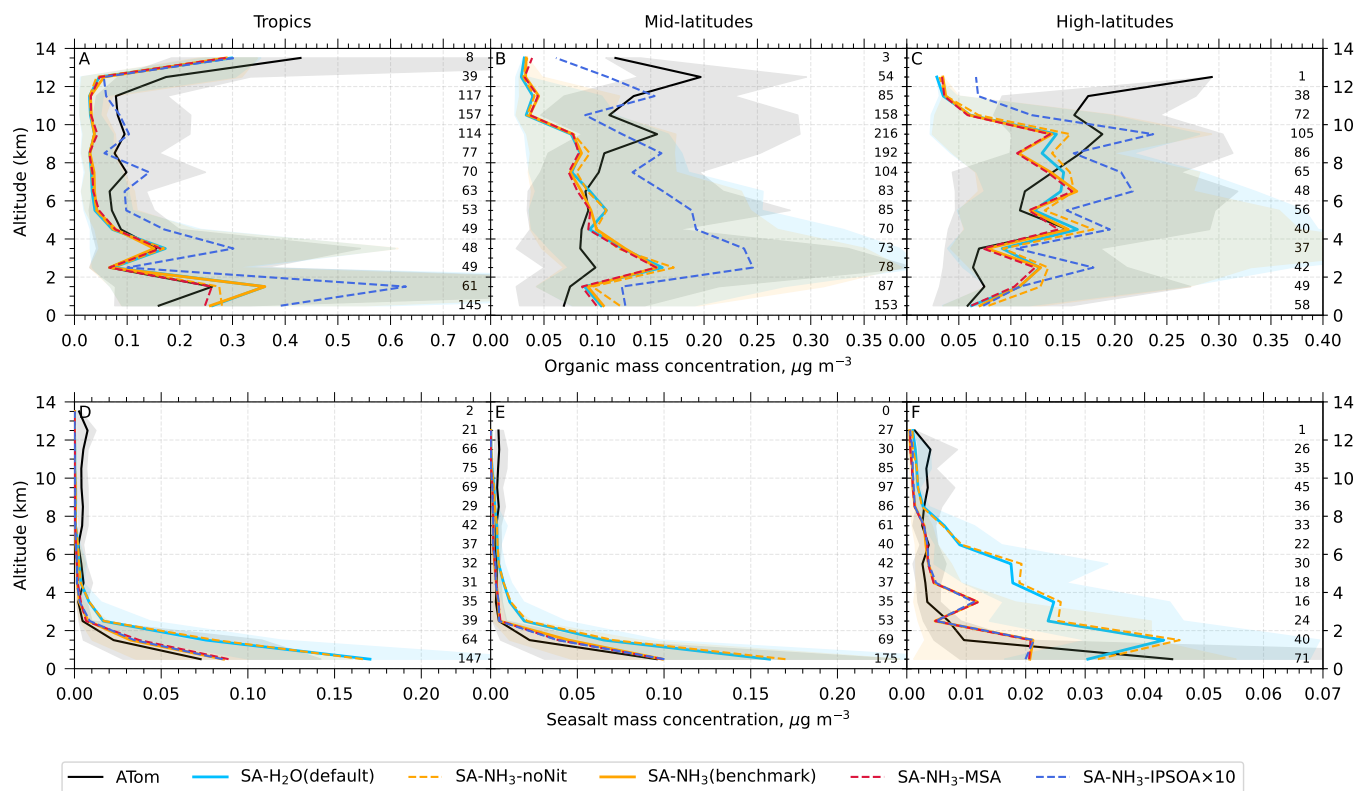
Figure A3. Vertical profiles of organic and seasalt mass concentrations in particles smaller than 1 \mu\text{m} ( \mu\text{g m}^{-3} ). ATom observations (black lines) and selected model simulations (coloured lines; see Table 2 for simulation details) are presented. Median values are shown for organic mass concentrations in the tropics (A, 25 °S to 25 °N), mid-latitudes (B, 25 - 60 °N/S), and high-latitudes (C, 60 - 90 °N/S), and for seasalt mass concentrations in the tropics (D), mid-latitudes (E), and high-latitudes (F). Shaded areas for solid lines represent the interquartile range (25th to 75th percentiles) for both ATom observations and model simulations, indicating the variability in aerosol concentrations. Numbers on the right edge of each panel show the sample size used to calculate median values for each altitude bin at 5-minute temporal resolution.
