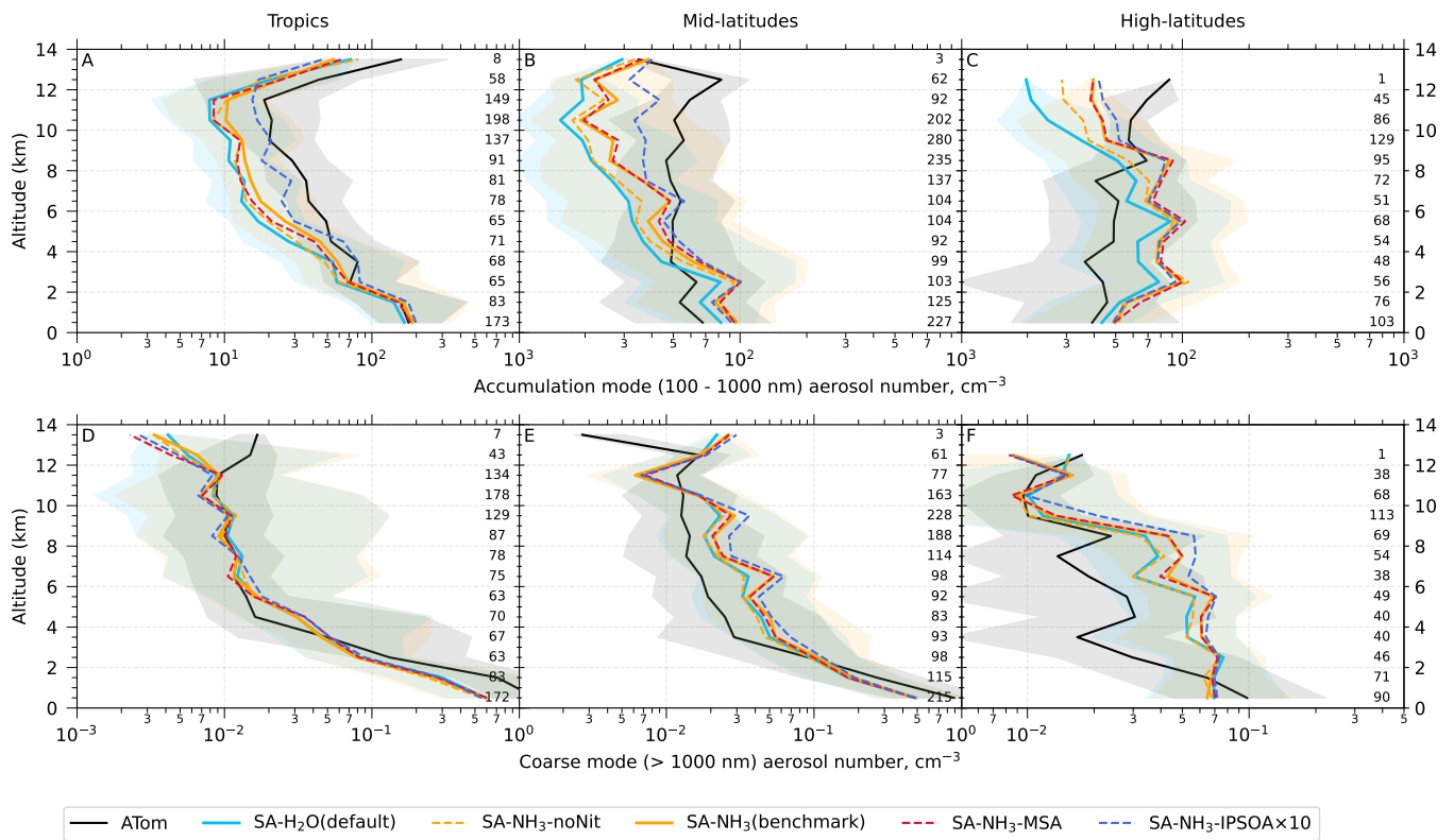
Figure A1. Vertical profiles of accumulation mode (100 - 1,000 nm) and coarse mode (1,000 - 10,000) aerosol number concentrations. ATom observations (black lines) and selected model simulations (coloured lines; see Table 2 for simulation details) are presented. Median values are shown for accumulation mode aerosols in the tropics (A, 25 °S to 25 °N), mid-latitudes (B, 25 - 60 °N/S), and high-latitudes (C, 60 - 90 °N/S), and for coarse mode aerosols in the tropics (D), mid-latitudes (E), and high-latitudes (F). Shaded areas for solid lines represent the interquartile range (25th to 75th percentiles) for both ATom observations and model simulations, indicating the variability in aerosol concentrations. Numbers on the right edge of each panel show the sample size used to calculate median values for each altitude bin at 5-minute temporal resolution.
