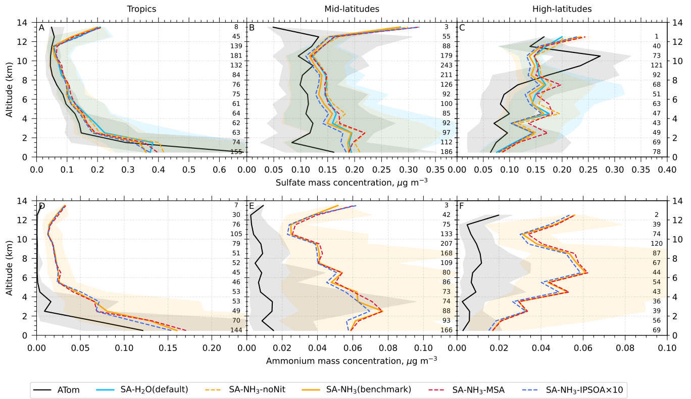
Figure A2. Vertical profiles of sulfate and ammonium mass concentrations in particles smaller than 1 \mu\text{m} ( \mu\text{g m}^{-3} ). ATom observations (black lines) and selected model simulations (coloured lines; see Table 2 for simulation details) are presented. Median values are shown for sulfate mass concentrations in the tropics (A, 25^\circ\text{S} to 25^\circ\text{N} ), mid-latitudes (B, 25^\circ - 60^\circ\text{N/S} ), and high-latitudes (C, 60^\circ - 90^\circ\text{N/S} ), and for ammonium mass concentrations in the tropics (D), mid-latitudes (E), and high-latitudes (F). Shaded areas for solid lines represent the interquartile range (25th to 75th percentiles) for both ATom observations and model simulations, indicating the variability in aerosol concentrations. Numbers on the right edge of each panel show the sample size used to calculate median values for each altitude bin at 5-minute temporal resolution.
