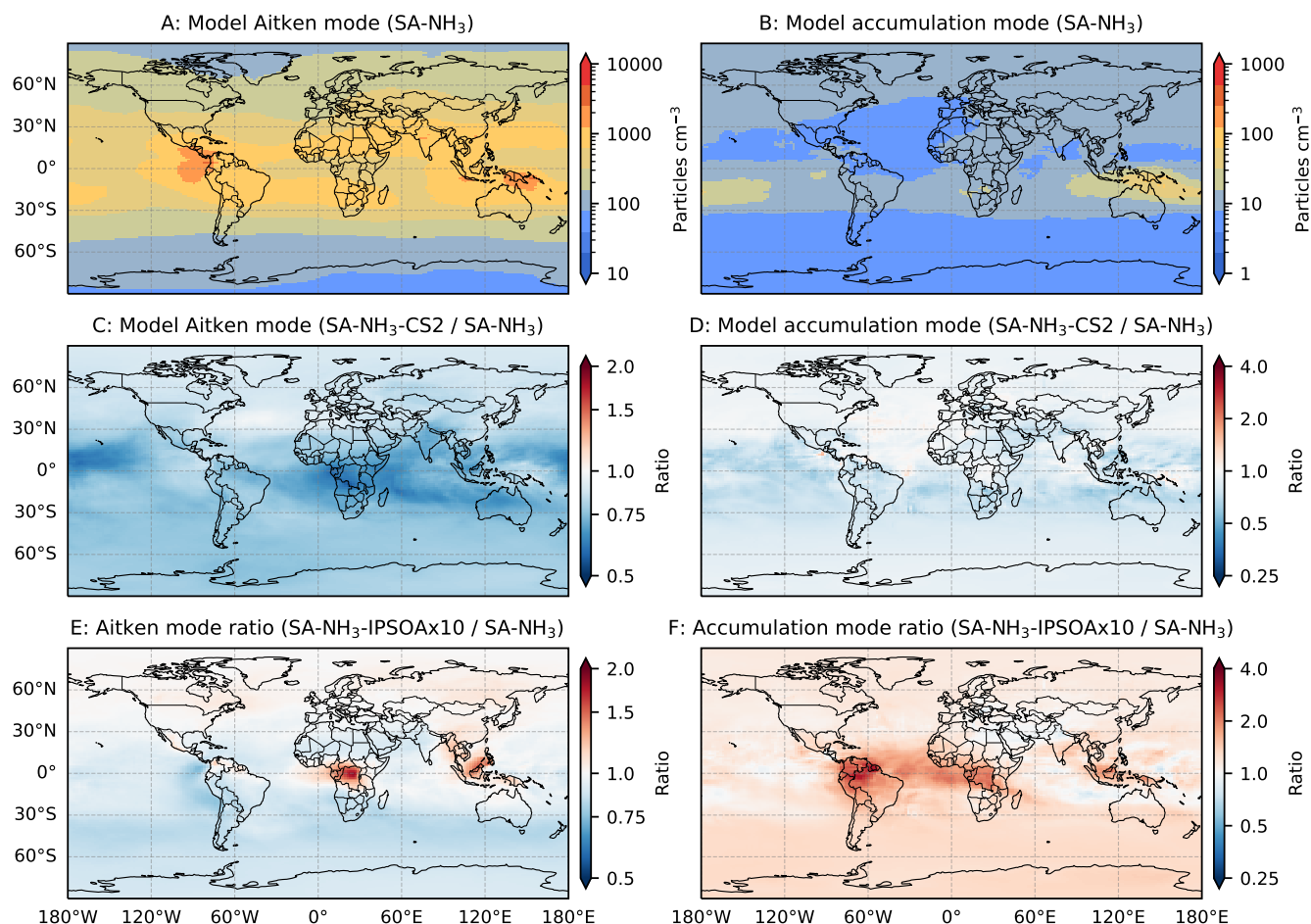
Figure 13. Global distribution of upper tropospheric aerosol changes following implementation of the CRI-Strat2 scheme and isoprene secondary organic aerosol formation scheme. Panels show aerosol number concentrations in the upper troposphere (8 - 12 km altitude) averaged over monthly means from July 2016 to June 2018: (A) Aitken mode aerosols from the benchmark SA-NH 3 simulation, (B) accumulation mode aerosols from the benchmark SA-NH 3 simulation, (C) ratio of Aitken mode concentrations between SA-NH 3 -CS2 and benchmark SA-NH 3 simulations, and (D) ratio of accumulation mode concentrations between SA-NH 3 -CS2 and benchmark SA-NH 3 simulations, (E) ratio of Aitken mode concentrations between SA-NH 3 -IPSOA×10 and benchmark SA-NH 3 simulations, and (F) ratio of accumulation mode concentrations between SA-NH 3 -IPSOA×10 and benchmark SA-NH 3 simulations.
