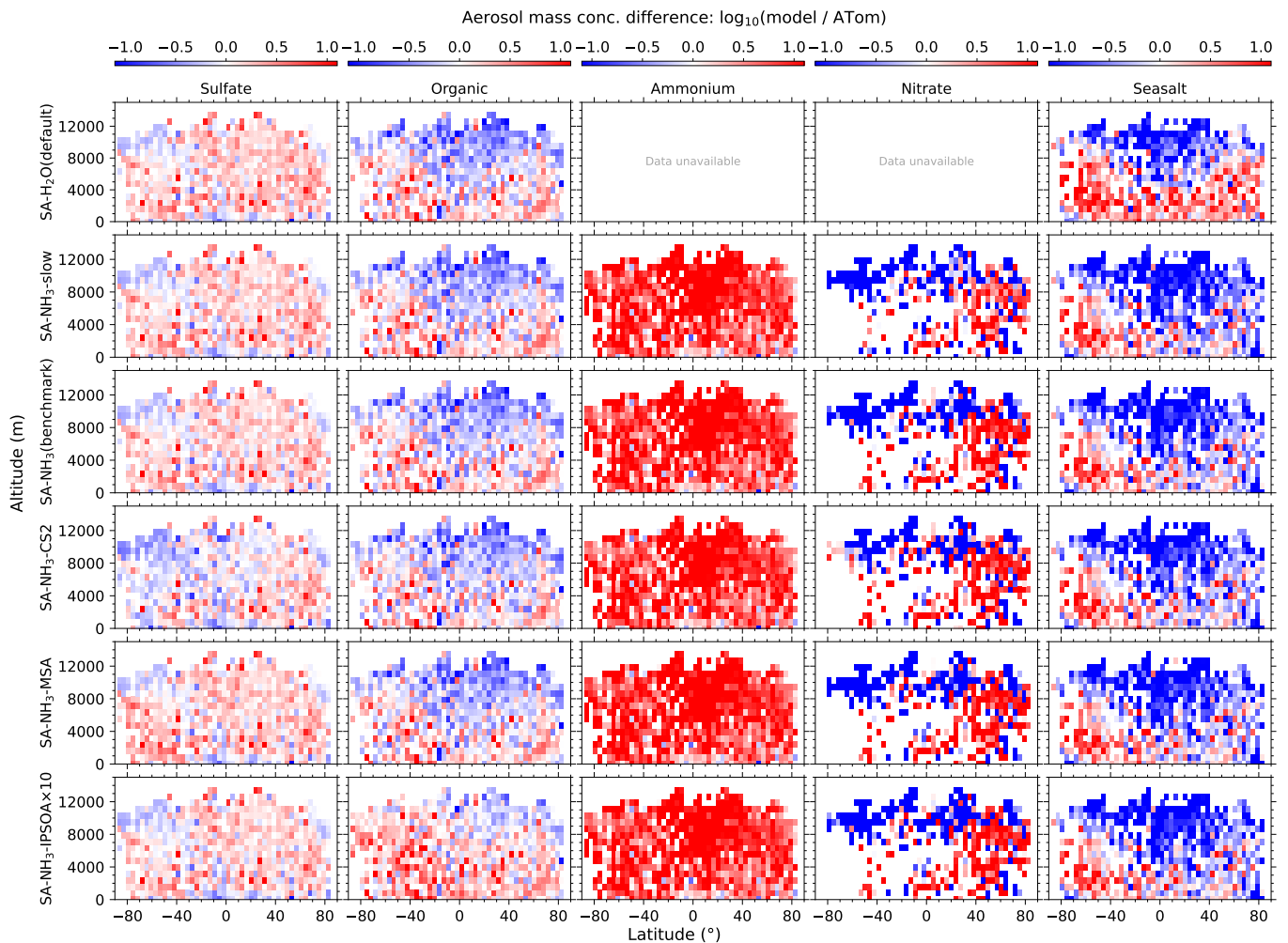
Figure 10. Curtain plots of model-to-ATom ratios for aerosol composition along ATom flight tracks. Mean ratios of modelled to observed values for sulfate, organic, ammonium, nitrate and seasalt mass concentrations are shown for selected model simulations (see Table 2 for simulation details). Model outputs are interpolated to ATom flight coordinates and times. Data are displayed on a logarithmic scale with a diverging colour scheme where values greater than 1 indicate model overestimation and values less than 1 indicate model underestimation. Colour scales are consistent within each column to facilitate comparison between different model configurations. The SA-H 2 O (default) simulation does not include ammonium or nitrate in aerosols, thus the absence of data in the corresponding plots.
