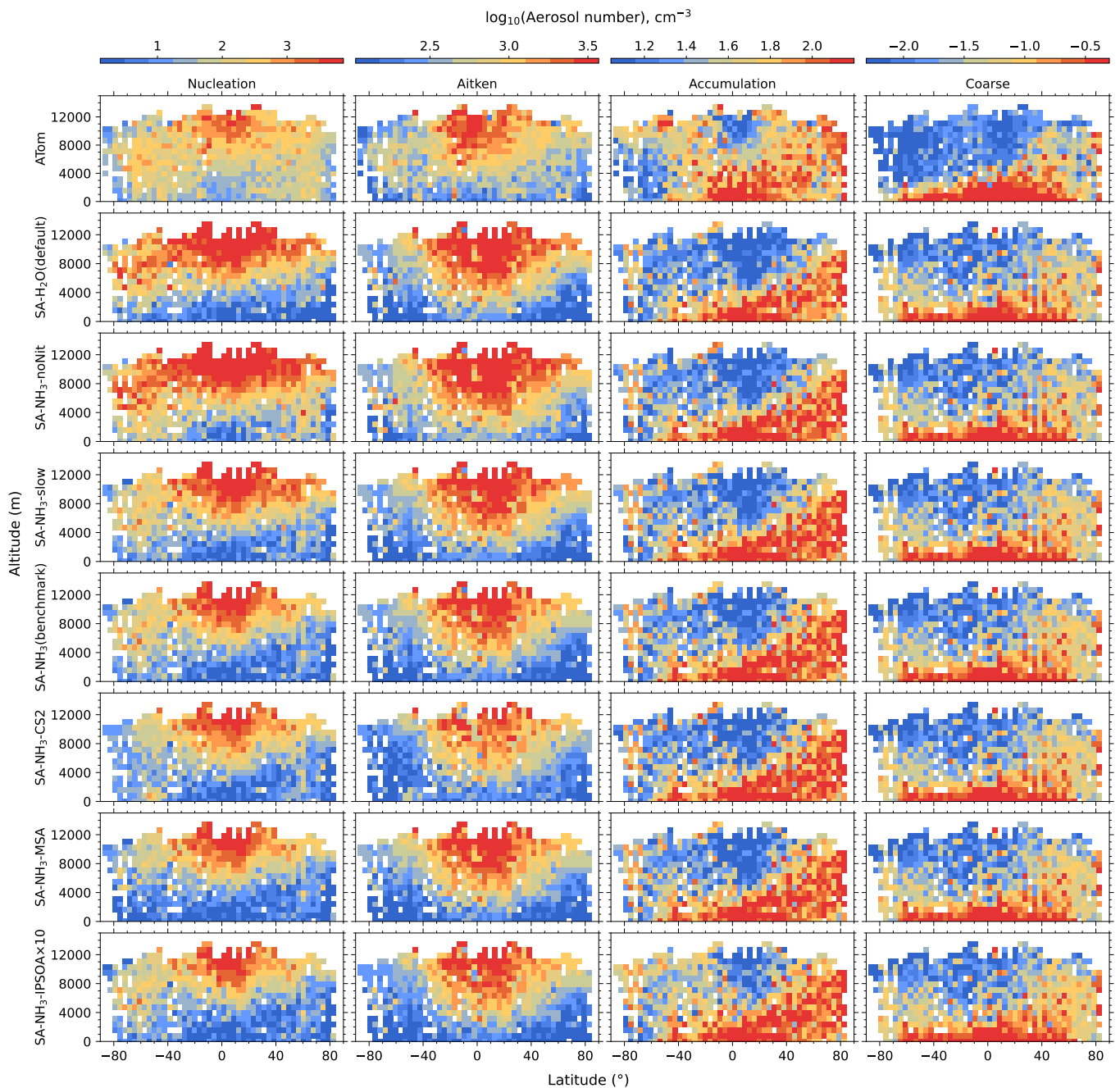
Figure 5. Curtain plots of aerosol number size distribution along ATom flight tracks. Mean nucleation mode ( < 10 nm), Aitken mode (10 - 100 nm), accumulation mode (100 - 1000 nm), and coarse mode (1000 - 10,000 nm) aerosol number concentrations are shown for ATom observations (first row) and selected model simulations (subsequent rows; see Table 2 for simulation details). Model outputs are interpolated to ATom flight coordinates and times. All data are displayed on a logarithmic axis to enhance visualisation of the variations in parameters. Colour scales are consistent within each column to facilitate direct comparison between observations and model simulations.
