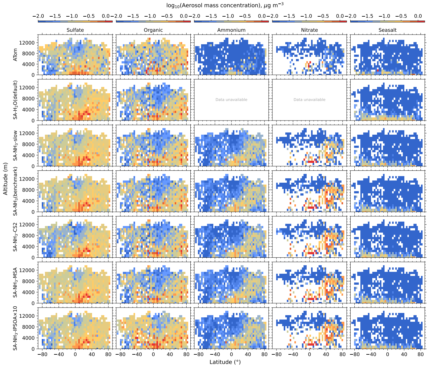
Figure 9. Curtain plots of aerosol composition along ATom flight tracks. Mean sulfate, organic, ammonium, nitrate and seasalt mass concentrations are shown for ATom observations (first row) and selected model simulations (subsequent rows; see Table 2 for simulation details). Model outputs are interpolated to ATom flight coordinates and times. All data are displayed on a logarithmic to enhance visualisation of the variations in parameters. Colour scales are consistent within each column to facilitate direct comparison between observations and model simulations. The SA-H 2 O (default) simulation does not include ammonium or nitrate in aerosols, thus the absence of data in the corresponding plots.
