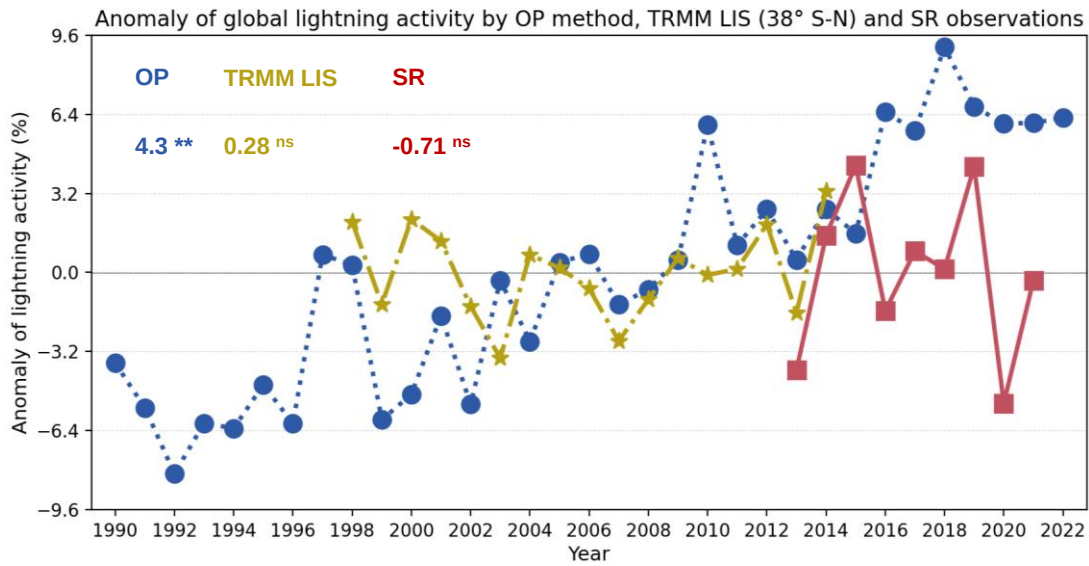
175 Figure 3: Anomaly of global lightning activity based on OP method, TRMM LIS (38°S–38°N), and SR observations. The linear trends (% dec -1 ) are shown in the upper left. ** denotes significant trends ( P < 0.05 ), * moderately significant trends ( 0.05 \leq P < 0.1 ) and ns insignificant trends.
