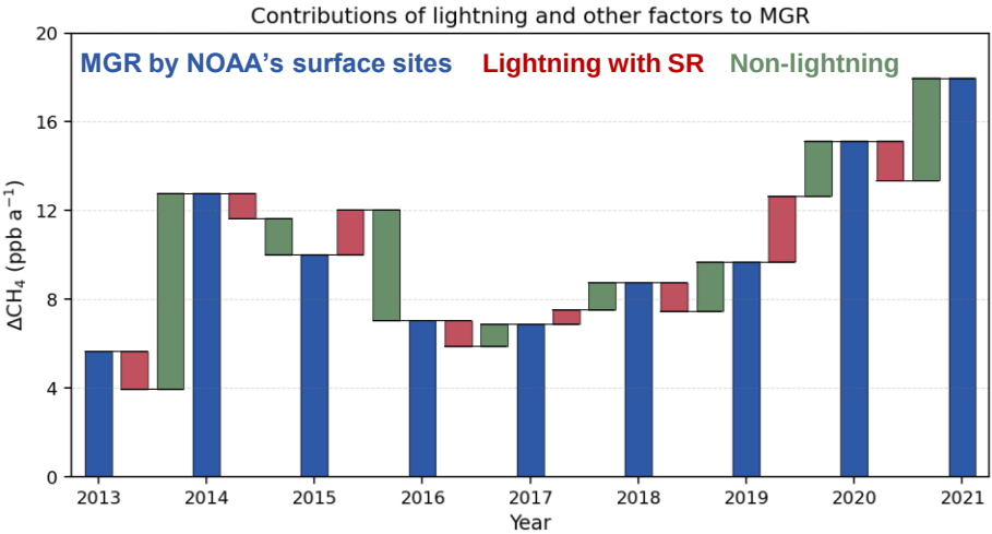
260 Figure 6: Contributions of lightning-driven variations in the methane sink by OH oxidation to annual atmospheric methane growth rate (MGR) from 2013 to 2021 based on SR observations. The gap between observed year-to-year anomalies in MGR and simulated lightning contribution is attributed to non-lightning factors.
