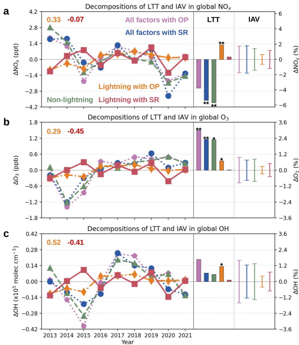
210 Figure 4: Annual anomalies, LTT, and IAV of global \text{NO}_x (a), \text{O}_3 (b) and OH (c), and their decompositions into lightning and non-lightning factors during 2013–2021. LTT values are reported in the unit of \% \text{ dec}^{-1} . ** denotes significant trends ( P < 0.05 ) and * moderately significant trends ( 0.05 \leq P < 0.1 ). IAV values represent standard deviation of annual anomalies after LTT is removed. Shown in the upper left of each panel are correlation coefficients between the annual anomalies (with LTTs removed) of lightning (OP: orange; SR: red) and non-lightning contributions.
