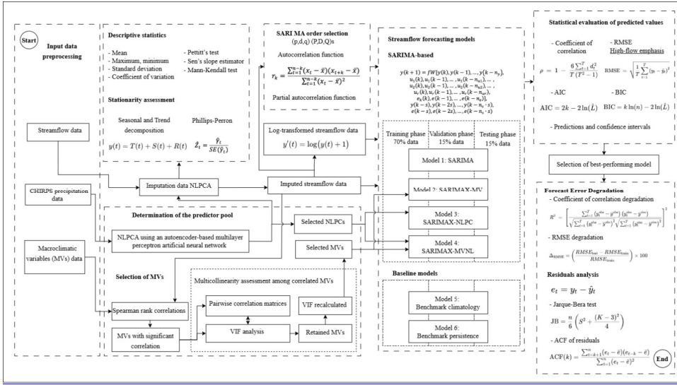
Figure 1: Schematic representation overview of the methodological workflow for, including input data preprocessing, determination of the predictor pool, streamflow forecasting under data-scarce conditions, and performance evaluation of the best-performing model.
