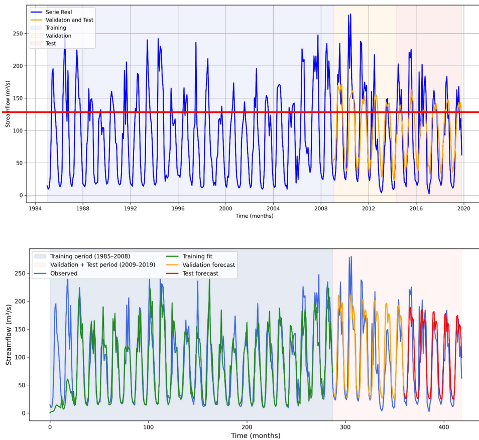
Figure 10: Observed and predicted streamflow for training and validation using the NNLOG-SARIMAX-MVNL model.
