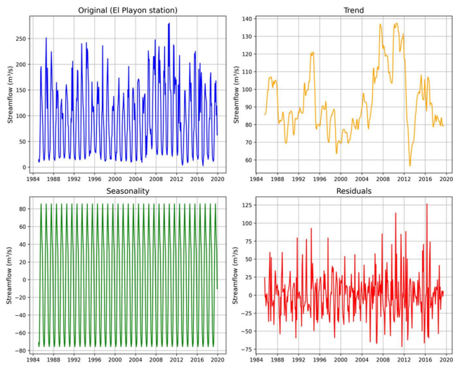
340 Figure 5: Decomposition of El Playón streamflow time series into trend, seasonality, and residual components.
