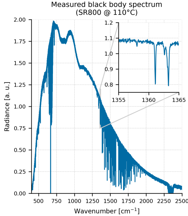
Figure 1. Hot black-body blackbody spectrum containing lab air absorption lines as observed by the NYAEM-FTS in Ny-Ålesund, Svalbard.
