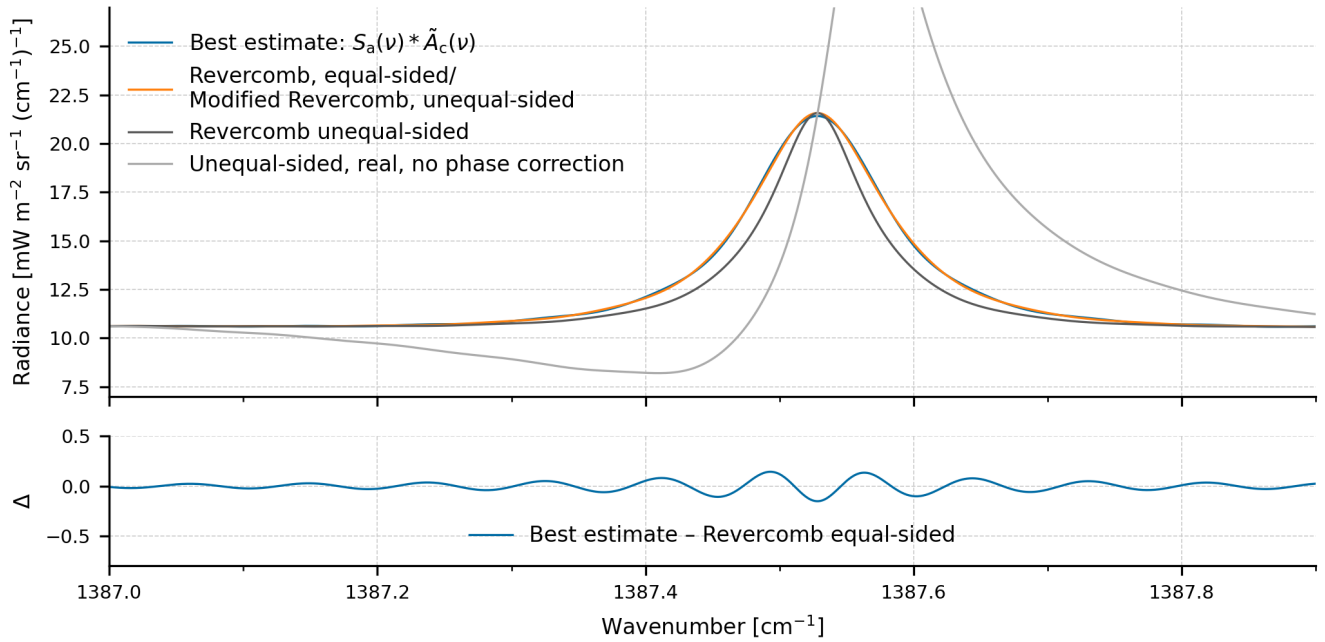
Figure 3. Upper panel: The best spectral estimate in FTIR spectroscopy, given by the atmospheric spectrum convolved with the real scanning function from symmetric truncation (Eq. 20), is shown in blue. The spectral estimate from total power calibration, given by either symmetric truncation in the Revercomb formula or equivalently by applying the modified calibration method presented in this work to unequal-sided interferograms, is shown in orange. The spectral estimate resulting from applying the standard Revercomb formula to unequal-sided interferograms is shown in dark gray. The estimate resulting from applying the incompletely modified Revercomb formula (real parts only but without phase correction) to unequal-sided interferograms is shown in light gray. Lower panel: Difference between the best estimate without calibration and the estimate with calibration.
