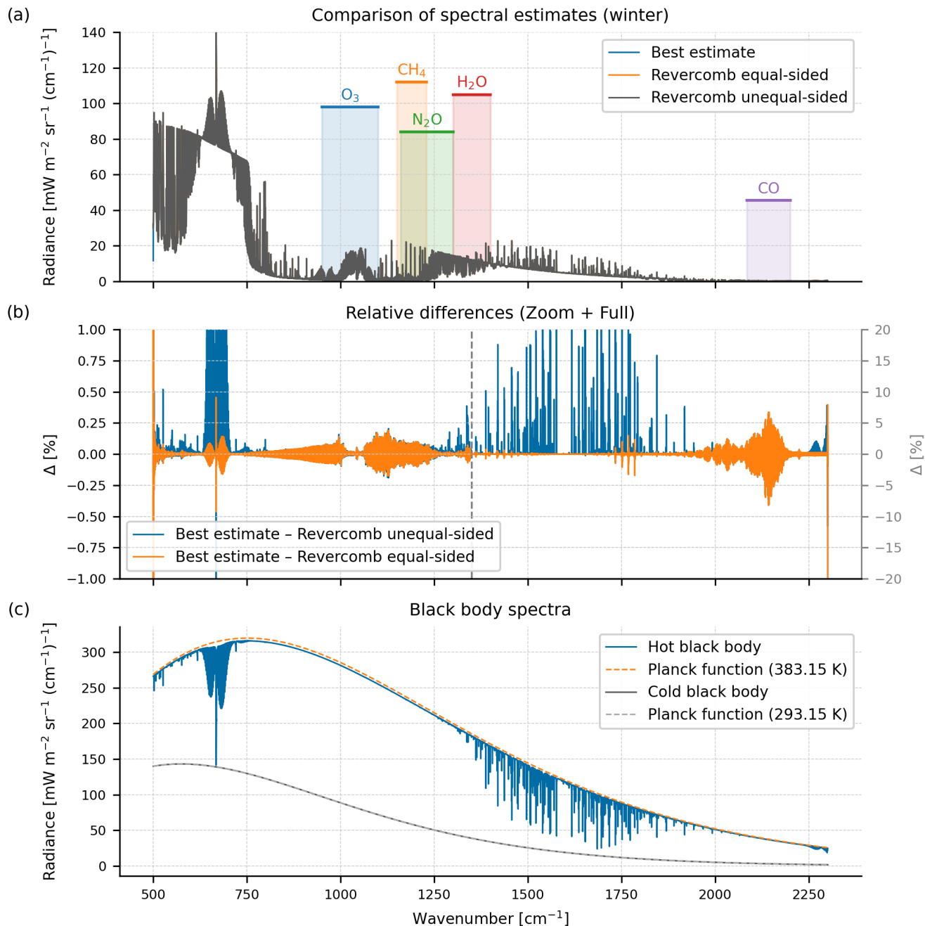
Figure 4. As in figure Figure 3 , the first panel shows the best estimate in blue, the Revercomb calibration for equal-sided interferograms (modified method for unequal-sided interferograms) in orange and the application of the complex-original Revercomb method to unequal-sided interferograms in gray, but for a larger part of the spectrum entire measured mid-infrared spectral range . The second panel shows the relative differences. In the left part, where absorption lines are small in the black-body-blackbody spectrum, the differences are minor and become larger the stronger the absorption lines in the black-body-blackbody spectrum as can be seen on the right hand side (note the different axis scalings). The black-body-blackbody spectra are shown in the bottom panel. All are synthetic spectra from a realistic Arctic atmospheric winter profile (see Fig. 2) .
