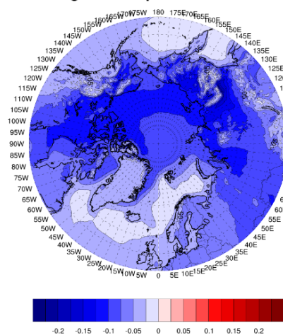
Dec Average d\theta/dp 1000-850 mb 1980-2024
