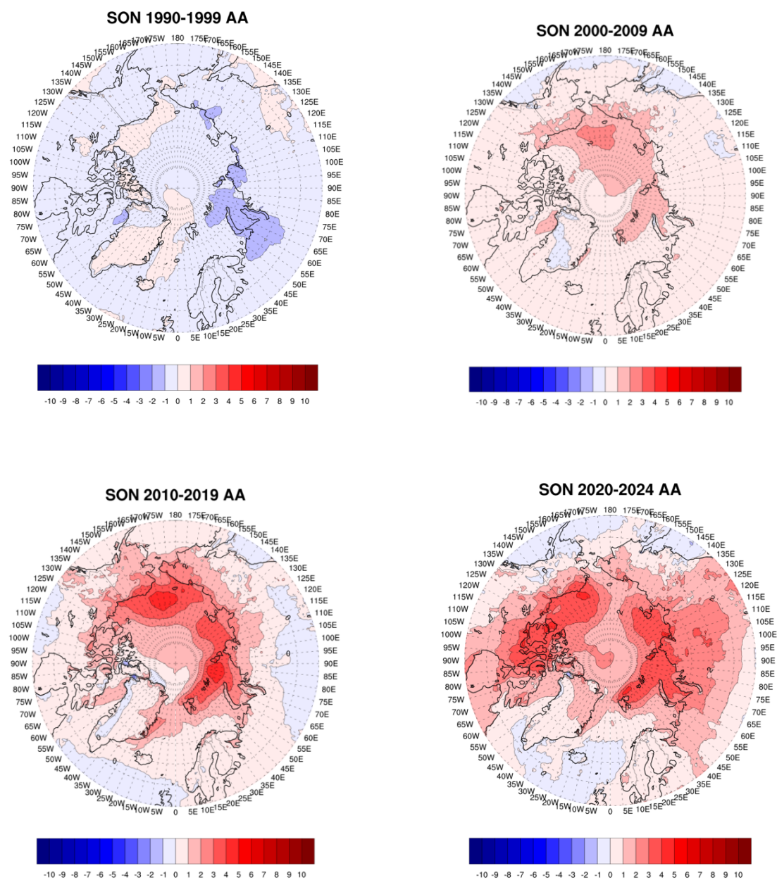
Figure 3. Autumn 2-m temperature anomalies in °C relative to 1981-2010 for 1990-1999, 2000-2009, 2010-2019 and 2020-2024 185 minus the global average temperature anomaly for each period.
