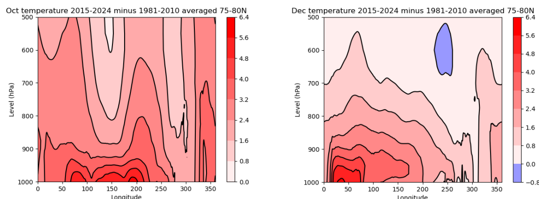
Figure 5: Vertical cross sections by longitude across latitudes 75°N to 80°N for October (left) and December (right) of temperature anomalies for 2015-2024 minus 1981-2010.
