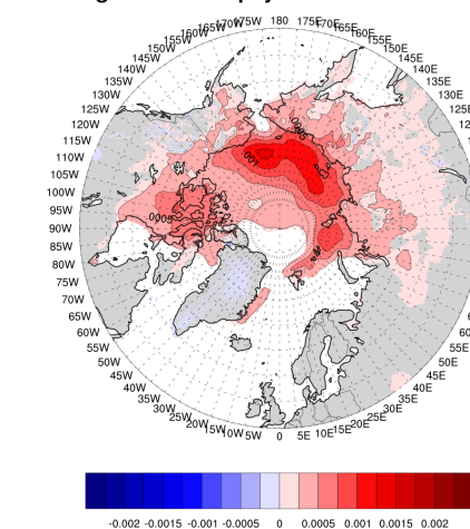
Oct change in dtheta/dp /year 1000-850 mb 1980-2024
