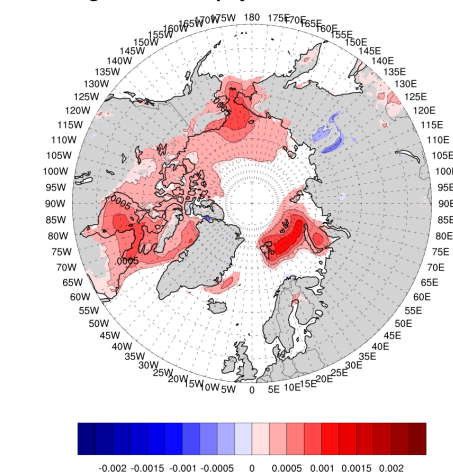
Dec change in d\theta/dp /year 1000-850 mb 1980-2024
