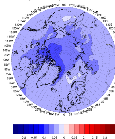
Oct Average dtheta/dp 1000-850 mb 1980-2024
