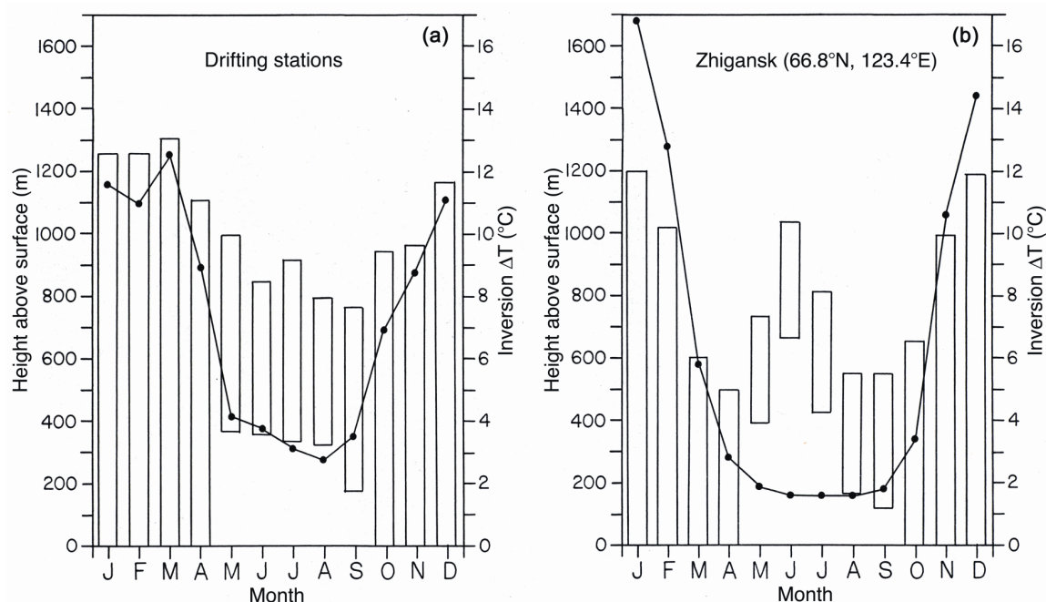
265 Figure 6: Monthly median inversion top (top of bars), base (bottom of bars) and temperature difference (solid lines) from (a) drifting station data from the central Arctic Ocean; (b) station Zhigansk over the Siberian tundra, taken as representative of the region [from Serreze et al., 1992, by permission of AMS].
