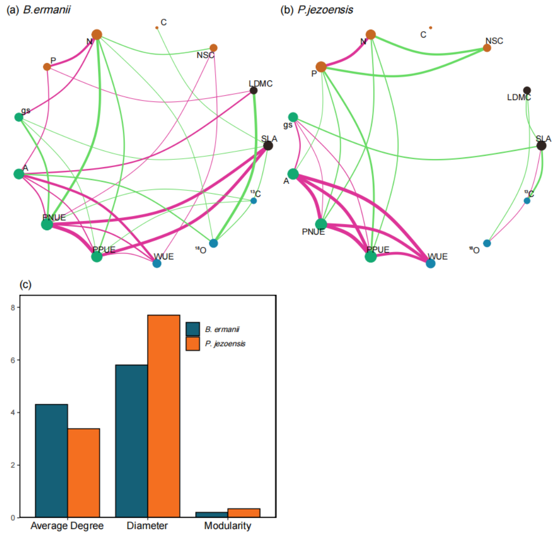
Figure 4. Network of leaf functional traits of (a) B. ermanii and (b) P. jezoensis . Pink lines indicate significant positive correlations ( p < 0.05 ), and green lines indicate significant negative correlations. (c) showed the overall parameters of both leaf functional trait network. The parameter descriptions are provided in Table S2.
