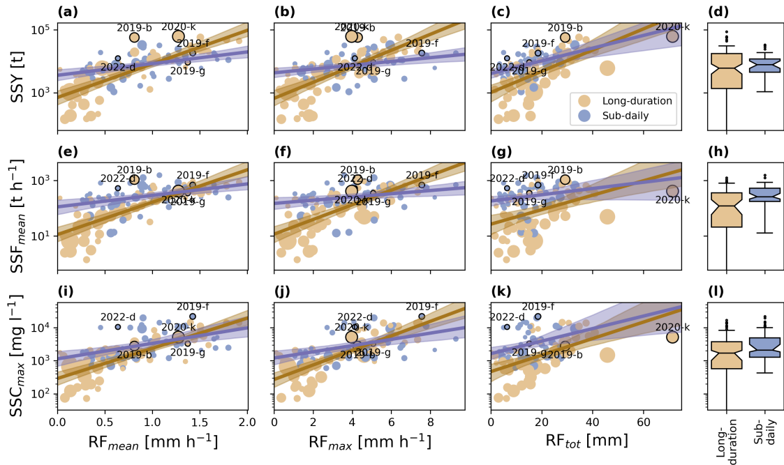
Figure 6. Suspended sediment response to heavy precipitation events in Tumpen-Ötztal (107 events between 2011-2022) in terms of their mean intensity of catchment-averaged rainfall RF_{mean} (a,e,i), maximum intensity of catchment-averaged rainfall RF_{max} (b,f,j), and total cumulative catchment-averaged rainfall RF_{tot} (c,g,k). There are 58 long-duration and 49 sub-daily heavy precipitation events. Dot size indicates the duration of events. Lines are means from linear regression, and shaded areas are 95% bootstrap confidence intervals based on 1000 randomisations. Labelled events are the same as in Fig. 4. See Fig. 4 for details on boxplot configuration.
