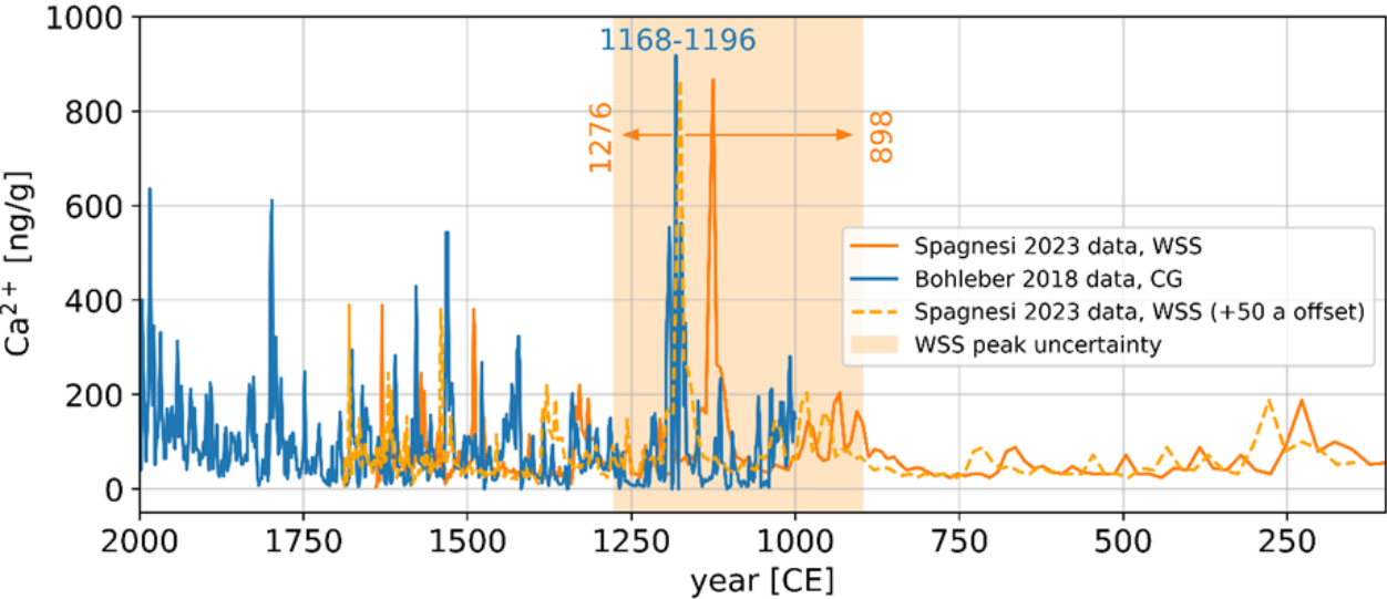
390 Figure 6: \text{Ca}^{2+} data from WSS (Spagnesi et al., 2023) are plotted against time using the conversion of depth to age derived in this work. \text{Ca}^{2+} data from Colle Gnifetti (Bohleber et al., 2018) are plotted for comparison. The shaded area and its boundary values indicate the 1\sigma age uncertainty of the major peak of the WSS data set due to its time scale uncertainty. The blue values indicate the extent of the CG peak in years, not considering its time scale uncertainties. Adding a 50 a offset to the WSS timescale results in good alignment of the major peak around 1175 and also smaller peaks between 1550 and 1700. 395
