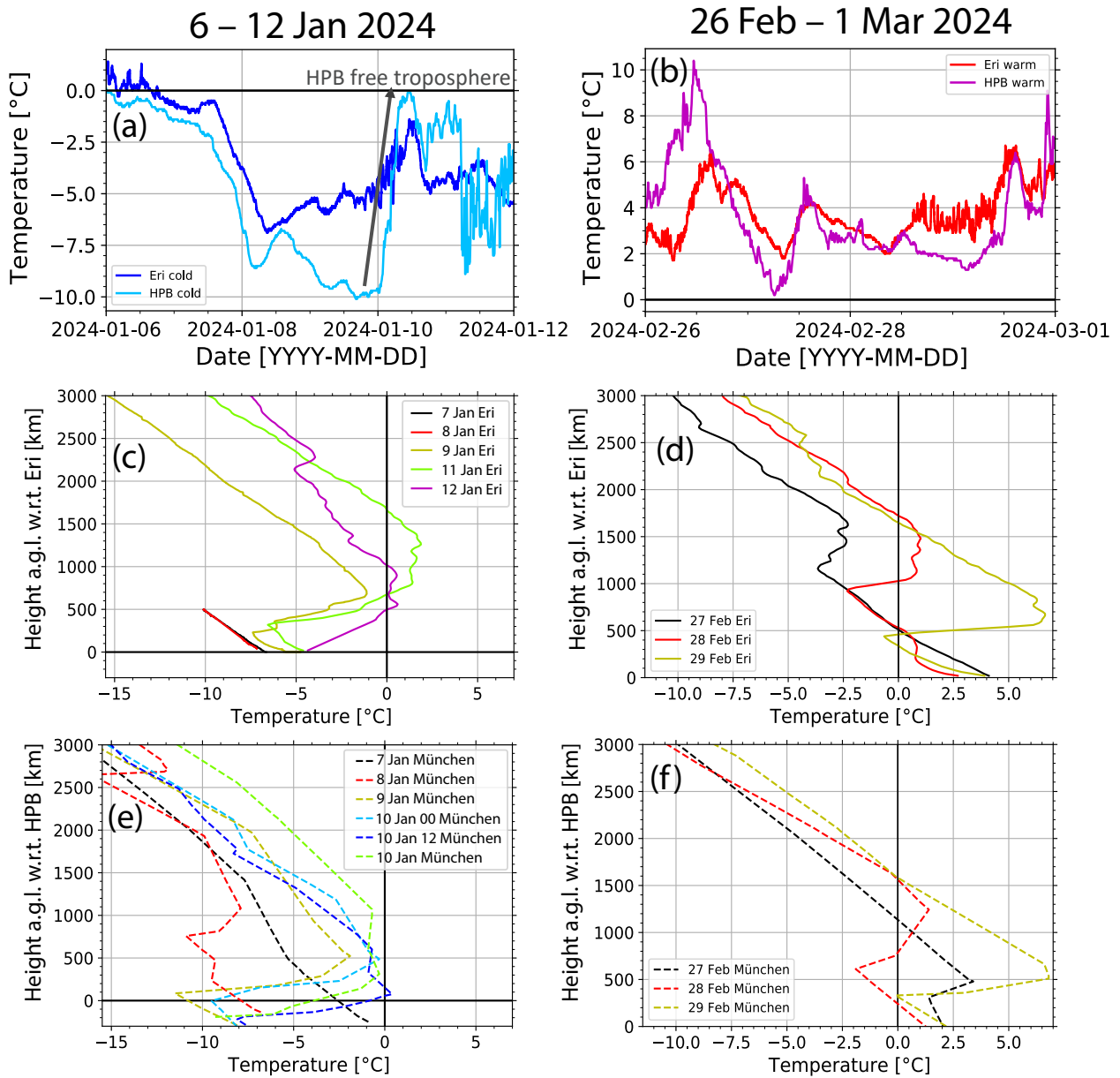
Figure 2. Temperature evolution during both measurement periods. a) Surface temperature during cold period (6–12 January 2024). The transition time when the inversion has lowered and HPB is no longer in the boundary layer but in the free troposphere is indicated with a gray arrow. b) Surface temperature evolution for the warm period (26 Feb 2024 to 1 Mar 2024). c) Temperature profiles for the cold period in Eri. d) Temperature profiles for the warm period in Eri. e) and f) Temperature profiles for HPB for the cold and warm periods, respectively, represented by München-Oberschleißheim data (CDC, 2024). Eri surface data are observed by LACROS instrumentation at the field site in Eri. HPB profile data are from University of Wyoming (2024). Eri profile data are from radiosonde launches at Eri. Note that a.g.l. relates to the height of 921 m for Eri and 977 m for HPB.
