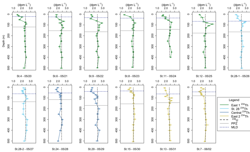
431 432 Figure 4. Profiles of total 234 Th and 238 U in the upper 500 m of the water column in East 1 stations (green), Station 28 433 (light blue), central stations (dark blue) and East 2 stations (yellow). The base of the primary production zone (PPZ) is 434 shown with a grey solid line and the base of the mixed layer (MLD) is shown with a blue dashed line.
