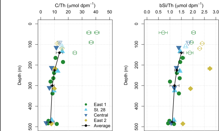
Figure 5. Profiles of POC/ 234 Th (C/Th) and bSi/ 234 Th (bSi/Th) ratios in >51 \mu\text{m} particles across regions. Black symbols denote average C/Th ratios (all stations) and average bSi/Th ratios (all stations except East 2) for the following depth horizons: 115–185, 210–240, 260–340, 465–490 m. Empty symbols denote samples collected within the primary production zone. Analytical uncertainties are represented by horizontal bars and uncertainties less than \sim 3 \mu\text{mol dpm}^{-1} are not visible against filled symbols. POC = particulate organic carbon, bSi = biogenic silica.
