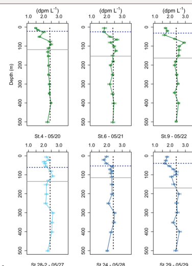
Deleted: Figure 4. Profiles of total 234 Th and 238 U in the upper 500 m of the water column in East 1 stations (green), Station 28 (light blue), central stations (dark blue) and East 2 stations (yellow). The base of the primary production zone (PPZ) is shown with a grey solid line and the base of the mixed layer (MLD) is shown with a blue dashed line.
