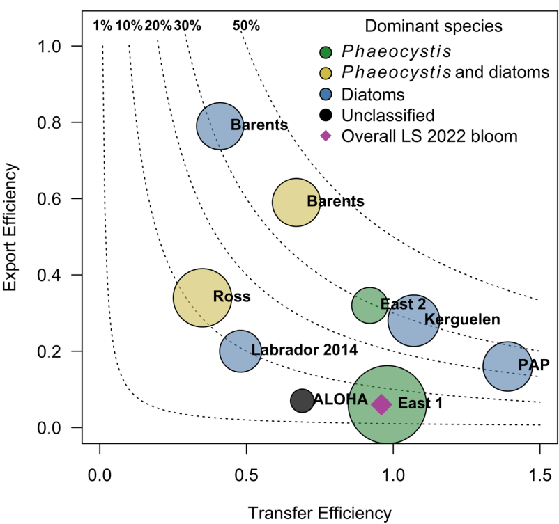
795 796 Figure 8. Biological carbon pump efficiency (BCP) comparing bloom studies across different regions (see Table 2). The 797 x-axis depicts transfer efficiency (flux at 100 m below PPZ base/flux at PPZ base) and the y-axis export efficiency (flux 798 at PPZ base/integrated NPP within PPZ). Contour lines represent overall BCP efficiency (percentages), and symbol 799 area is proportional to NPP. The "East 1" and "East 2" symbols and the diamond correspond to this study. The 800 diamond represents the overall BCP efficiency for the Labrador Sea (LS) 2022 bloom, calculated using satellite-derived 801 NPP integrated from the bloom peak to the final day of sampling. Studies are colour-coded according to the dominant 802 phytoplankton species. The ALOHA site (Buesseler and Boyd, 2009) is also shown as a low-end member. PPZ = primary 803 production zone, NPP = net primary production.
