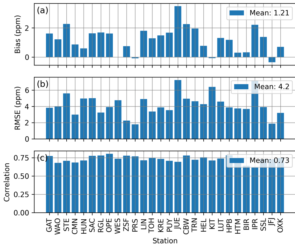
Figure S2. Annual statistics of mean modeled versus observed afternoon CO 2 mole fractions at ICOS stations in the European model domain. Panel (a) shows monthly mean biases for each site inside the model domain, (b) RMSEs, and (c) correlation coefficients.
