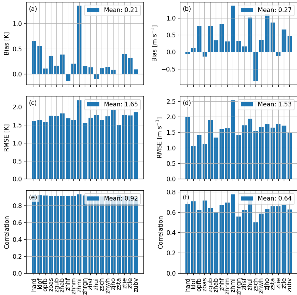
Figure S7. Annual statistics of mean modeled versus observed afternoon wind speed and temperature values in Zurich. Panels (a), (c), (e) show annual mean temperature Bias, RMSE, and correlation, correspondingly, while panels (b), (d), (f) show similar statistics for the wind speed.
