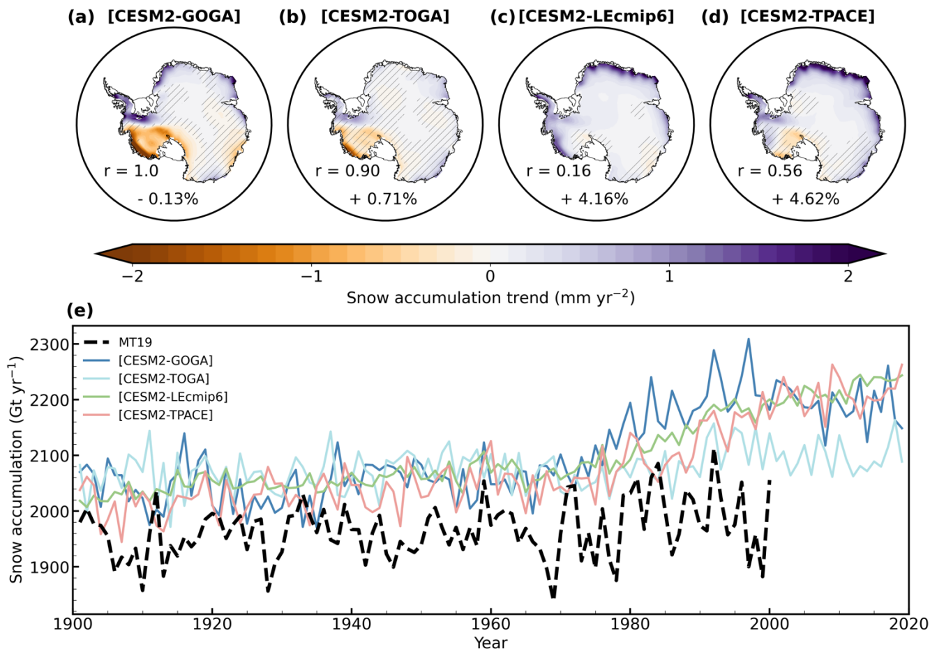
Figure 6. Maps of 1979-2019 linear trends in snow accumulation for a) [CESM2-GOGA], b) [CESM2-TOGA], c) [CESM2-LEcmip6], and d) [CESM2-TPACE]. The percentages indicate changes of the Antarctic-wide snow accumulation rate averaged over 2005-2019 compared with 1979-1993. The r values represent the pattern correlation of the simulated trend with the trend given by [CESM2-GOGA]. Hatching indicates where the accumulation trend is not significant at the p < 0.05 level or better. e) Timeseries of annual snow accumulation over the grounded AIS from MT19 and various model simulations.
