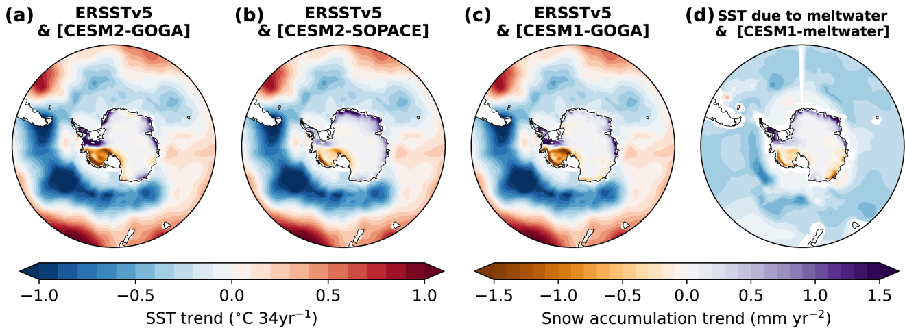
125 Figure B6. As in Fig. 8 but including results from the CESM Southern Ocean Pacemaker experiment that was nudged to SST anomalies from ERSSTv5 over the Southern Ocean (Kang et al., 2023). Data from CESM2 Southern Ocean Pacemaker provided by Yue Yu and Sarah Kang.
