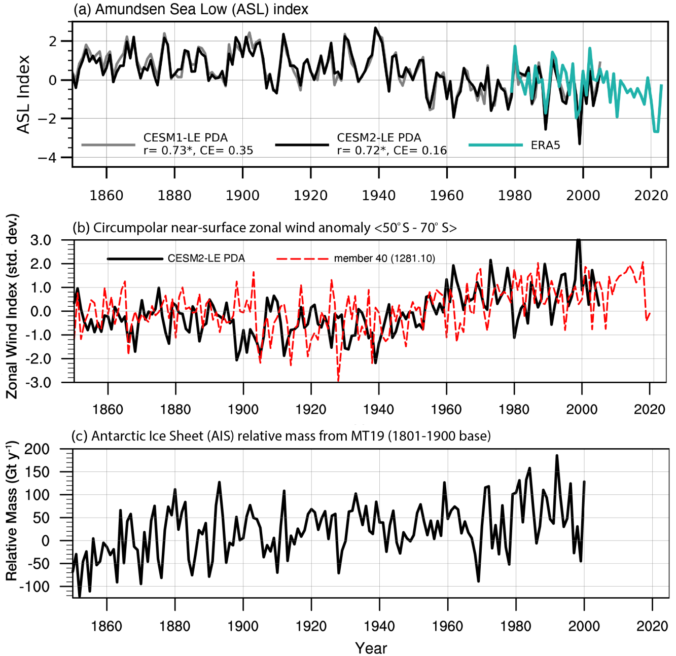
320 Figure 1. a) Timeseries of annual-mean Amundsen Sea Low (ASL) index from two different instances of PDA, compared with ERA5. Anomalies relative to 1979-2005. The ASL Index is the standardized mean SLP over 60^\circ\text{-}75^\circ\text{S} , 180^\circ\text{-}310^\circ\text{E} ; b) 325 Standardized, annual mean, near-surface zonal wind indices across 50^\circ\text{-}70^\circ\text{S} from CESM2-LE PDA and member 40 of CESM2- LEcnp6 (using 10 m zonal wind). The 1901-2000 linear trend in the CESM2-LE PDA zonal wind index is statistically significant ( p < 0.01 ); c) Relative mass timeseries integrated over the grounded AIS from MT19 snow accumulation reconstruction. Base period is 1801-1900. The 1901-2000 linear trend in relative mass is statistically significant ( p < 0.05 ). Over 1901-2000, detrended relative mass and the detrended zonal wind index from CESM2-LE PDA are significantly correlated ( r = -0.39 , p < 0.01 ).
