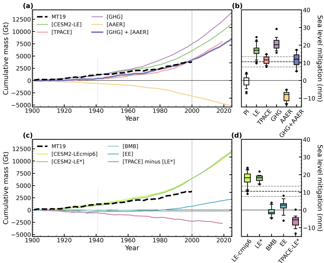
370 Figure 2. Cumulative mass and equivalent sea level mitigation due to accumulated snow on the grounded Antarctic Ice Sheet (AIS) 375 in MT19 and CESM2: (a) Cumulative mass timeseries from MT19 compared with timeseries from selected ensemble means; (b) Box plot indicating ensemble spread of cumulative mass at the year 2000 for each of the ensembles and the pseudo ensemble generated by summing 15 individual members of GHG and AAER. The boxes indicate the interquartile range; the median is shown by a horizontal line. Whiskers represent the 5% and 95% bounds of the ensemble, with the values lying outside of these bounds indicated by closed black circles. “PI” refers to the piControl simulation: mass was accumulated over 24 overlapping, 100- year segments. Dashed black horizontal line indicates the mean value of MT19; gray dashed lines indicate its \pm 1 \sigma uncertainty
