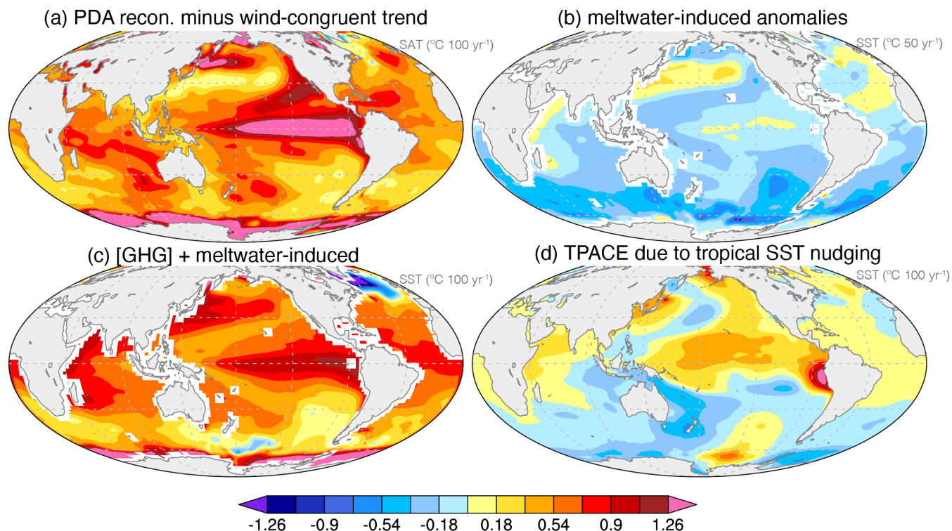
730 Figure 9. a) Map of 1901-2000 trend in CESM1-LE PDA SAT after removal of the wind-congruent trends (as in Fig. 5f); b) SST 735 anomalies due to historical Antarctic meltwater anomalies from the CESM1-AIS meltwater experiment (decadal trend multiplied by five to estimate meltwater's role over the second half of the 20th Century); c) SST anomalies formed from [GHG] (as in Fig. 5l) added to the meltwater-induced anomalies in panel b. d) 1901-2000 trend in TPACE due to tropical SST nudging. To ensure that the anomalies in d) are not aliasing interannual ENSO variability, an 8-y lowpass filter was applied to annual timeseries in [TPACE]-[CESM2-LE*] before computing the trend. Radiative surface temperature is used for [GHG]. Note that the SAT pattern in a) likely contains an aerosol signature, especially in the north Pacific and north Atlantic.
