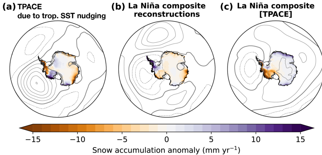
115 Figure B5. (a) Tropically driven ([TPACE] - [CESM2-LE*]) trend patterns in SLP and snow accumulation (1976:2000 minus 1901:1925). (b, c) Composites of snow accumulation and SLP anomalies during La Niña years over 1901-2000. Accumulation and SLP timeseries were linearly detrended before forming the composites. La Niña years are defined from NOAA's extended multivariate ENSO index, using austral autumn (MAM) values ( https://psl.noaa.gov/enso/mei.ext/ ). The years composited are 1902, 1904, 1907, 1908, 1909, 1910, 1911, 1913, 1916, 1917, 1921, 1950, 1955, 1956, 1963, 1971, 1974, 1975, 1976, 1982, 1985, 1989, 1991, 1999, and 2000. SLP contours (gray lines) are in intervals of 0.25 hPa. Negative SLP values are dotted lines and positive values are solid lines; the zero contour is a heavier solid line. 120
