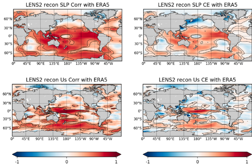
Figure A1. Verification statistics for the CESM2-LE PDA reconstruction SLP (top row) and U10 (bottom row), compared to ERA5 reanalysis for the period of overlap, 1979 to 2005 (anomaly reference period used in this analysis is 1979 to 2005). Correlations are shown on the left, with contours highlighting p-values of 0.01 and 0.05. Coefficient of efficiency (CE) is shown on the right ( > 0 demonstrates skill). See further verification and discussion in O'Connor et al. (2025). From https://jortuck.github.io/PaleoclimateVisualizer/ , the 50°-70° S near-surface zonal wind index that we use from CESM2-LE PDA is
