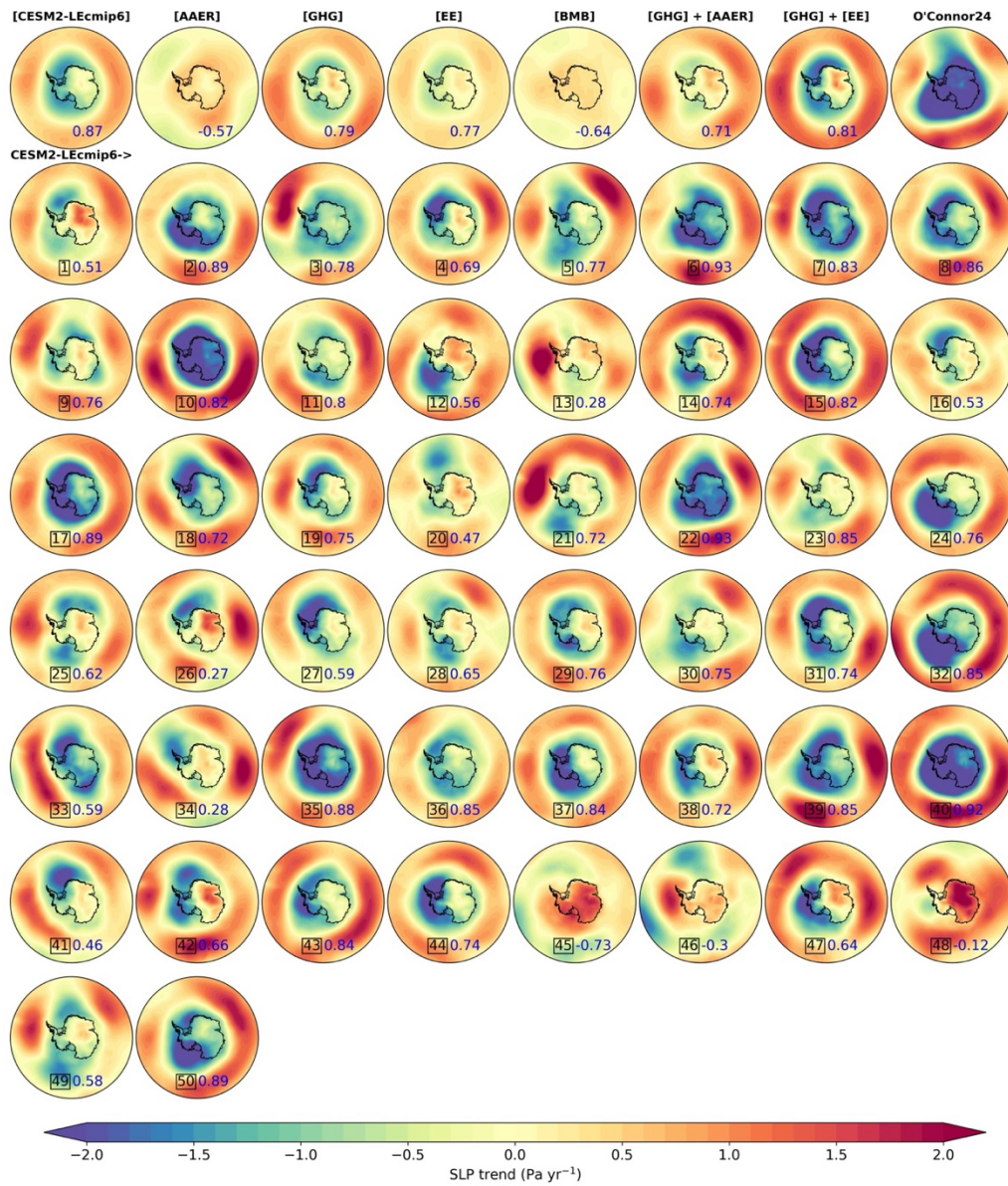
110 Figure B4. As in Fig. B3, but for SLP and using the CESM2-LE PDA reconstruction (labeled O'Connor24) as the benchmark for the pattern correlation over 40°-90° S.
