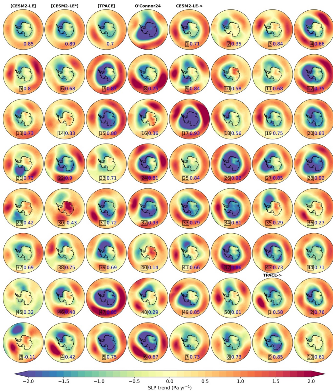
100 Figure B2: As in Fig. B1, but for SLP and using the CESM2-LE PDA reconstruction (labeled O'Connor24) as the benchmark for the pattern correlation over 40°-90°S, a domain that covers the footprint of the ASL and most of the footprint of the SAM (e.g. Marshall, 2003).
