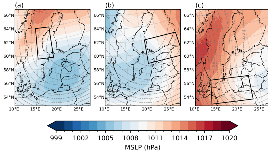
Figure 10. As in Figure ?? Composite mean 500 hPa-level geopotential height (gpm, but for the number of days contours) and mean sea level pressure (hPa, color shading) associated with snowfall exceeding 5 on snowband days in the three subregions shown in Figs. 1 and 9. Snowband day in each subregion is defined here as a day during which all the refined snowband criteria (see Table 1) were fulfilled, and the 900 hPa-level wind direction was (a) 350–360° or 0–140°, (b) 90–255° and (c) 280–360° or 0–80°, in at least one grid box at least once somewhere in the subregion.
