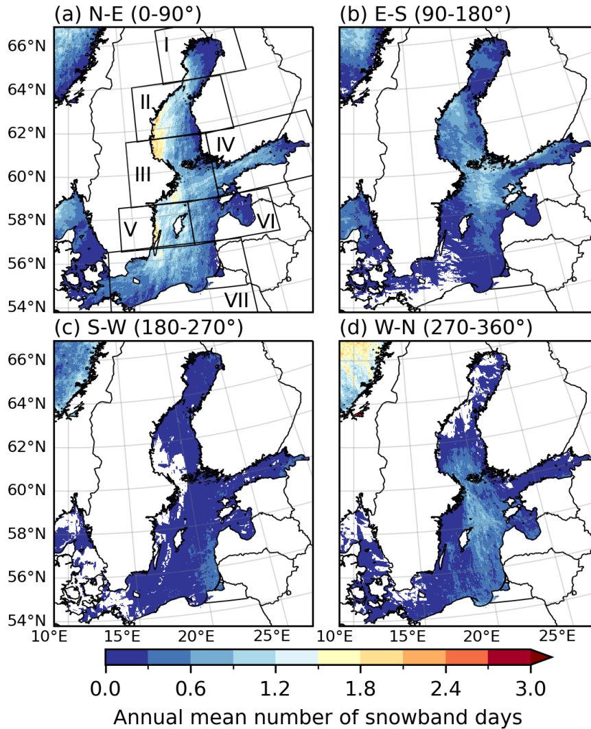
Figure 6. As in Figure ?? Fig. 5 , but with an additional criterion for the 900 hPa-level wind direction between (a) 0–90°, (b) 90–180°, (c) 180–270° and (d) 270–360°. The subregions presented in Table 3 and Figure ?? Fig. 8 are marked in (a).
