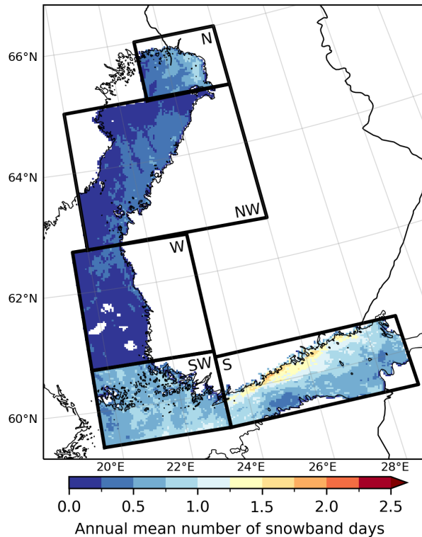
Figure 3. Annual mean number of snowband days in 1998–2018 in HCLIM detected by using the criteria close to those used by ? , or OLS2022, criteria given in Table 1 of Olsson et al. (2023, or OLS2023, criteria given in Table 1) . Snowband day in each grid box is defined here as a day during which all the criteria were fulfilled at least once.
