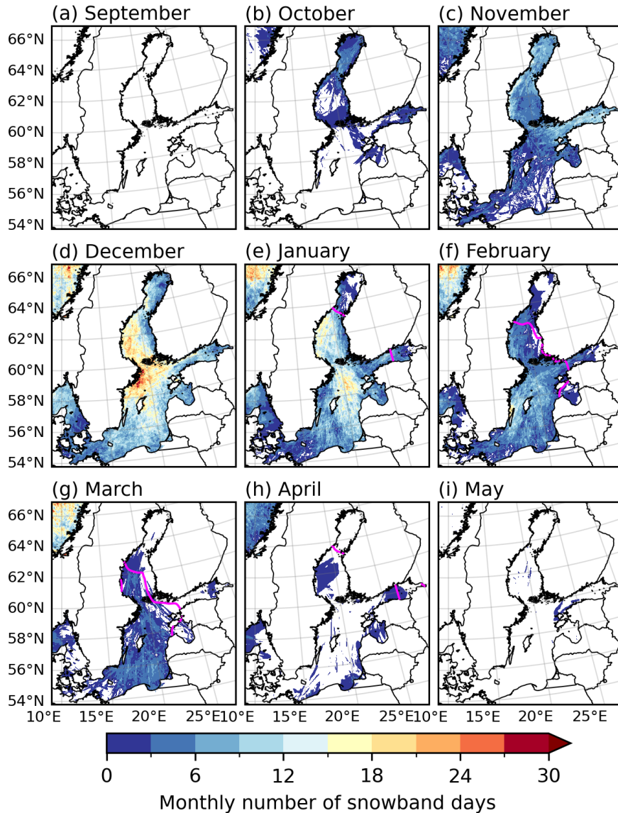
Figure 7. As in Figure 5 , but for the total monthly number of snowband days. Purple line indicates the mean sea ice extent in HCLIM.
