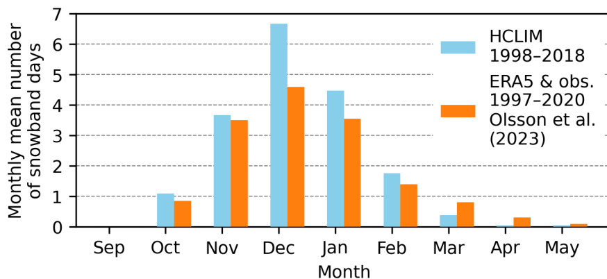
Figure 2. Monthly mean number of snowband days in Finland (FI, see subregion in Fig. ??1) in HCLIM in 1998–2018 (blue) and that estimated from Figure Fig. 2 of ?, or OLS2022, licensed under CC BY 4.0 Olsson et al. (2023, or OLS2023, licensed under CC BY 4.0) using ERA5 reanalysis data and snow depth observations in 1997–2020 (orange). The snowband days are detected from HCLIM using the criteria close to those of OLS2022 OLS2023 (see Table 1). Snowband day is defined here as a day during which all the criteria were fulfilled in at least one grid box at least once a day somewhere in FI.
