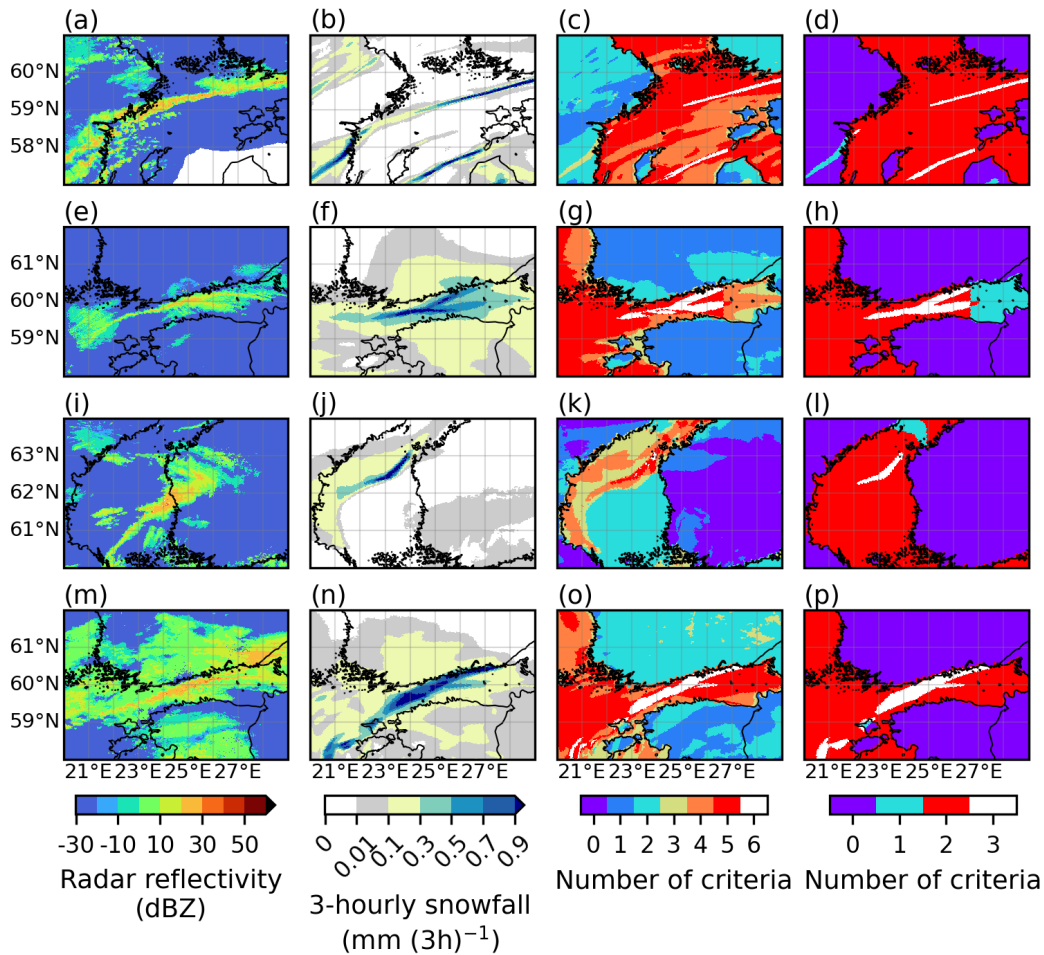
Figure 4. Observed radar reflectivity (dBz, first column), 3-hourly snowfall ( \text{mm (3h)}^{-1} , left panel), from HCLIM (second column) and the number of refined (middle third column) and loose (right fourth column) criteria fulfilled at each grid box in HCLIM on (in the four case studies). Note that for a (e) certain case study, the time and date in the first column may differ from that of the other columns. Namely, data is shown on 13 November 2007 at 15 UTC, in (da)–(fd), on 2 February 2012 at 23 UTC in (e) and at 15 UTC, in (gf)–(h), on 8 January 2016 at 11 UTC in (i) and on 9 January 2016 at 0 UTC and in (j)–(l), and on 8 November 2016 at 18 UTC (m) and 15 UTC in (n)–(p)
