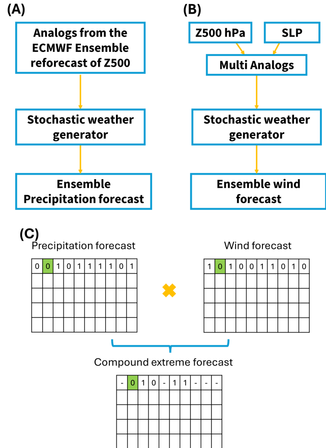
Figure 1. Illustration of the forecast process. (a) The HC-SWG used to forecast extreme precipitation; (b) the MA-SWG used to forecast wind speed, and (c) the ensemble forecast of the co-occurrence of precipitation and wind speed extremes.
