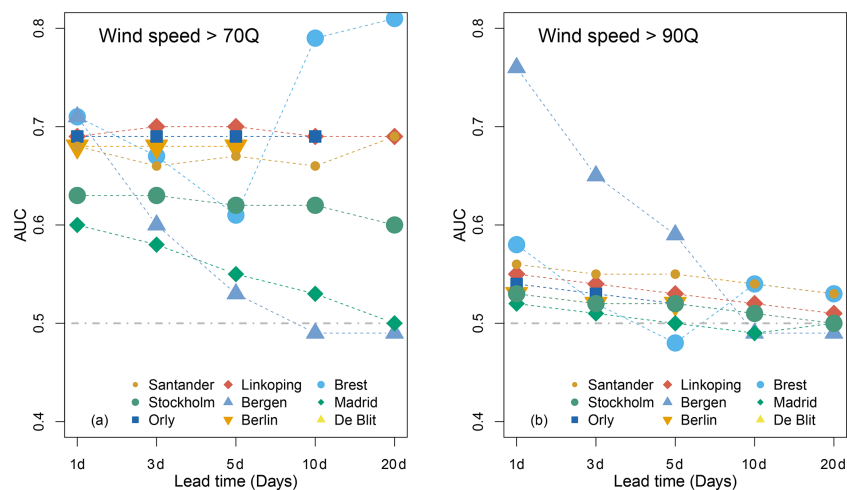
Figure E3. AUC for the MA-SWG wind speed forecasts for (a) wind speed events exceeding the 70 th Q threshold, and (b) wind speed events exceeding the 90 th Q threshold. The dashed grey lines represent AUC = 0.5 .
