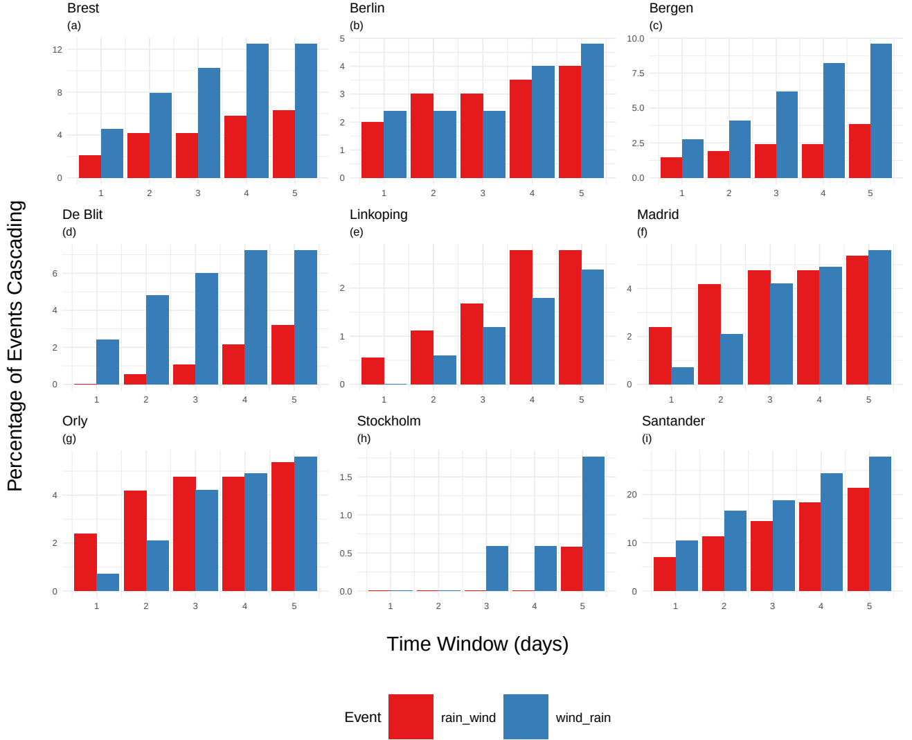
Figure 12. Percentage of extreme precipitation or wind events which are followed by the other extreme, as forecasted by the SWG at lead time T = 10 days. Red represents events where extreme precipitation is followed by extreme wind, and blue represents events where extreme wind is followed by extreme precipitation. We consider time windows (lags between the two extreme weather events) from 1 to 5 days. The y-ranges differ between panels.
