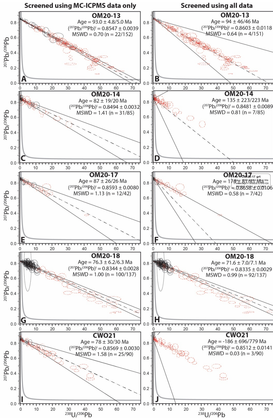
Figure 11: Tera-Wasserburg diagrams of garnet U-Pb LASS-ICPMS analyses for OM20-13 (a, b), OM20-14 (c, d), OM20-17 (e, f), OM20-18 (g, h), and CWO21 (i, j). Only analyses with Zr contents at or below the average Zr background content are plotted in (f). Data points are color-coded in grayscale for Zr content between white (lowest
