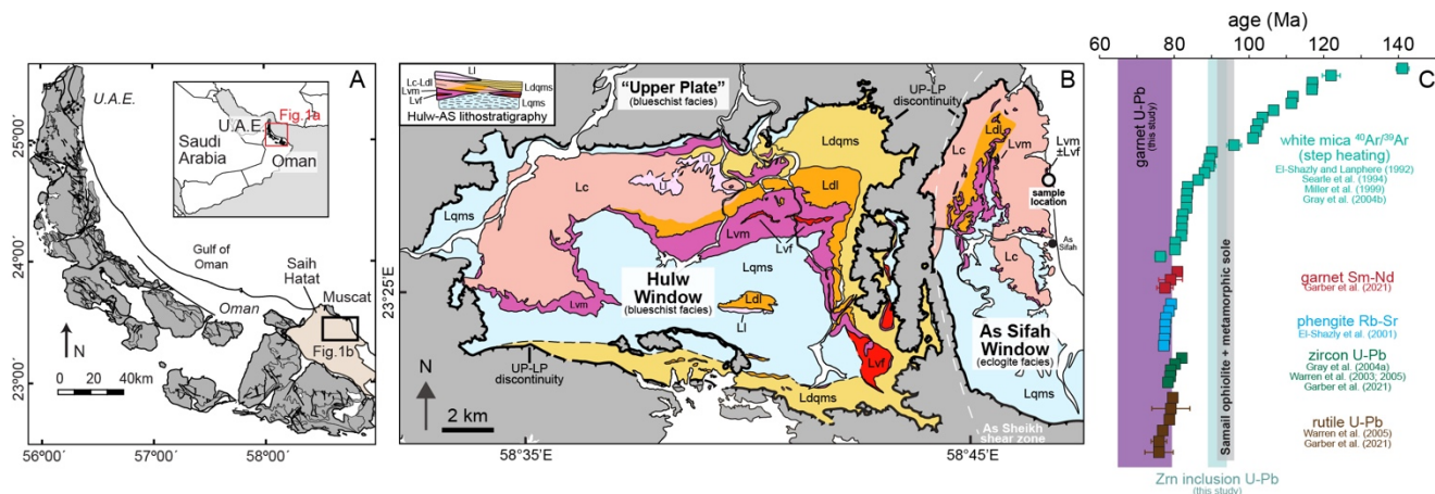
135 Figure 1: (a) Regional overview map modified from Nicolas et al. (2000) showing the Samail ophiolite (dark gray) and subducted continental margin rocks of the Saih Hatat (light brown). (b) Lithologic map of the Hulw and As Sifah windows in the Saih Hatat, modified from Miller et al. (2002), Searle et al. (2004), and Warren and Miller (2007) (and lightly modified from Garber et al., 2021). The dominant structural feature is the “UP-LP” discontinuity (bold line), which separates “Upper Plate” rocks (dark gray) from “Lower Plate” units. The poorly-exposed but structurally necessary “As Sheikh” ductile shear zone between the Hulw and As Sifah Windows is shown in a dashed white line. Unit abbreviations: Lqms = lower-plate quartz-mica schist; Lvf = lower-plate felsic volcanic; Lvm = lower-plate mafic volcanic; Lc = lower-plate calcschist and quartz schist; Ldl = brown dolomite; Ldqml = dolomitic quartz-mica schist; LI = Permian metacarbonate. The mafic eclogite samples in this study are interpreted to be part of the “Lvm” and “Lvf” units exposed just north of the town of As Sifah. The inset stratigraphic sketch is modified from Miller et al. (2002); the Hulw and As Sifah Windows are interpreted as stratigraphically correlative equivalents of the Ordovician (Lqms; Amdeh Fm.) to Permian (Lc-LI; Saiq Fm.) Arabian continental margin sequence that is also exposed in the “Upper Plate” (e.g., Searle et al., 2004; Warren and Miller, 2007; Chauvet et al., 2009). (c) Previously published geochronology from the As Sifah eclogites, including the new U-Pb dates in this study. Ar/Ar hornblende and U-Pb zircon geochronology from the overlying Samail ophiolite and metamorphic sole is shown as a gray bar (dates from Hacker et al., 1996; Warren et al., 2005; Styles et al., 2006; Rioux et al., 2012; 2013; 2016; 2021; 2023). Where not visible, error bars on dates are smaller than symbols. See text for additional discussion.
