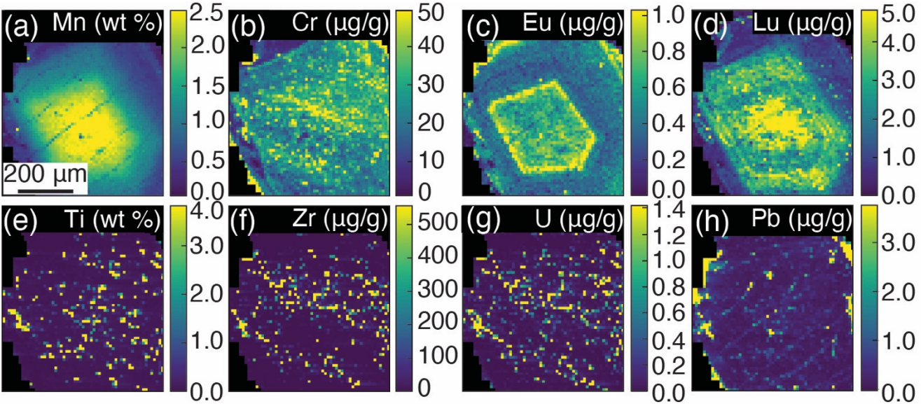
Figure 3: LA-ICPMS minor- and trace-element maps of Mn (a), Cr (b), Eu (c), Lu (d), Ti (e), Zr (f), U (g), and Pb (h) in a garnet grain in sample CWO21. Each pixel is 20 x 20 μm 2 . High Pb regions at the edge of the garnet are the result of contamination by matrix phases, such as epidote, chlorite, and white mica.
