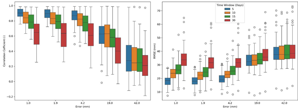
Figure S2 Daily Boxplots of correlation coefficient (CC), root mean square error (RMSE) of 100 grid points randomly selected over Europe at four time windows (5, 10, 15 and 30) with an error of 1.9 mm, 4.2 mm, 19 mm and 42 mm for estimating 30-day precipitation for the period 2003-2012.
