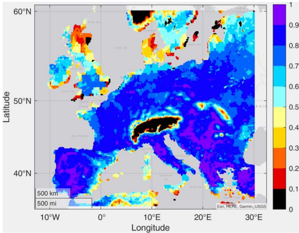
Figure S1 Correlation between ERA5L based TWS and GRACE based TWS
