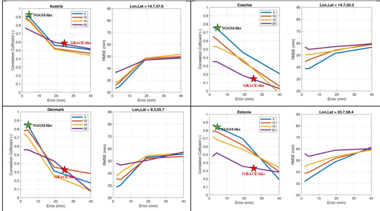
Figure 5: Evaluation of the NGGM/MAGIC synthetic experiments at four temporal resolutions (5, 10, 15 and 30) with error levels ranging from 0 mm to 40 mm for estimating 30-day precipitation over random locations in Italy, Germany, Spain, Greece, Austria, Czechia, Denmark, Estonia for the period 2003-2012 in terms of correlation coefficient (R) and root mean square error (RMSE).
