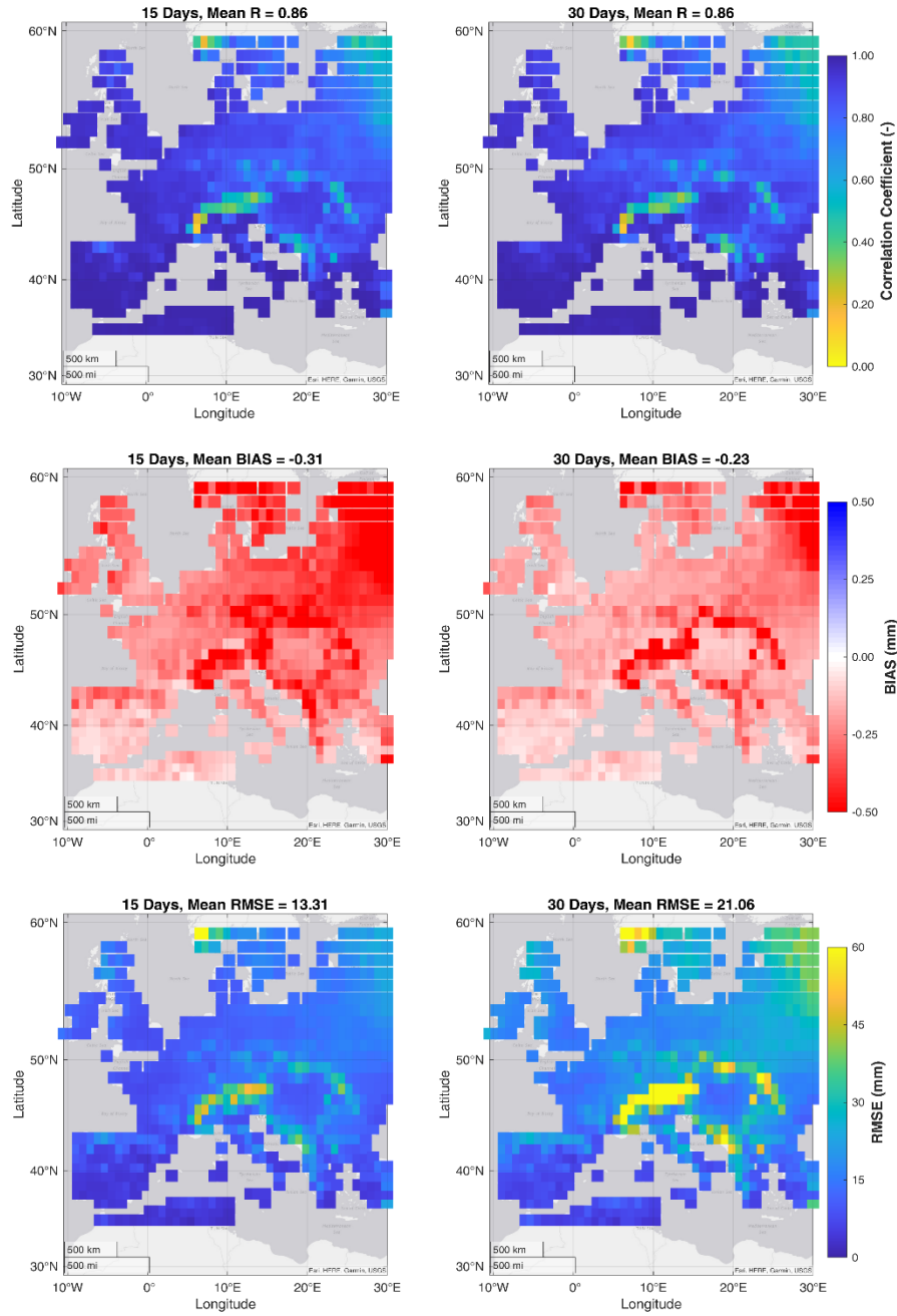
Figure 2: Performances of SM2RAIN algorithm forced with ERA5L based TWS proxy against the ERA5L precipitation data over Europe for the period 2003–2012. The two columns refer to 15-day and 30-day aggregation period., rows indicate the correlation coefficient, R (top panel), bias (middle panel) and root mean square error, RMSE (lower panel).
