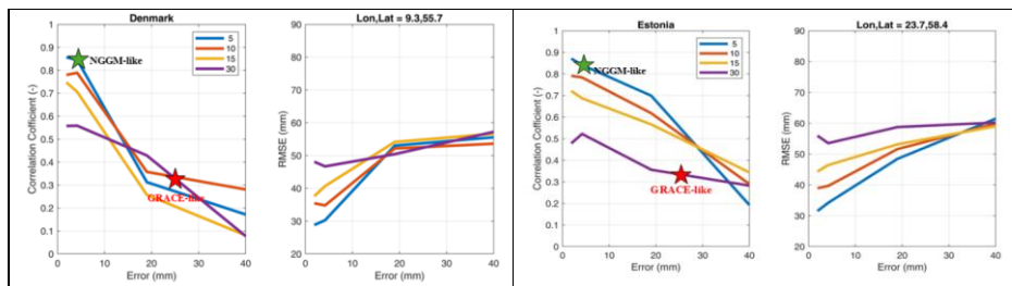
Figure 5: Evaluation of the NGGM/MAGIC synthetic experiments at four temporal resolutions (5, 10, 15 and 30) with error levels ranging from 0 mm to 40 mm for estimating 30-day precipitation over random locations in Italy, Germany, Spain, Greece, Austria, Czechia, Denmark, Estonia for the period 2003-2012 in terms of correlation coefficient (R) and root mean square error (RMSE).
