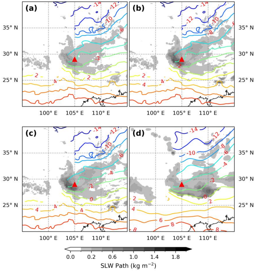
Figure 3 Spatial distribution of SLW path (shaded, unit: \text{kg m}^{-2} ) and 700 hPa temperature fields (colour lines, unit: ^{\circ}\text{C} ) for (a) Default, (b) Climatology, (c) CAMS, and (d) ERA5 reanalysis. Red triangles denote the observed icing locations.
