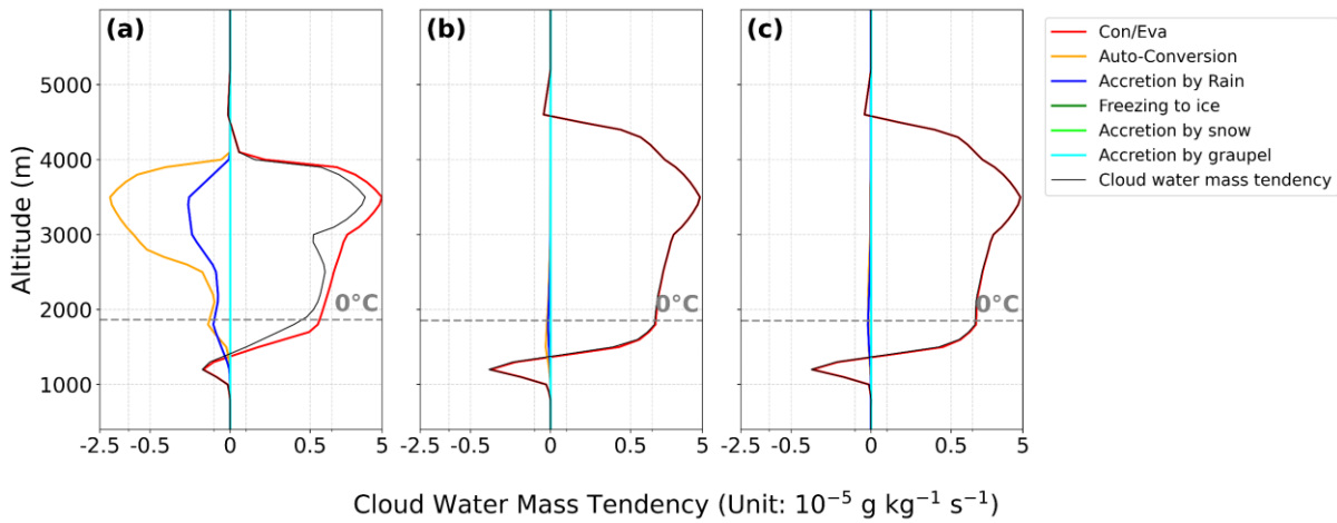
Figure 5 Time-domain-average vertical profiles of cloud water mass tendency for Default (left), Climatology (middle) and CAMS (right) from 12:00 to 14:00 UTC.
