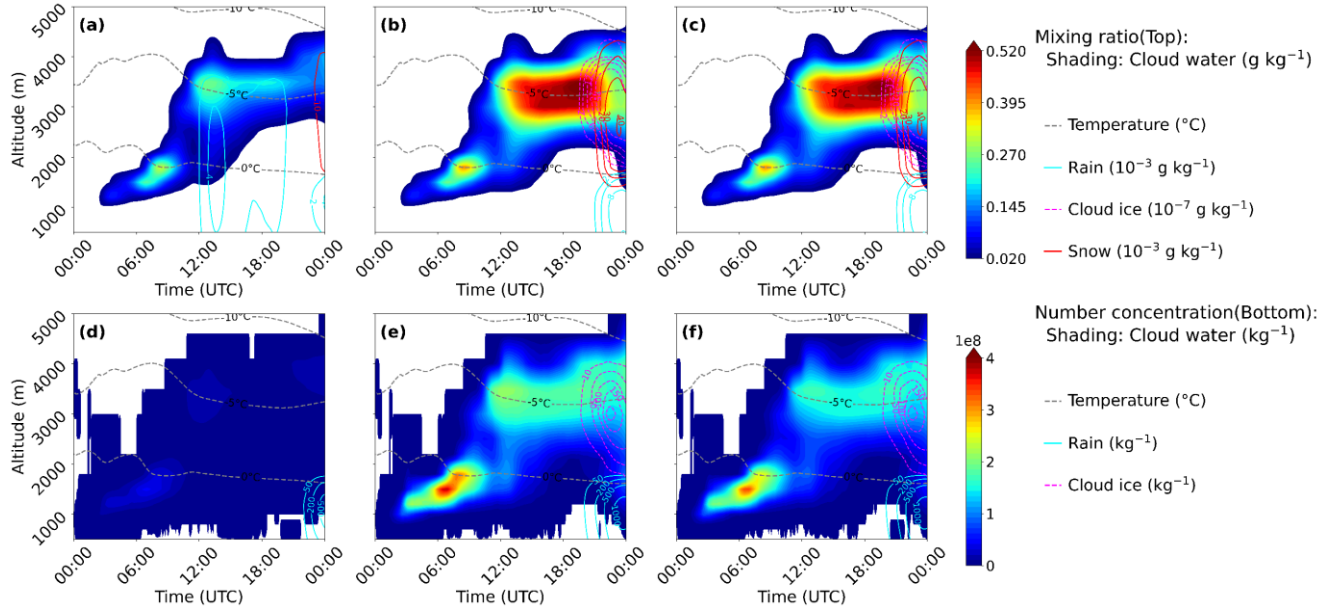
Figure 4 Domain-average time-altitude cross section of hydrometeor mass mixing ratio (top) and number concentration (bottom) averaged over the in-flight icing region (orange path in Fig. 1b) for the three experiments: Default (left), Climatology (middle) and CAMS (right).
