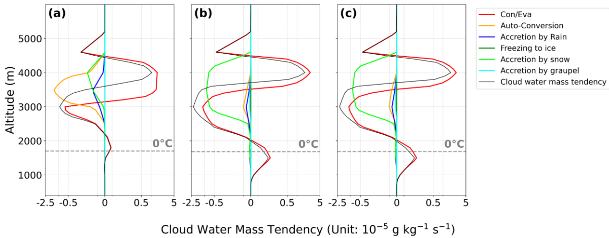
Figure 6 Same as Fig.5 but for 21:00 to 24:00 UTC.
