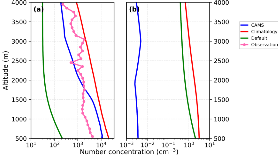
235 Figure 2 Vertical profiles of initial CCN (left) and IN (right) number concentrations for Default (green), Climatology (red), CAMS (blue) experiments, along with the aerosol number concentration from PCASP (pink).
