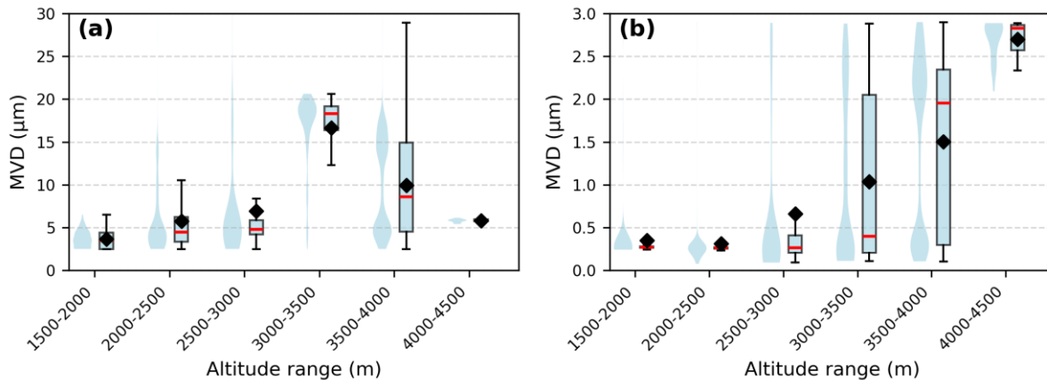
390 Figure 9 Altitude-resolved violin and box plots of MVD for cloud droplets (left) and aerosols (right), in 500 m bins, derived from CDP and PCASP data (The diamonds indicate the mean values, and the red lines denote the medians).
