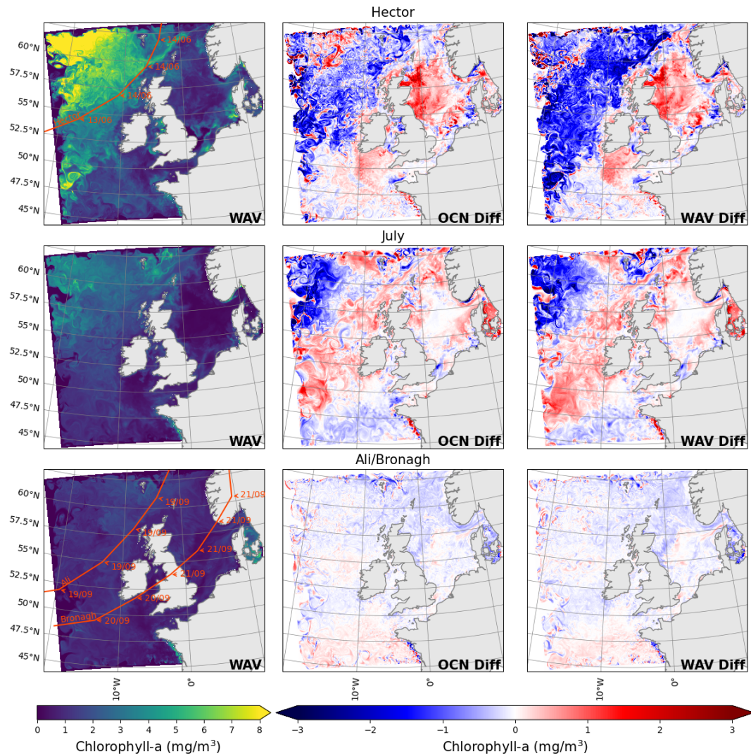
Figure 14. Mean chlorophyll in the five days before the storm from the ocean-biogeochestry model (left), the difference between the mean of the five days after the storm and the mean of the five days before the storm from the ocean-biogeochestry model (middle) and the ocean-wave-biogeochestry model (right), for storm Hector (top), July storm (middle) and storms Ali and Bronagh (bottom). The start of the five days before and the end of the five days after the storms are highlighted in Figure 3 as vertical bars.
