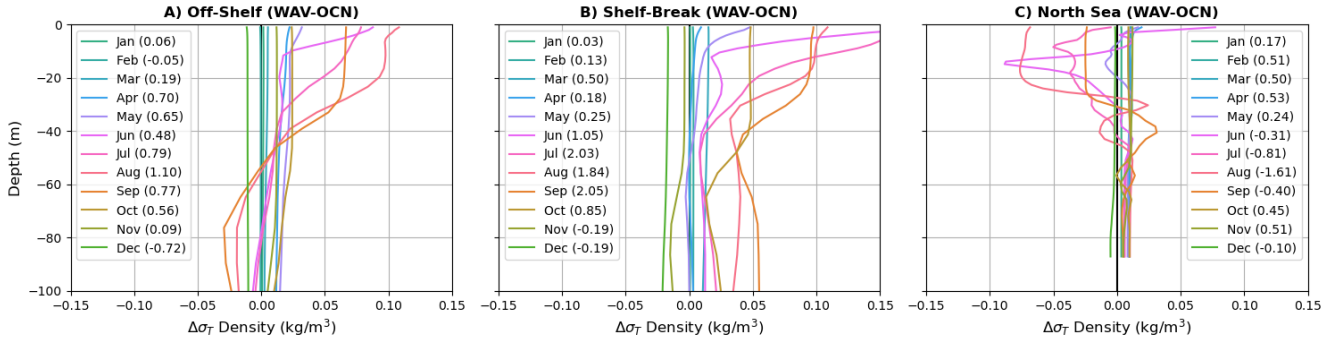
Figure 13. Difference in density ( \text{kg/m}^3 ) stratification profiles in the upper 100m throughout the year for the three regions. Density given in \sigma_T (= \sigma - 1000) coordinates, with the total difference throughout the column for each month shown in parenthesis.
