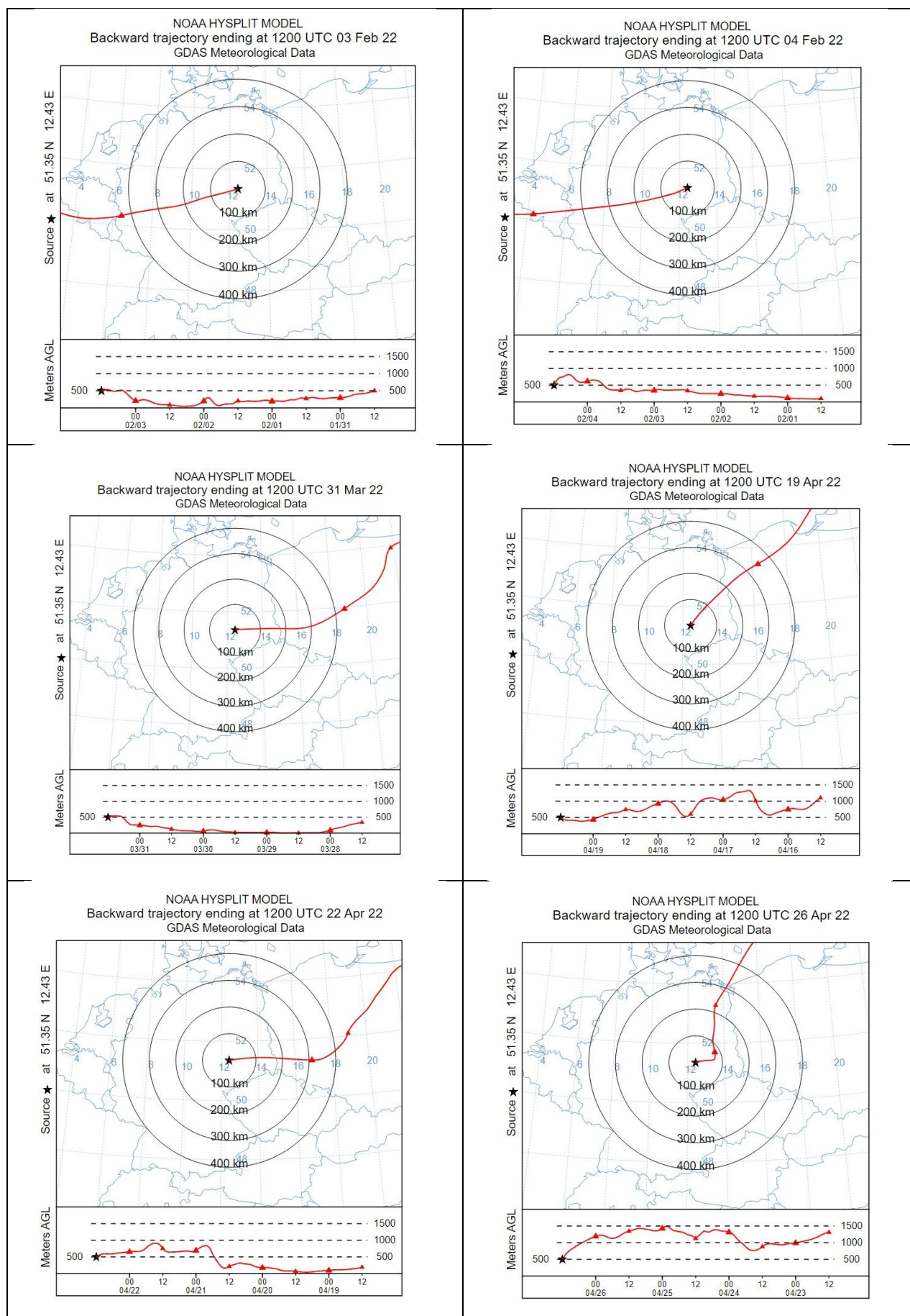
Figure S1: Graphical output files created by the HYSPLIT model for February 3, February 4, March 31, April 19, April 22, and April 26, 2022
