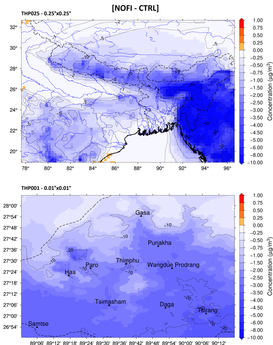
Figure 11. Impact of fires on \text{PM}_{2.5} concentrations for the THP025 and THP001 domains (respectively top and bottom). Average concentration decrease without fire emissions over all domains (NOFI - CTRL) from the 17 to 31 March. The contour lines are the reduction in % (from the CTRL reference case concentration)
