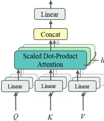
225 Figure 3. Multi-Head Attention consists of h parallel attention heads, each operating on a distinct learned projection of the input. Q , K , and V are all derived from the BiLSTM output.
