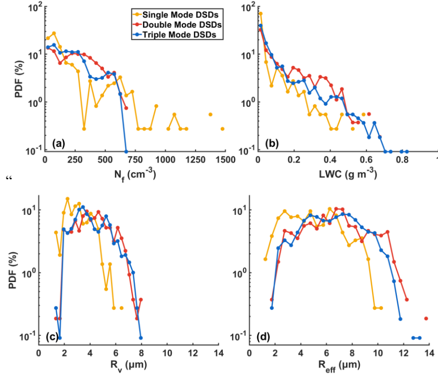
Figure 9 PDF distributions of N_f (a), LWC (b), R_v (c) and R_{eff} (d) for DSDs with different modes”
