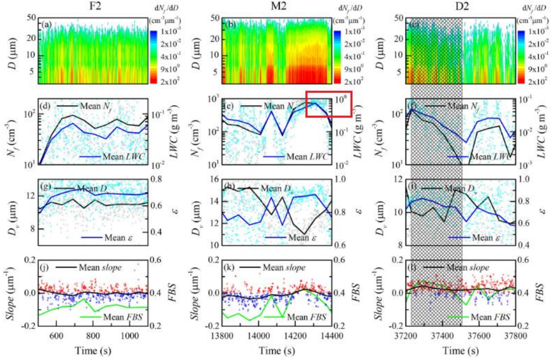
Figure 7. Same with Figure 5 but for the fourth fog case.
