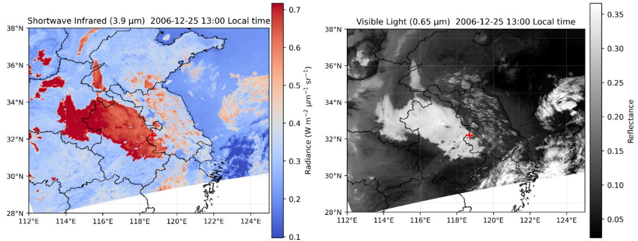
Figure A2 Aqua MODIS 3.9 \mu m shortwave infrared and visible channel imagery for Fog 1-1, with the observation site marked by a red cross.
