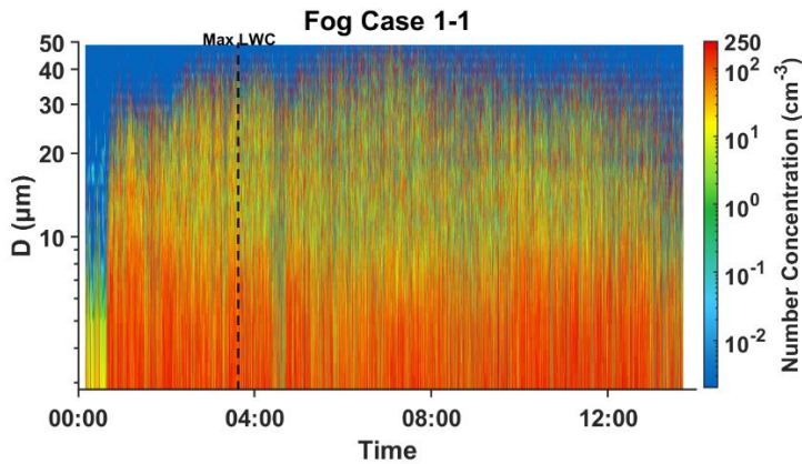
Figure A11 The time series of DSDs at 1s resolution of Fog Case 22, Fog Case 4, Fog Case 1-1, Fog Case 10 and Fog Case 20”
