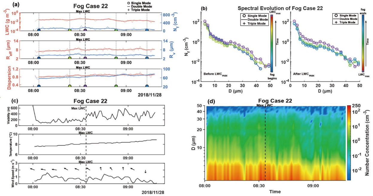
Figure 4 (a) is the temporal evolution of N_f , LWC, R_{\text{eff}} , FBS and dispersion for fog case 22, the dark lines represent 5-minute averaged values while the light lines are 1-minute averaged values. (b) is the 5-minute average DSD. As LWC reaches its maximum, the colors vary from blue to red, and each DSD in (b) are marked by colored dots in (a) with each color corresponding to a specific DSD and its number of peaks indicated. (c) is the temporal evolution of visibility, temperature and wind speed, with wind direction represented by wind barbs. (d) is the 1-minute temporal evolution of DSDs.
