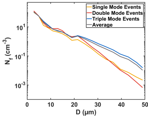
Figure 3 Average spectra of fog events with different modes
