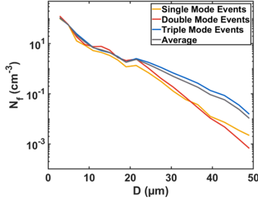
Figure 3 Average spectrums of fog events with different modes
