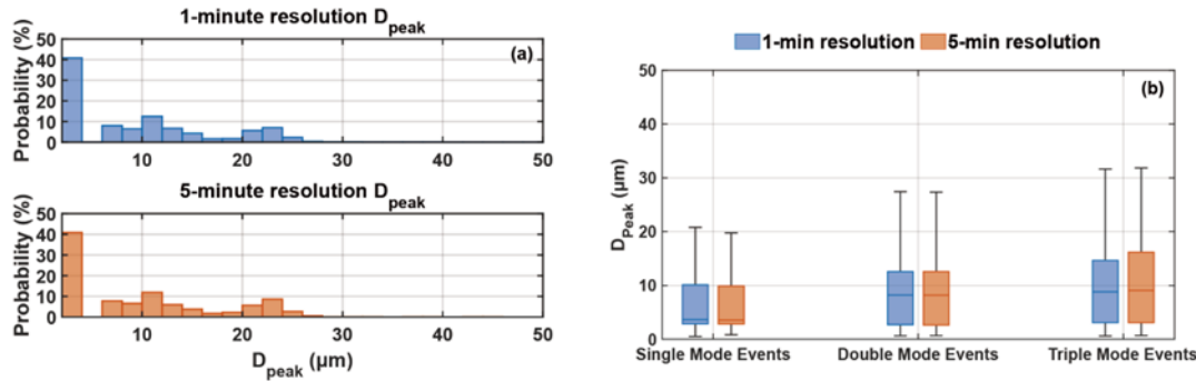
Figure 2 (a) The D_{\text{peak}} distributions of all DSDs at 1-min and 5-min resolution, and (b) the D_{\text{peak}} distributions by fog type at both resolutions
